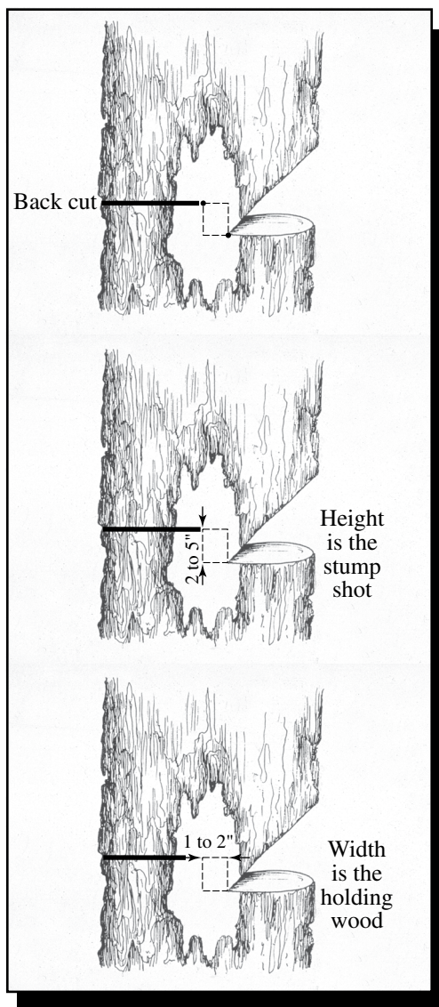
Figure 60—An imaginary rectangle can help the sawyer understand the importance of the back cut. The dimensions of this rectangle are based on a 24-inch diameter tree.
