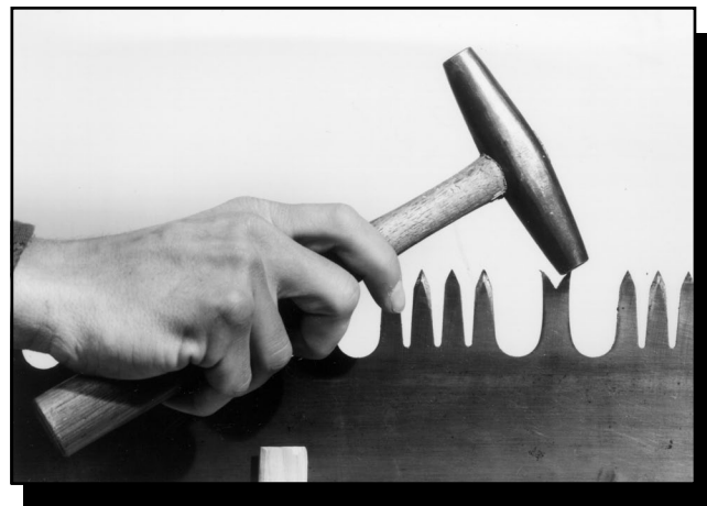
Figure 23—Striking the inside face of the raker tip with a hammer.
