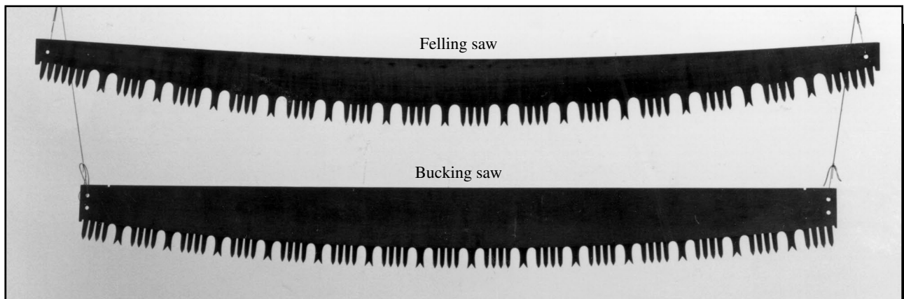
Figure 4—Felling saws have a curved back and often have just one handle hole per side. Straight-backed bucking saws often have two holes per side.
