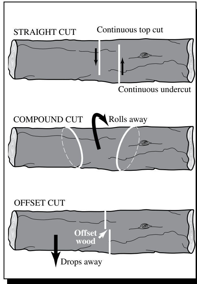
Figure 47—Three basic cuts: straight, compound, and offset.
