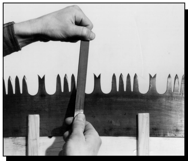
Figure 24—Filing a cutter tooth.
