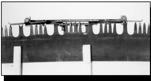
Figure 21—Jointing a saw with a long jointer, the preferred tool.
