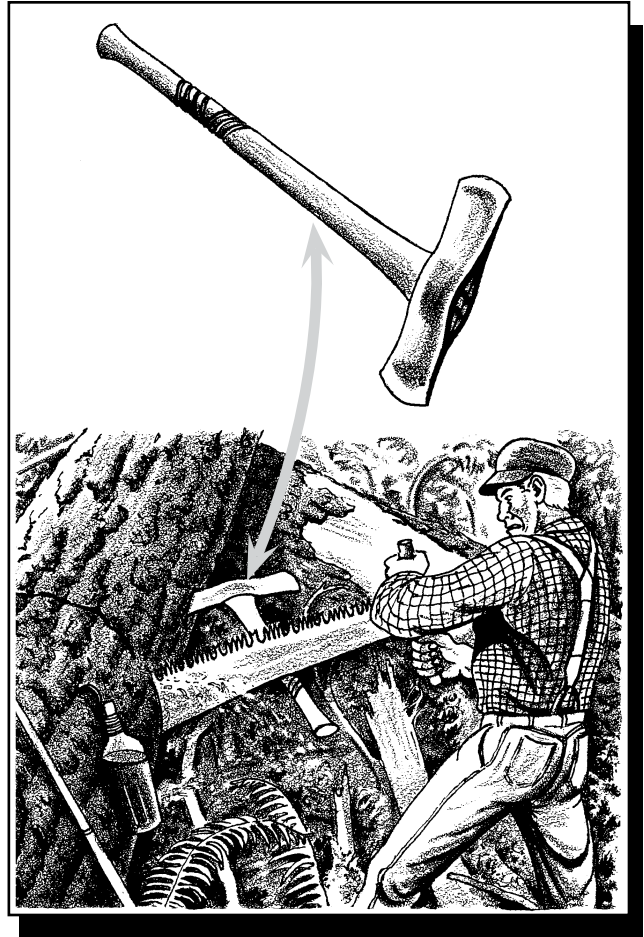
Figure 41—A double-bit ax that has been modified and grooved for underbucking. Usually a less-than-favorite ax was dedicated to this purpose.—Now You're Logging, by Bus Griffiths, with permission of Harbour Publishing, Madeira Park, BC, Canada
