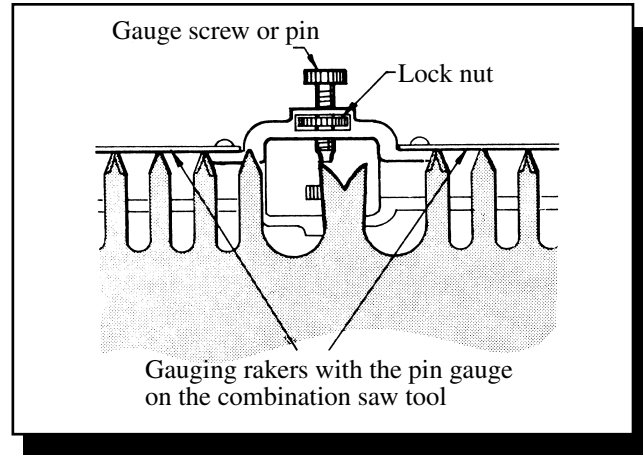
Figure 22—Gauging rakers.
