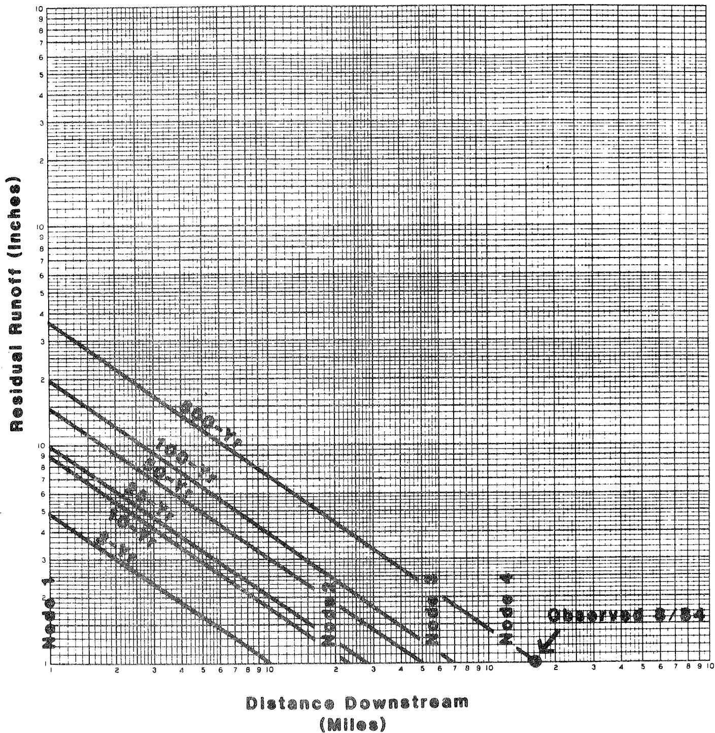
Figure 6 Local Thunderstorm AMC-I Residual Runoff vs. Distance Downstream
