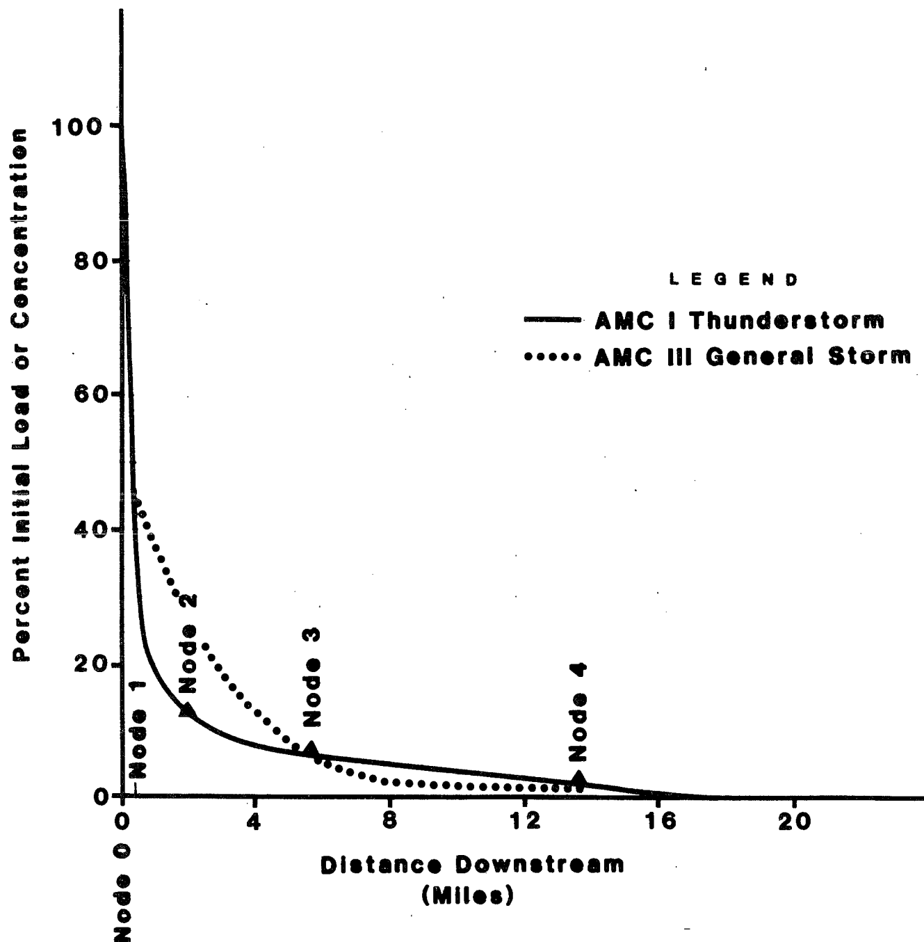
Figure 7 Estimated Downstream Effects Of Introduced Sediment or Leachate From Proposed Canyon Mine For Thunderstorm & General Storm Flood Occurrences.
