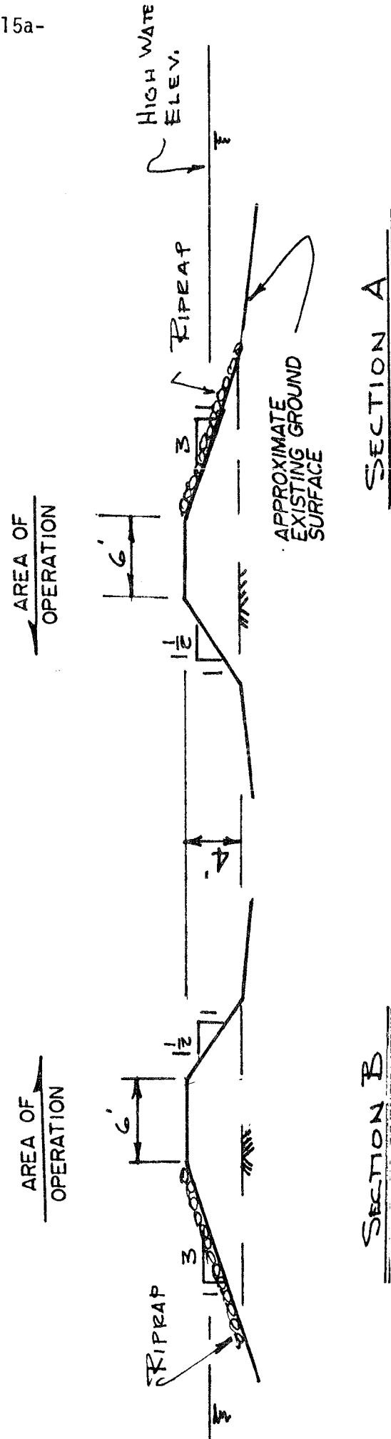
Figure 4A- Cross Sections For Proposed Drainage Plan (Top) and Alternative 2 (Bottom).
