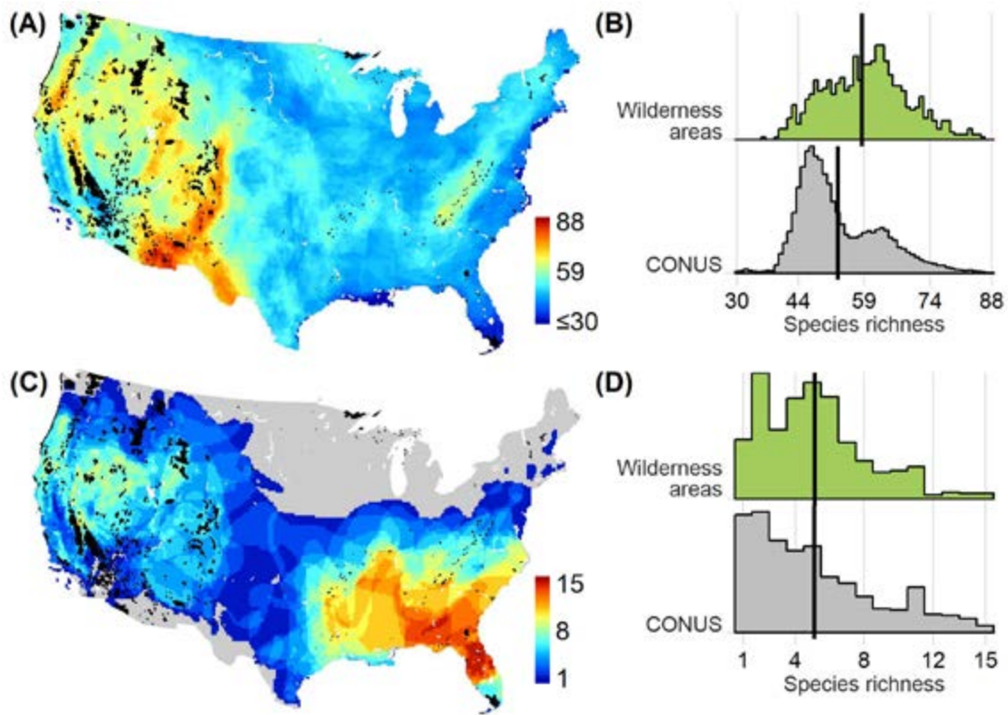
Figure 2.7—Geographic distribution and number of (A, B) mammal species (n = 359) and (C, D) endemic mammal species (n = 102) occurring within the CONUS and wilderness areas (shown in black). The vertical black line indicates the mean species richness value (B, D). Data from Jenkins and others (2015). See McCarley and Aycrigg (2020) and Jenkins and others (2015) for more details.
