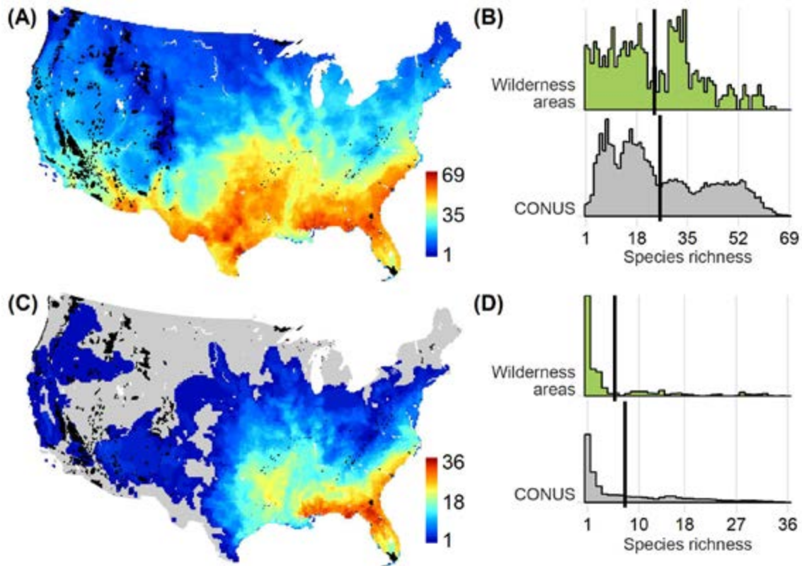
Figure 2.8—Geographic distribution and number of (A, B) reptile species (n = 295) and (C, D) endemic reptile species (n = 89) occurring within the CONUS and wilderness areas (shown in black). The vertical black line indicates the mean species richness value (B, D). Data from Jenkins and others (2015). See McCarley and Aycrigg (2020) and Jenkins and others (2015) for more details.
