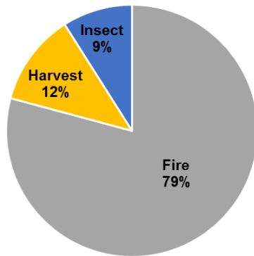
Effect of Different Disturbances, 1990-2011, on Carbon Storage in Lincoln National Forest
