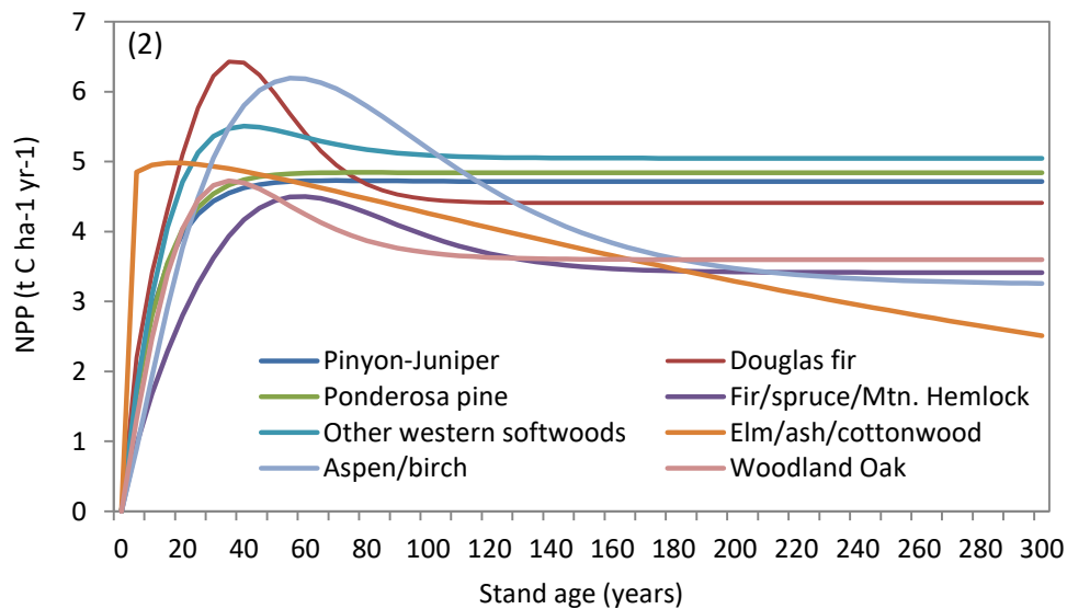
Figure 4.2. Relationship between net primary productivity (NPP) and stand age for each forest type in the Coronado National Forest.
