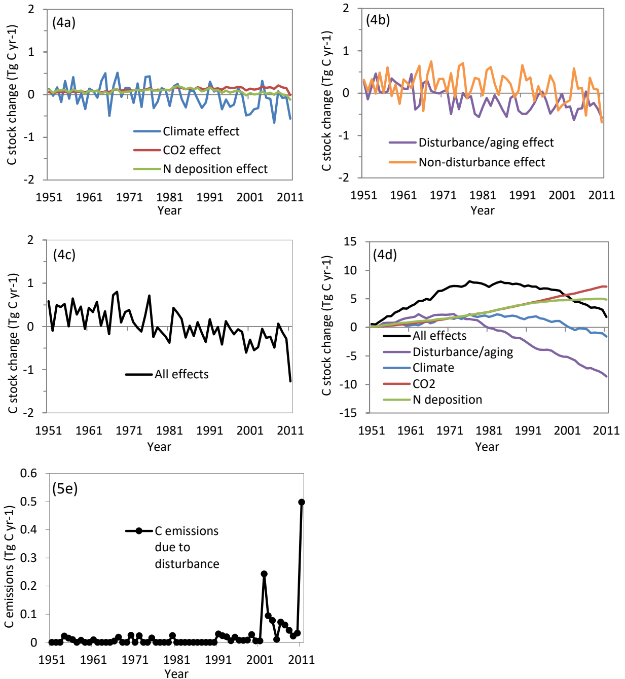
Figure 4.4. Changes in carbon stocks in the Apache-Sitgreaves National Forest due to: (a) individual non-disturbance factors alone including climate variability, atmospheric CO 2 concentration, and nitrogen deposition; (b) all disturbance factors such as fire, harvest, and insects, as well as regrowth and aging and the sum of all non-disturbance factors combined; and (c) all factors combined which is the sum of disturbance\aging and non-disturbance effects; (d) Accumulated C due to individual disturbance\aging and non-disturbance factors and all factors combined from 1950-2011 excluding C accumulated pre-1950; and (e) C emissions due to disturbance events only. Positive values in Figures 4.4 a-c represent C sinks from the atmosphere or enhancement effects, whereas negative values represent C sources to the atmosphere, or detracting effects.
