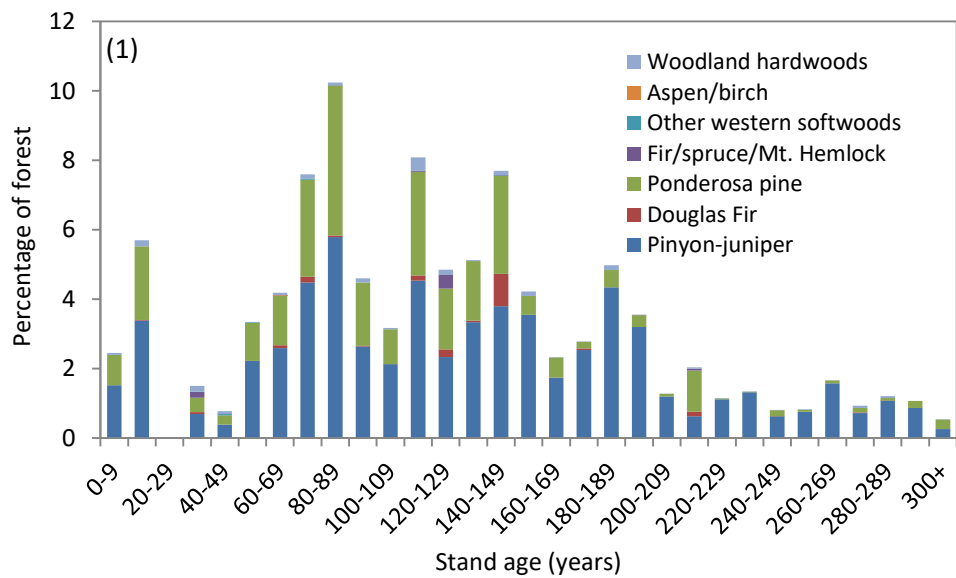
Figure 4.1. Age class distribution in 2011 in the Cibola National Forest displaying the percentage of forested area of each forest type in 10-year age classes. Forest types are symbolized by stacked, colored bars that also correspond to the forest types in Figure 2 below.
