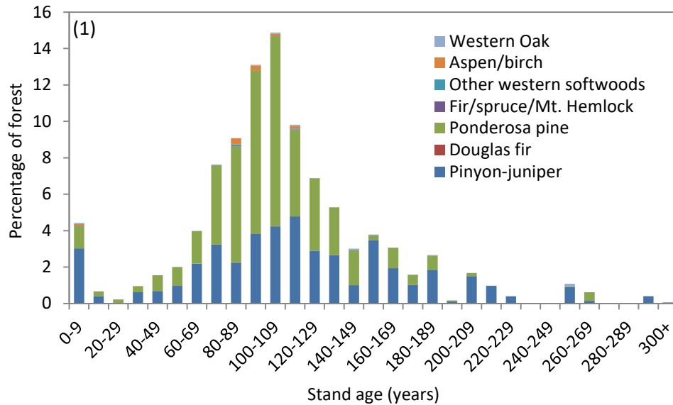
Figure 4.1. Age class distribution in 2011 in the Coconino National Forest displaying the percentage of forested area of each forest type in 10-year age classes. Forest types are symbolized by stacked, colored bars that also correspond to the forest types in Figure 2 below.
