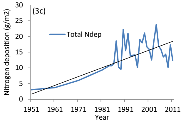
Figure 4.3. (a) Total annual precipitation (cm), (b) average annual temperature (°C), and (c) total annual nitrogen deposition from 1950-2011 in the Prescott National Forest. Linear trend lines shown in black.
