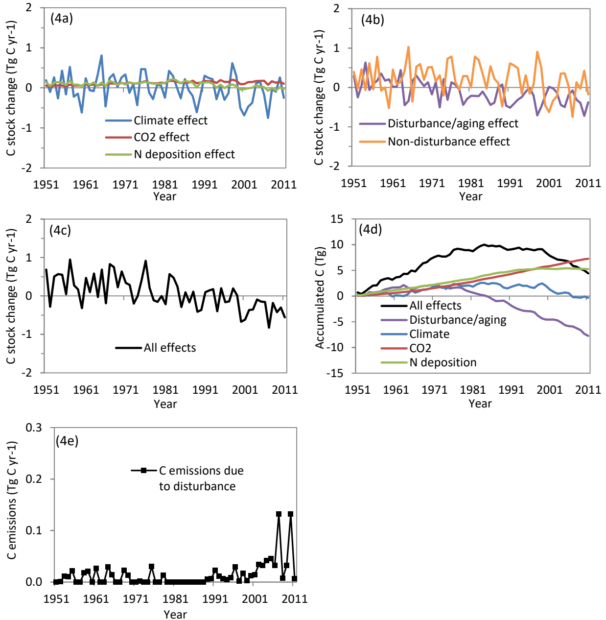
Figure 4.4. Changes in carbon stocks in the Coconino National Forest due to: (a) individual non-disturbance factors alone including climate variability, atmospheric CO 2 concentration, and nitrogen deposition; (b) all disturbance factors such as fire, harvest, and insects, as well as regrowth and aging and the sum of all non-disturbance factors combined; and (c) all factors combined which is the sum of disturbance\aging and non-disturbance effects; (d) Accumulated C due to individual disturbance\aging and non-disturbance factors and all factors combined from 1950-2011 excluding C accumulated pre-1950; and (e) C emissions due to disturbance events only. Positive values in Figures 4.4 a-c represent C sinks from the atmosphere or enhancement effects, whereas negative values represent C sources to the atmosphere, or detracting effects.
