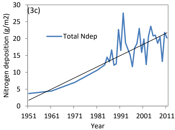
Figure 4.3. (a) Total annual precipitation (cm), (b) average annual temperature (°C), and (c) total annual nitrogen deposition from 1950-2011 in the Tonto National Forest. Linear trend lines shown in black.
