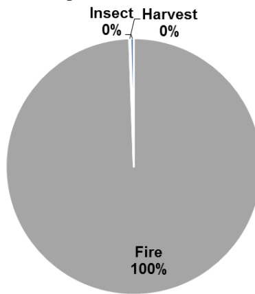
Effect of Different Disturbances, 1990-2011, on Carbon Storage in Coronado National Forest
