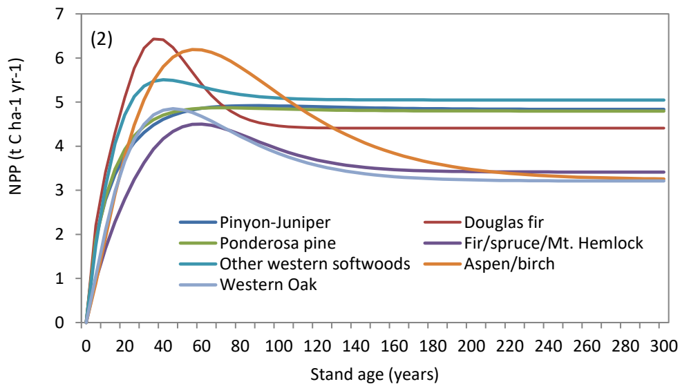
Figure 4.2. Relationship between net primary productivity (NPP) and stand age for each forest type in the Apache-Sitgreaves National Forest.
