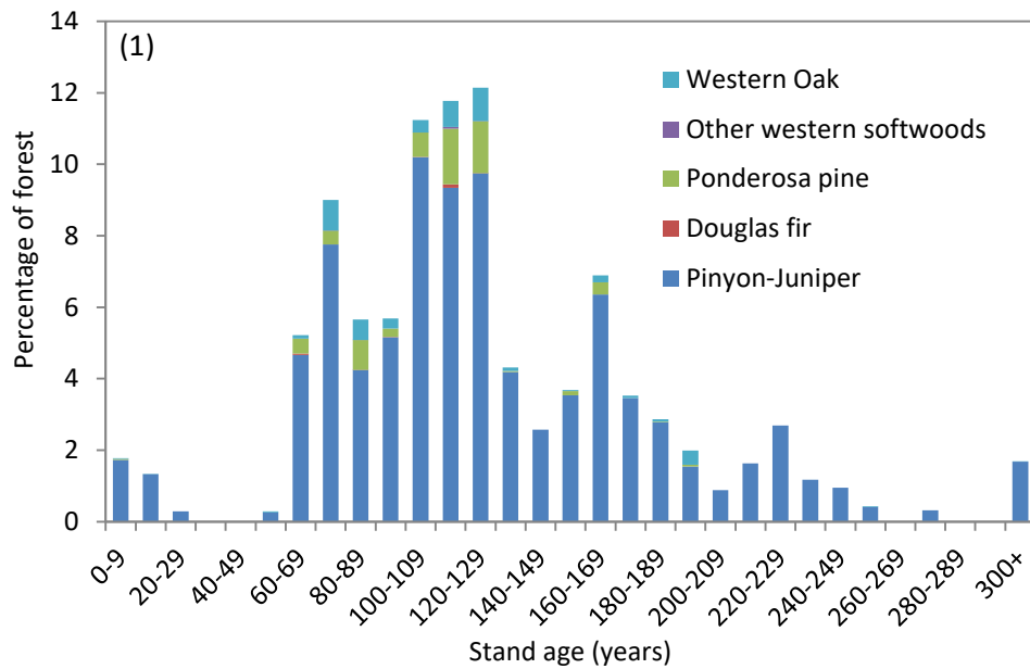
Figure 4.1. Age class distribution in 2011 in the Prescott National Forest displaying the percentage of forested area of each forest type in 10-year age classes. Forest types are symbolized by stacked, colored bars that also correspond to the forest types in Figure 2 below.
