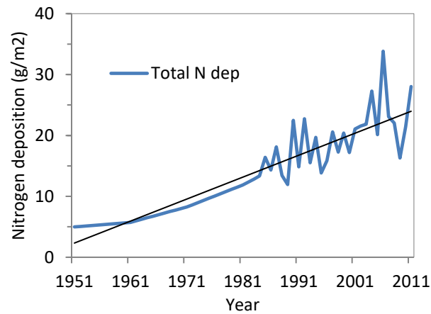
Figure 4.3. (a) Total annual precipitation (cm), (b) average annual temperature (°C), and (c) total annual nitrogen deposition from 1950-2011 in the Apache-Sitgreaves National Forest. Linear trend lines shown in black.
