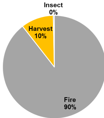
Effect of Different Disturbances, 1990-2011, on Carbon Storage in Apache-Sitgreaves National Forest
