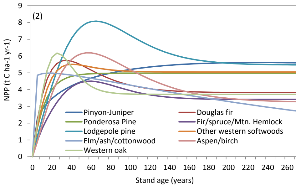
Figure 4.2. Relationship between net primary productivity (NPP) and stand age for each forest type in the Santa Fe National Forest.
