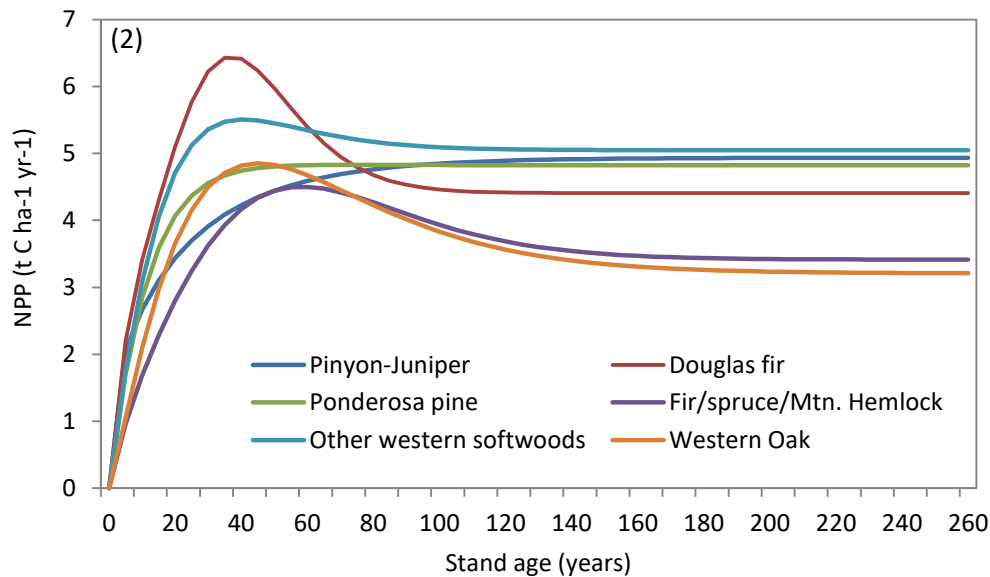
Figure 4.2. Relationship between net primary productivity (NPP) and stand age for each forest type in the Tonto National Forest.
