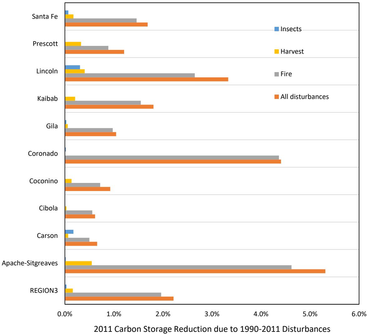
Figure 3.1. Carbon stock reduction in 2011 due to disturbances occurring from 1990 through 2011, by each national forest and for all national forests in the Southwestern Region. Percent reduction represents how much nonsoil carbon was lost from the baseline forest inventory carbon stock estimates.
