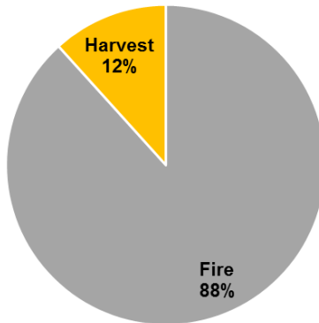
Effect of Different Disturbances, 1990-2011, on Carbon Storage in Kaibab National Forest
