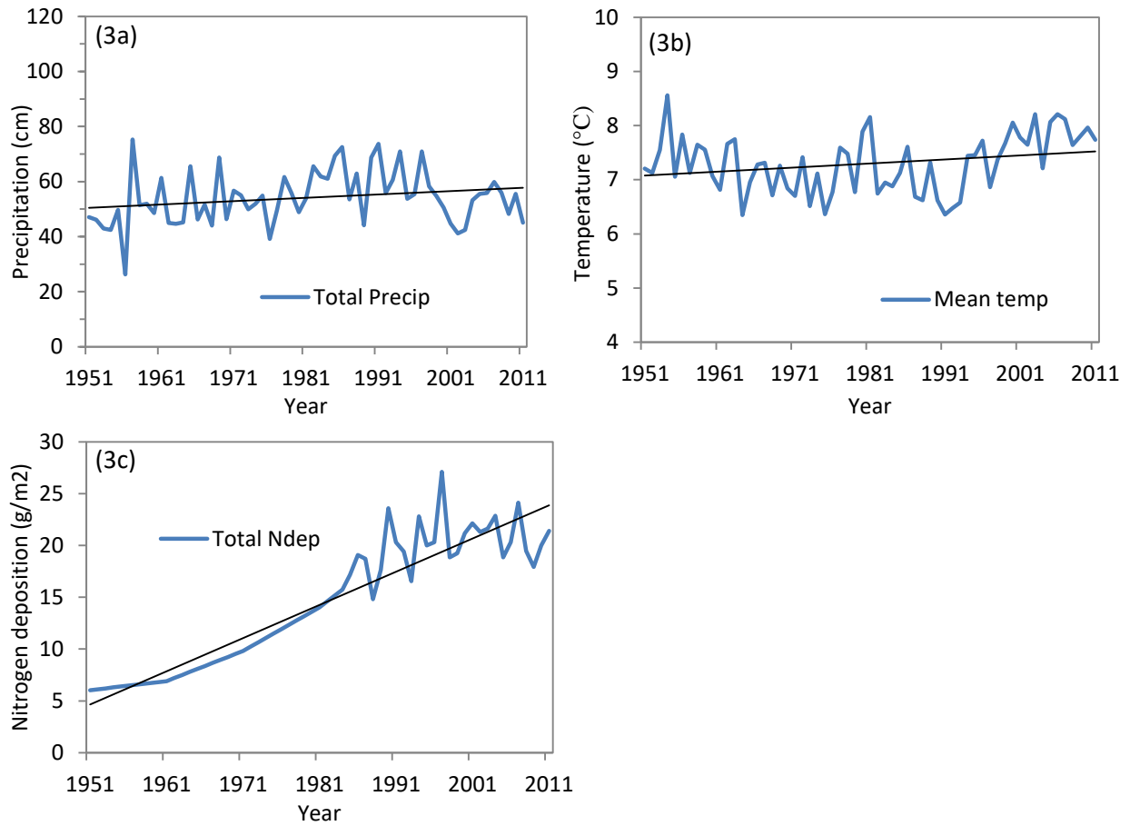
Figure 4.3. (a) Total annual precipitation (cm), (b) average annual temperature (°C), and (c) total annual nitrogen deposition from 1950-2011 in the Santa Fe National Forest. Linear trend lines shown in black.
