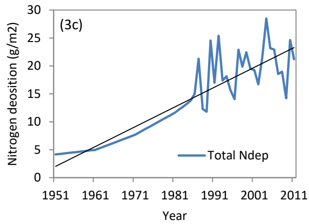
Figure 4.3. (a) Total annual precipitation (cm), (b) average annual temperature (°C), and (c) total annual nitrogen deposition from 1950-2011 in the Coconino National Forest. Linear trend lines shown in black.
