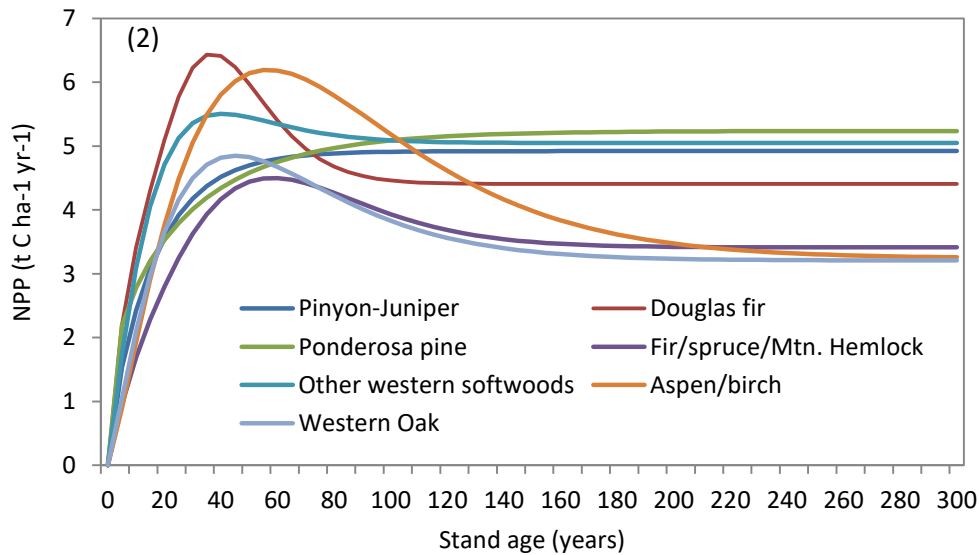
Figure 4.2. Relationship between net primary productivity (NPP) and stand age for each forest type in the Kaibab National Forest.
