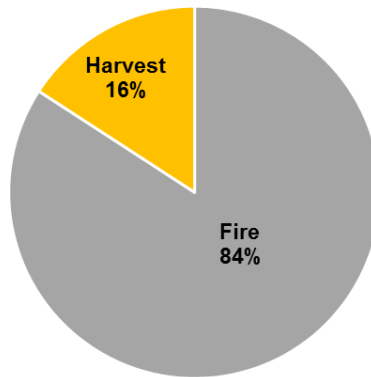
Effect of Different Disturbances, 1990-2011, on Carbon Storage in Coconino National Forest
