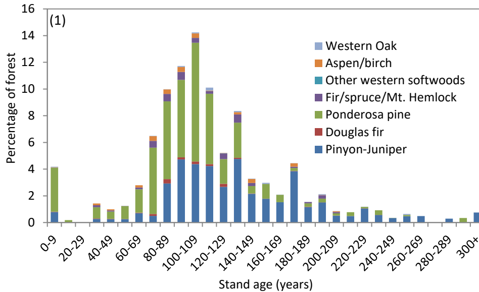
Figure 4.1. Age class distribution in 2011 in the Apache-Sitgreaves National Forest displaying the percentage of forested area of each forest type in 10-year age classes. Forest types are symbolized by stacked, colored bars that also correspond to the forest types in Figure 2 below.
