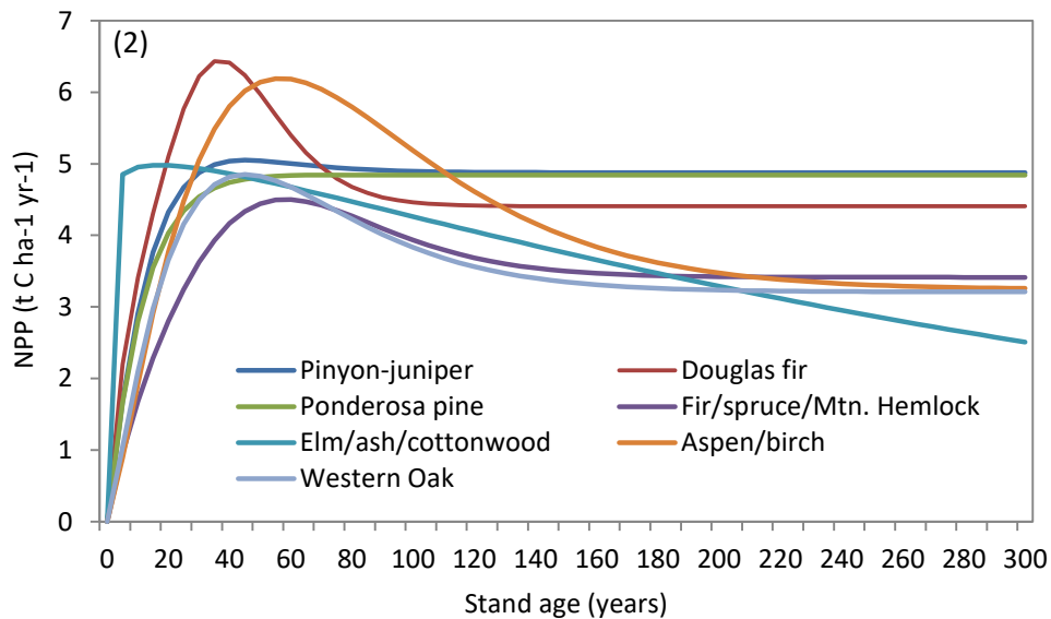
Figure 4.2. Relationship between net primary productivity (NPP) and stand age for each forest type in the Gila National Forest.
