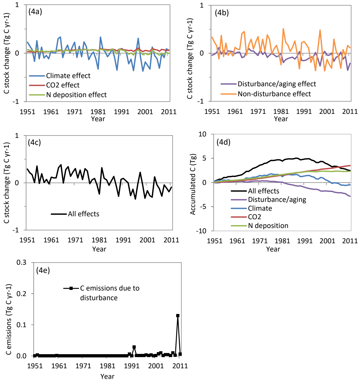
Figure 4.4. Changes in carbon stocks in the Prescott National Forest due to: (a) individual non-disturbance factors alone including climate variability, atmospheric CO 2 concentration, and nitrogen deposition; (b) all disturbance factors such as fire, harvest, and insects, as well as regrowth and aging and the sum of all non-disturbance factors combined; and (c) all factors combined which is the sum of disturbance\aging and non-disturbance effects; (d) Accumulated C due to individual disturbance\aging and non-disturbance factors and all factors combined from 1950-2011 excluding C accumulated pre-1950; and (e) C emissions due to disturbance events only. Positive values in Figures 4.4 a-c represent C sinks from the atmosphere or enhancement effects, whereas negative values represent C sources to the atmosphere, or detraction effects.
