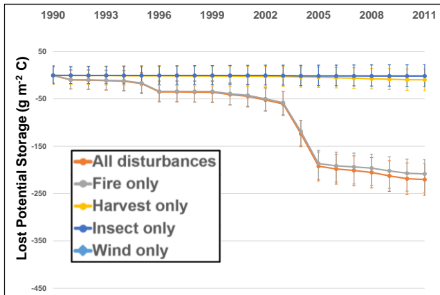
Figure 2.1. The impact of different kinds of disturbance, occurring from 1990 through 2011, on carbon (C) stores in the Southwestern Region. The difference in storage for each year is shown between an “undisturbed” scenario and a scenario that includes only observed amounts of the specified type of disturbance. Error bars represent a 95-percent confidence interval; 100 g/m 2 equals 1 metric tonne (or Mg)/ha.
