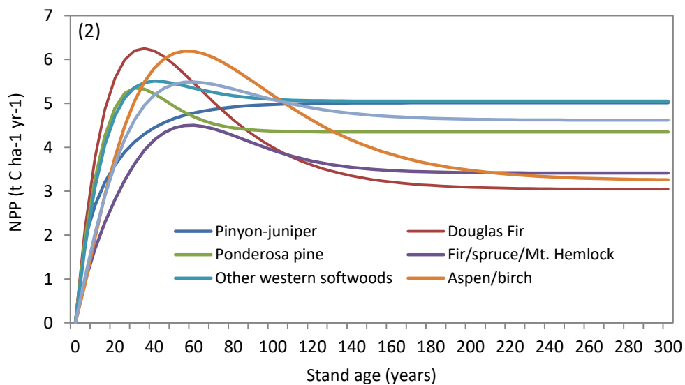
Figure 4.2. Relationship between net primary productivity (NPP) and stand age for each forest type in the Cibola National Forest.
