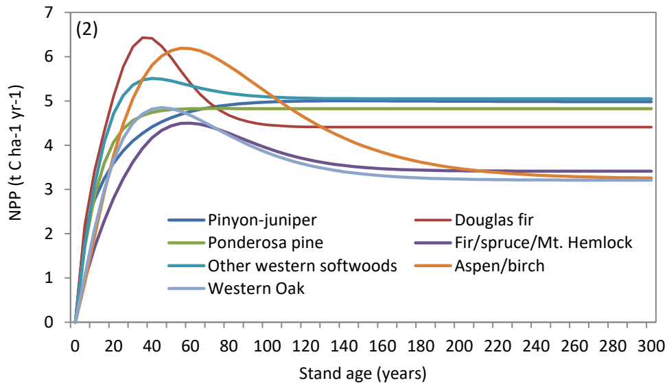
Figure 4.2. Relationship between net primary productivity (NPP) and stand age for each forest type in the Coconino National Forest.
