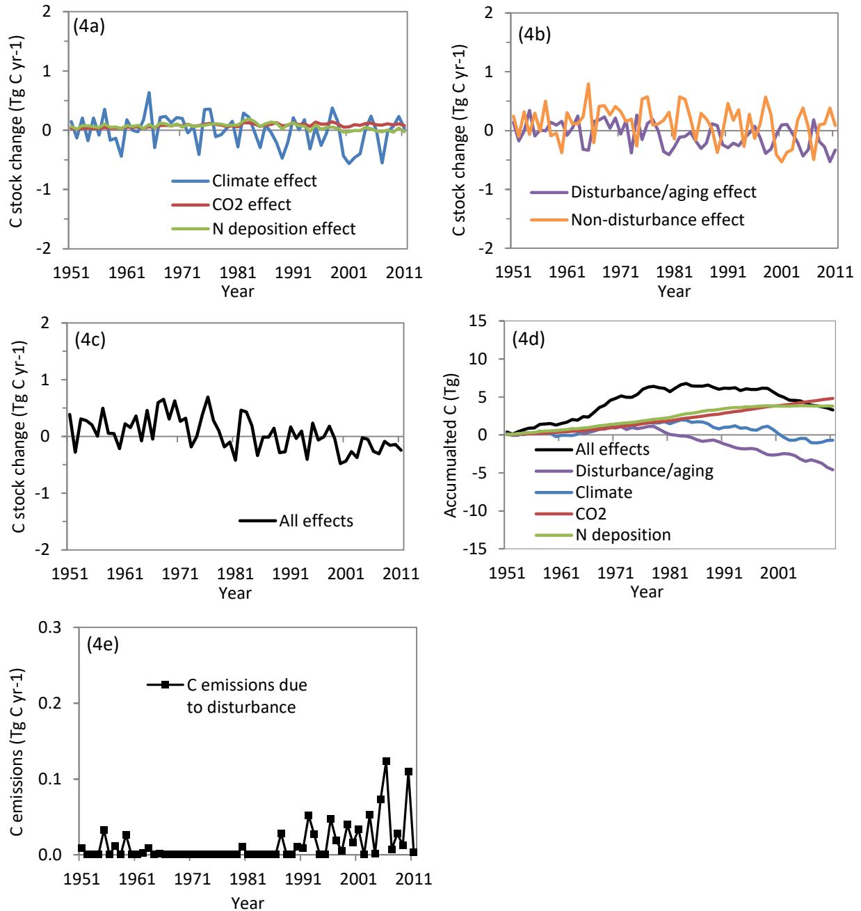
Figure 4.4. Changes in carbon stocks in the Kaibab National Forest due to: (a) individual non-disturbance factors alone including climate variability, atmospheric CO 2 concentration, and nitrogen deposition; (b) all disturbance factors such as fire, harvest, and insects, as well as regrowth and aging and the sum of all non-disturbance factors combined; and (c) all factors combined which is the sum of disturbance\aging and non-disturbance effects; (d) Accumulated C due to individual disturbance\aging and non-disturbance factors and all factors combined from 1950-2011 excluding C accumulated pre-1950; and (e) C emissions due to disturbance events only. Positive values in Figures 4.4 a-c represent C sinks from the atmosphere or enhancement effects, whereas negative values represent C sources to the atmosphere, or detracting effects.
