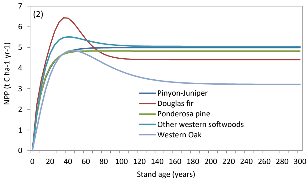
Figure 4.2. Relationship between net primary productivity (NPP) and stand age for each forest type in the Prescott National Forest.
