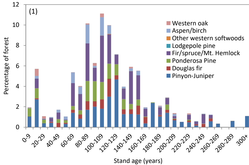
Figure 4.1. Age class distribution in 2011 in the Carson National Forest displaying the percentage of forested area of each forest type in 10-year age classes. Forest types are symbolized by stacked, colored bars that also correspond to the forest types in Figure 2 below.
