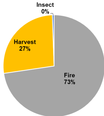
Effect of Different Disturbances, 1990-2011, on Carbon Storage in Prescott National Forest
