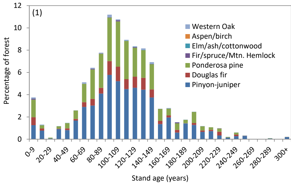
Figure 4.1. Age class distribution in 2011 in the Gila National Forest displaying the percentage of forested area of each forest type in 10-year age classes. Forest types are symbolized by stacked, colored bars that also correspond to the forest types in Figure 2 below.
