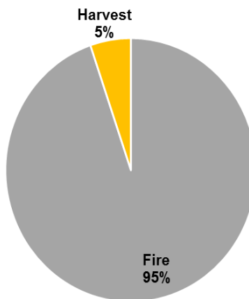
Effect of Different Disturbances, 1990-2011, on Carbon Storage in Cibola National Forest
