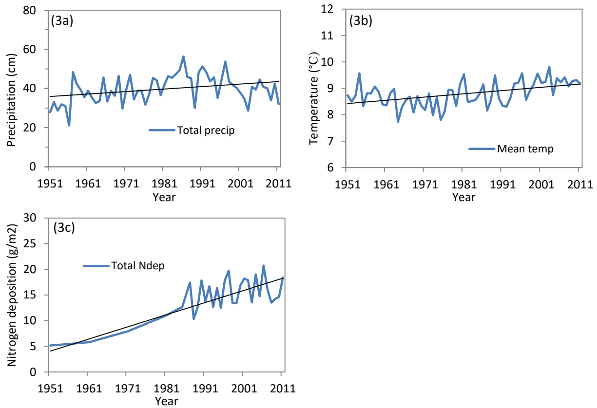
Figure 4.3. (a) Total annual precipitation (cm), (b) average annual temperature (°C), and (c) total annual nitrogen deposition from 1950-2011 in the Cibola National Forest. Linear trend lines shown in black.
