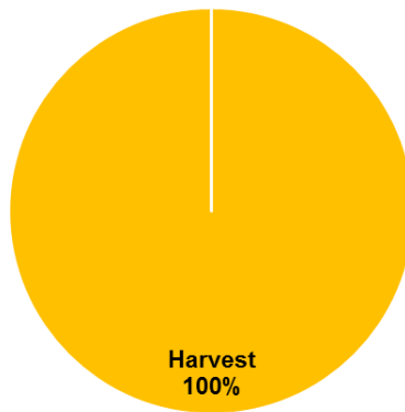
Effect of Different Disturbances, 1990-2011, on Carbon Storage in Allegheny
