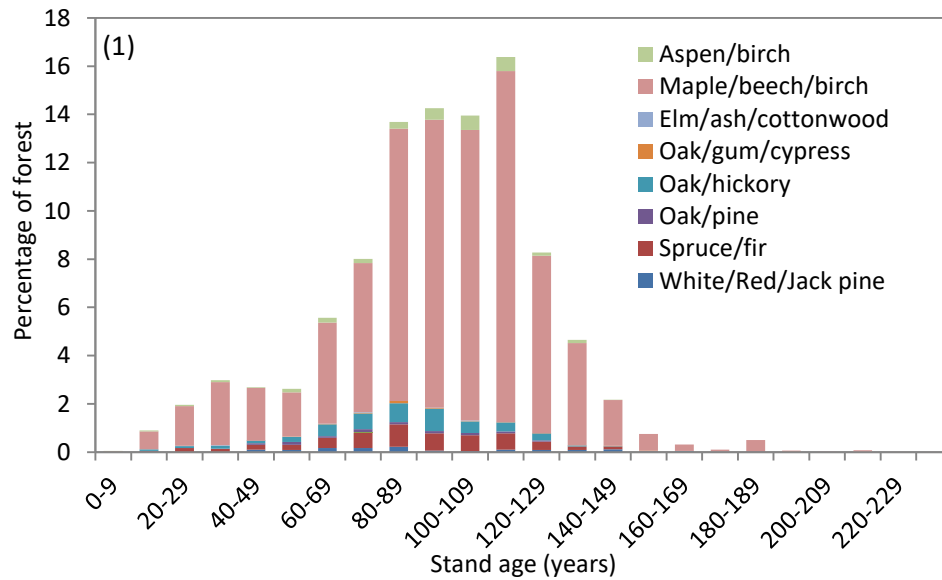
Figure 4.1. Age class distribution in 2011 in the Green Mountain and Finger Lakes National Forests displaying the percentage of forested area of each forest type in 10-year age classes. Forest types are symbolized by stacked, colored bars that also correspond to the forest types in Figure 2 below.
