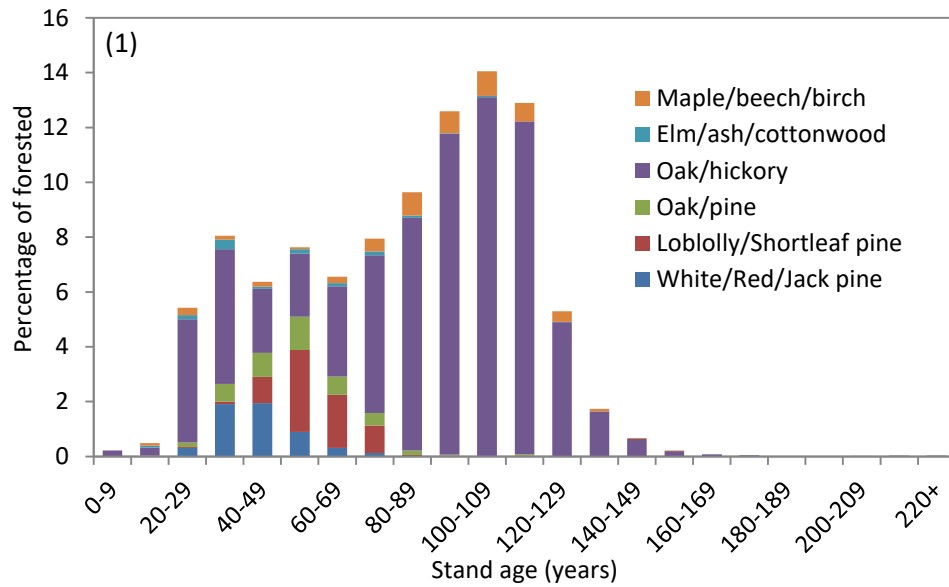
Figure 4.1. Age class distribution in 2011 in the Hoosier National Forest displaying the percentage of forested area of each forest type in 10-year age classes. Forest types are symbolized by stacked, colored bars that also correspond to the forest types in Figure 2 below.
