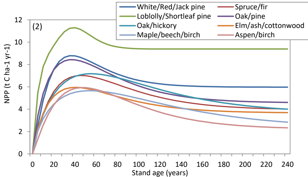
Figure 4.2. Relationship between net primary productivity (NPP) and stand age for each forest type in the Monongahela National Forest.
