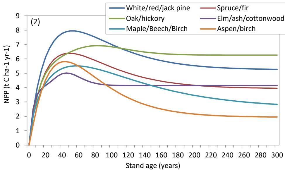
Figure 4.2. Relationship between net primary productivity (NPP) and stand age for each forest type in the Ottawa National Forest.
