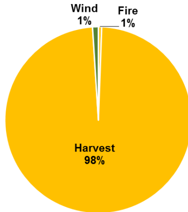
Effect of Different Disturbances, 1990-2011, on Carbon Storage in Chippewa National Forest
