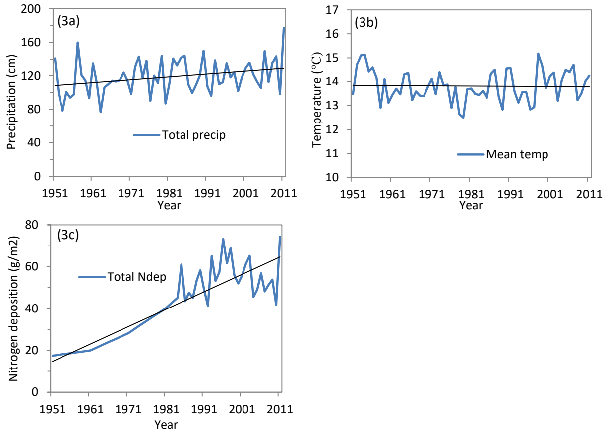
Figure 4.3. (a) Total annual precipitation (cm), (b) average annual temperature (°C), and (c) total annual nitrogen deposition from 1951-2011 in the Shawnee National Forest. Linear trend lines shown in black.
