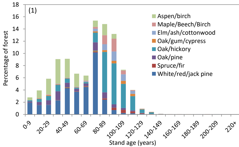
Figure 4.1. Age class distribution in 2011 in the Huron-Manistee National Forest displaying the percentage of forested area of each forest type in 10-year age classes. Forest types are symbolized by stacked, colored bars that also correspond to the forest types in Figure 2 below.
