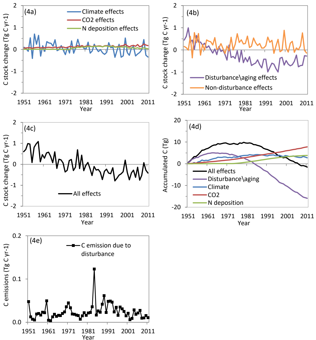
Figure 4.4. Changes in carbon stocks in the White Mountain National Forest due to: (a) individual non-disturbance factors alone including climate variability, atmospheric CO 2 concentration, and nitrogen deposition; (b) all disturbance factors such as fire, harvest, and insects, as well as regrowth and aging and the sum of all non-disturbance factors combined; and (c) all factors combined which is the sum of disturbance/aging and non-disturbance effects; (d) Accumulated C due to individual disturbance/aging and non-disturbance factors and all factors combined from 1950-2011 excluding C accumulated pre-1950; and (e) C emissions due to disturbance events only. Positive values in Figures 4.4 a-c represent C sinks from the atmosphere or enhancement effects, whereas negative values represent C sources to the atmosphere, or detracting effects.
