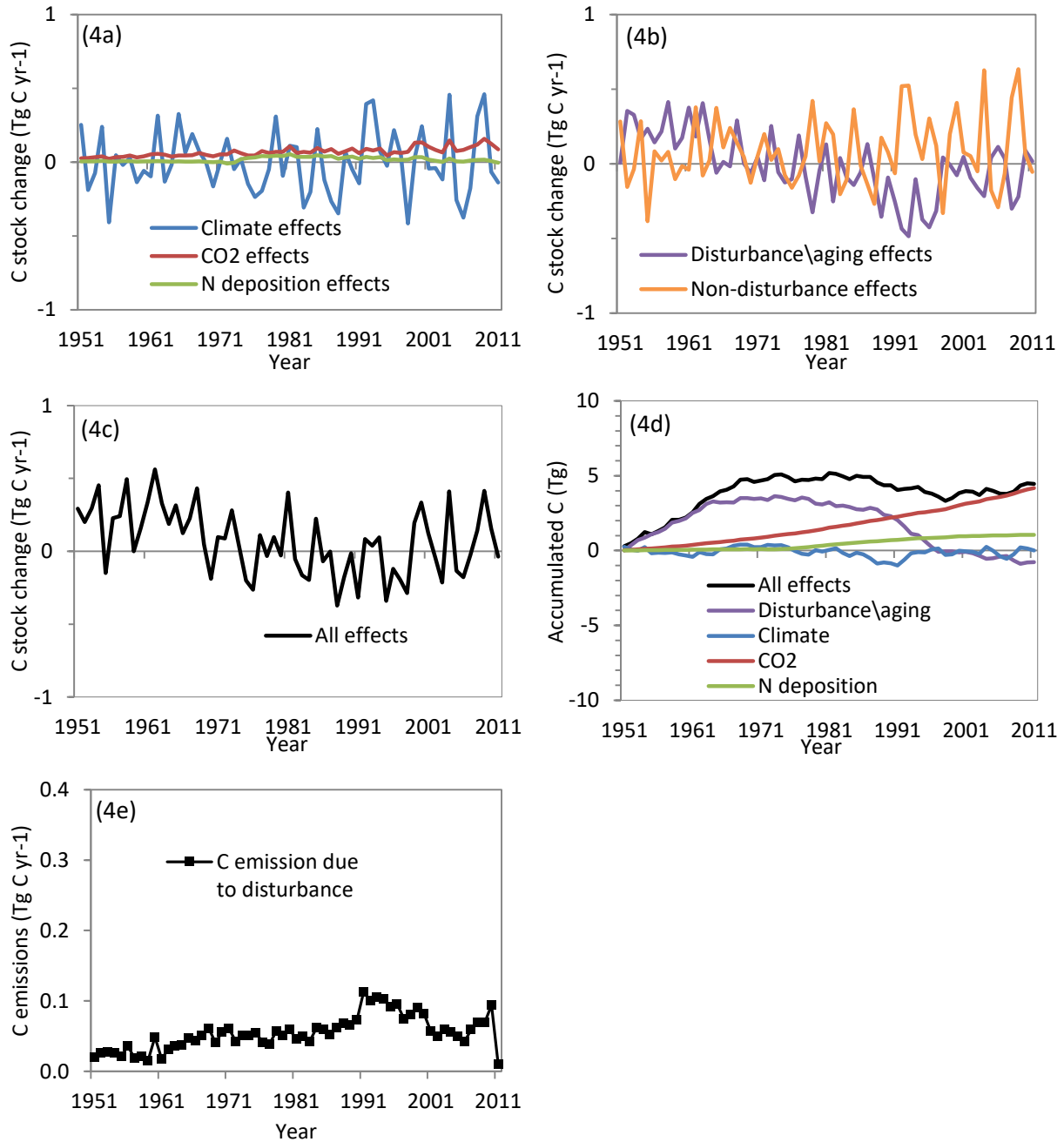
Figure 4.4. Changes in carbon stocks in the Chippawa National Forest due to: (a) individual non-disturbance factors alone including climate variability, atmospheric CO 2 concentration, and nitrogen deposition; (b) all disturbance factors such as fire, harvest, and insects, as well as regrowth and aging and the sum of all non-disturbance factors combined; and (c) all factors combined which is the sum of disturbance/aging and non-disturbance effects; (d) Accumulated C due to individual disturbance/aging and non-disturbance factors and all factors combined from 1950-2011 excluding C accumulated pre-1950; and (e) C emissions due to disturbance events only. Positive values in Figures 4.4 a-c represent C sinks from the atmosphere or enhancement effects, whereas negative values represent C sources to the atmosphere, or detracting effects.
