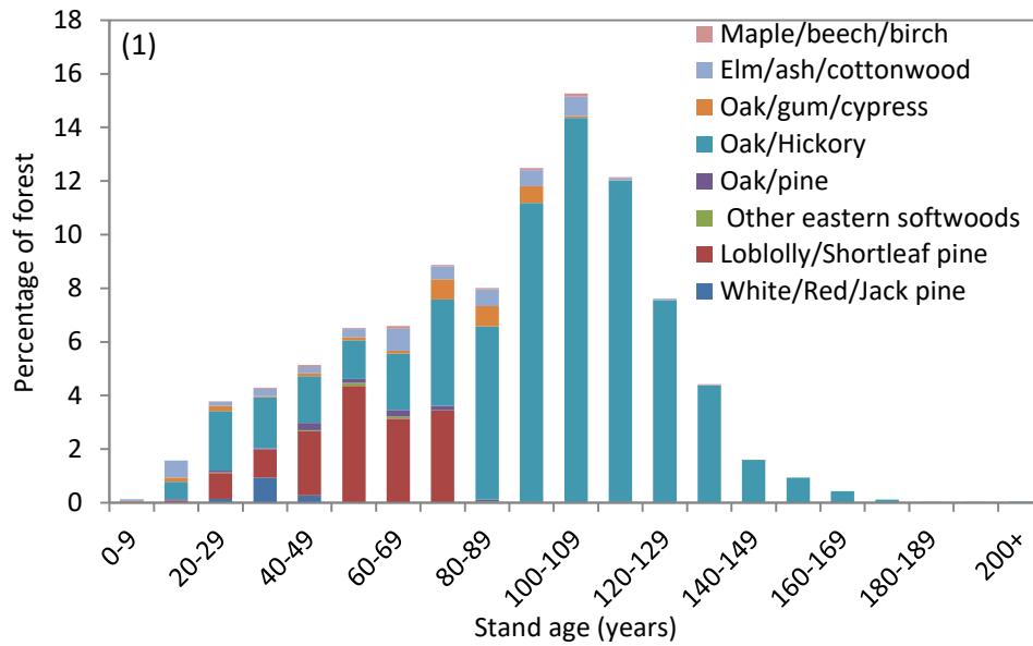
Figure 4.1. Age class distribution in 2011 in the Shawnee National Forest displaying the percentage of forested area of each forest type in 10-year age classes. Forest types are symbolized by stacked, colored bars that also correspond to the forest types in Figure 2 below.
