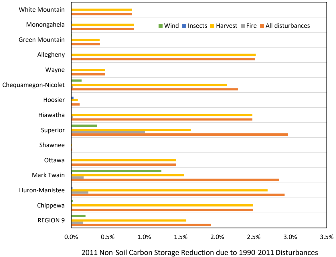
Figure 3.1. Carbon stock reduction in 2011 due to disturbances occurring from 1990 through 2011, by each national forest and for all national forests combined in the Eastern Region. Percent reduction represents how much nonsoil carbon was lost from the baseline forest inventory carbon stock estimates. “Wind” is a combination of ice and wind storms and was labelled “abiotic” in Figure 1.
