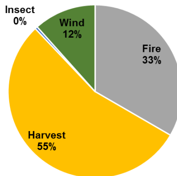
Effect of Different Disturbances, 1990-2011, on Carbon Storage in Superior National Forest
