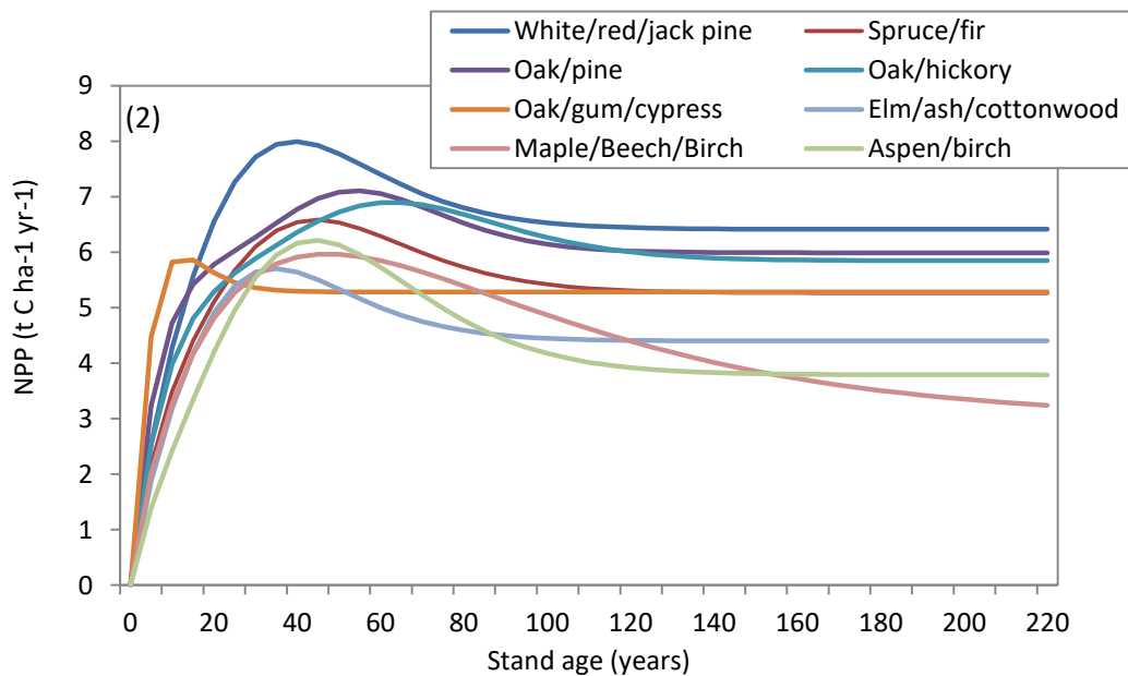
Figure 4.2. Relationship between net primary productivity (NPP) and stand age for each forest type in the Huron-Manistee National Forest.
