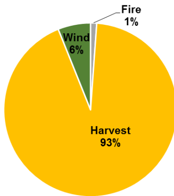
Effect of Different Disturbances, 1990-2011, on Carbon Storage in Chequamegon-Nicolet National Forest
