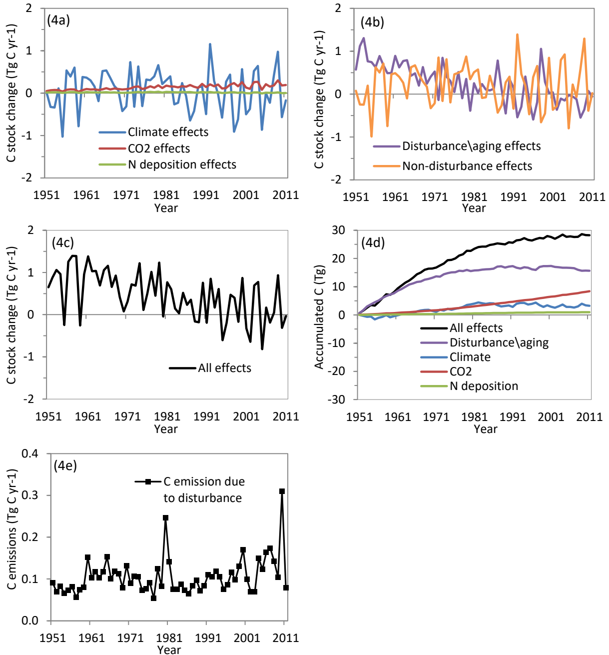
Figure 4.4. Changes in carbon stocks in the Huron-Manistee National Forest due to: (a) individual non-disturbance factors alone including climate variability, atmospheric CO 2 concentration, and nitrogen deposition; (b) all disturbance factors such as fire, harvest, and insects, as well as regrowth and aging and the sum of all non-disturbance factors combined; and (c) all factors combined which is the sum of disturbance\aging and non-disturbance effects; (d) Accumulated C due to individual disturbance\aging and non-disturbance factors and all factors combined from 1950-2011 excluding C accumulated pre-1950; and (e) C emissions due to disturbance events only. Positive values in Figures 4.4 a-c represent C sinks from the atmosphere or enhancement effects, whereas negative values represent C sources to the atmosphere, or detraction effects.
