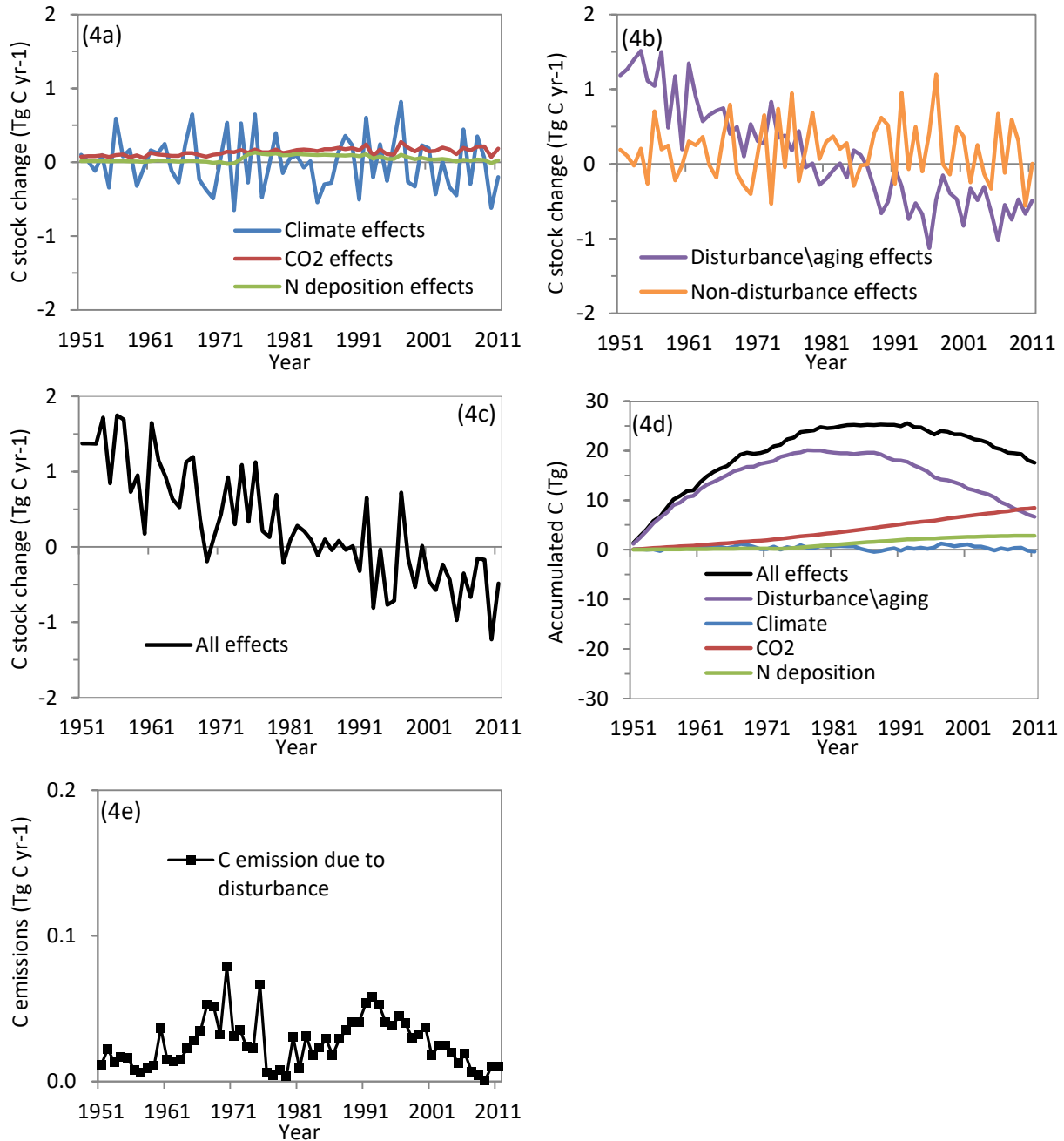
Figure 4.4. Changes in carbon stocks in the Monongahela National Forest due to: (a) individual non-disturbance factors alone including climate variability, atmospheric CO 2 concentration, and nitrogen deposition; (b) all disturbance factors such as fire, harvest, and insects, as well as regrowth and aging and the sum of all non-disturbance factors combined; and (c) all factors combined which is the sum of disturbance/aging and non-disturbance effects; (d) Accumulated C due to individual disturbance/aging and non-disturbance factors and all factors combined from 1950-2011 excluding C accumulated pre-1950; and (e) C emissions due to disturbance events only. Positive values in Figures 4.4 a-c represent C sinks from the atmosphere or enhancement effects, whereas negative values represent C sources to the atmosphere, or detracting effects.
