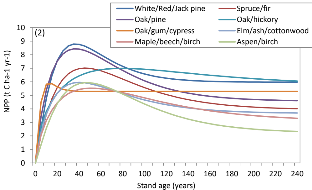
Figure 4.2. Relationship between net primary productivity (NPP) and stand age for each forest type in the Green Mountain and Finger Lakes National Forests.
