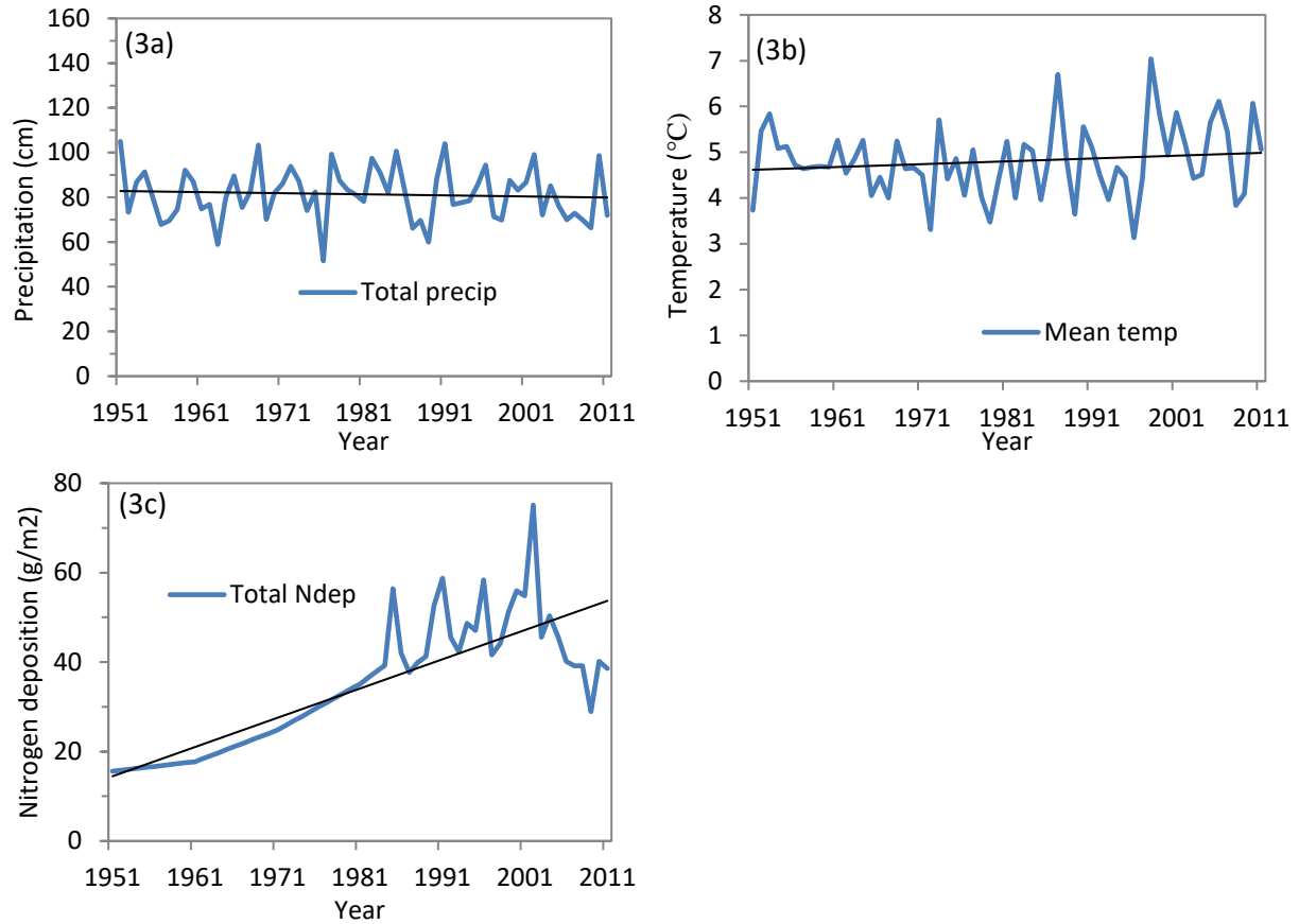
Figure 4.3. (a) Total annual precipitation (cm), (b) average annual temperature (°C), and (c) total annual nitrogen deposition from 1951-2011 in the Chequamegon-Nicolet National Forest. Linear trend lines shown in black.
