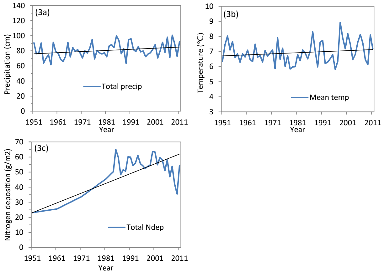
Figure 4.3. (a) Total annual precipitation (cm), (b) average annual temperature (°C), and (c) total annual nitrogen deposition from 1951-2011 in the Huron-Manistee National Forest. Linear trend lines shown in black.
