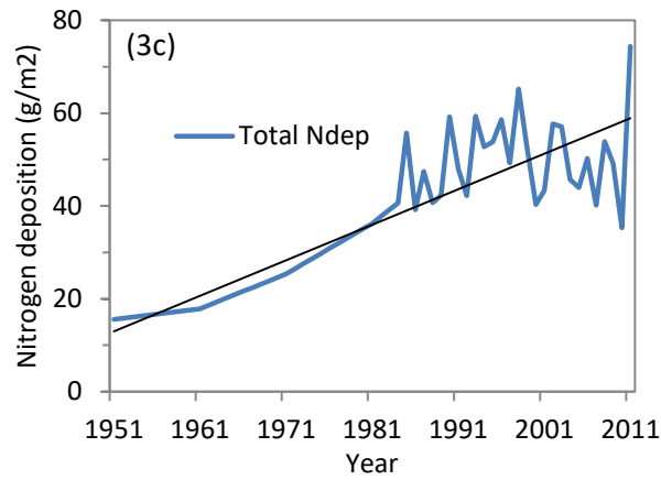
Figure 4.3. (a) Total annual precipitation (cm), (b) average annual temperature (°C), and (c) total annual nitrogen deposition from 1951-2011 in the Mark Twain National Forest. Linear trend lines shown in black.
