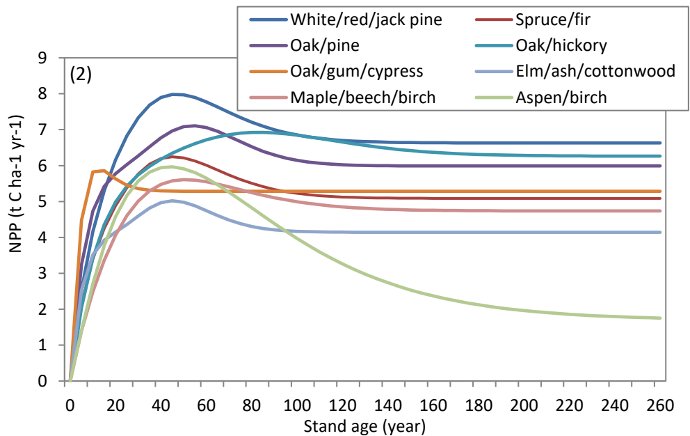
Figure 4.2. Relationship between net primary productivity (NPP) and stand age for each forest type in the Chequamegon-Nicolet National Forest.
