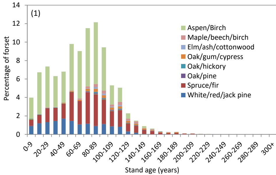
Figure 4.1. Age class distribution in 2011 in the Superior National Forest displaying the percentage of forested area of each forest type in 10-year age classes. Forest types are symbolized by stacked, colored bars that also correspond to the forest types in Figure 2 below.
