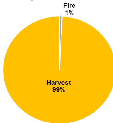
Effect of Different Disturbances, 1990-2011, on Carbon Storage in Hiawatha National Forest
