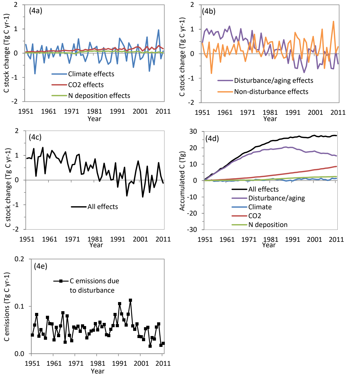
Figure 4.4. Changes in carbon stocks in the Ottawa National Forest due to: (a) individual non-disturbance factors alone including climate variability, atmospheric CO 2 concentration, and nitrogen deposition; (b) all disturbance factors such as fire, harvest, and insects, as well as regrowth and aging and the sum of all non-disturbance factors combined; and (c) all factors combined which is the sum of disturbance\aging and non-disturbance effects; (d) Accumulated C due to individual disturbance\aging and non-disturbance factors and all factors combined from 1950-2011 excluding C accumulated pre-1950; and (e) C emissions due to disturbance events only. Positive values in Figures 4.4 a-c represent C sinks from the atmosphere or enhancement effects, whereas negative values represent C sources to the atmosphere, or detracting effects.
