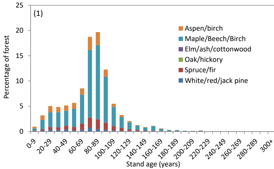
Figure 4.1. Age class distribution in 2011 in the Ottawa National Forest displaying the percentage of forested area of each forest type in 10-year age classes. Forest types are symbolized by stacked, colored bars that also correspond to the forest types in Figure 2 below.
