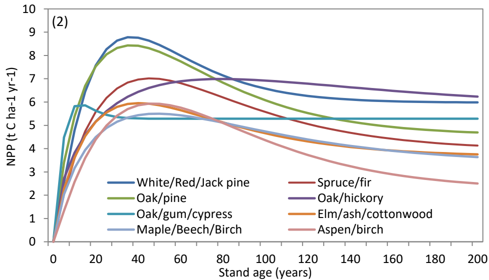
Figure 4.2. Relationship between net primary productivity (NPP) and stand age for each forest type in the Allegheny National Forest.
