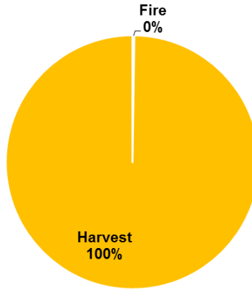
Effect of Different Disturbances, 1990-2011, on Carbon Storage in Ottawa National Forest
