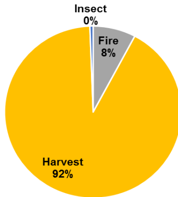
Effect of Different Disturbances, 1990-2011, on Carbon Storage in Huron-Manistee National Forest
