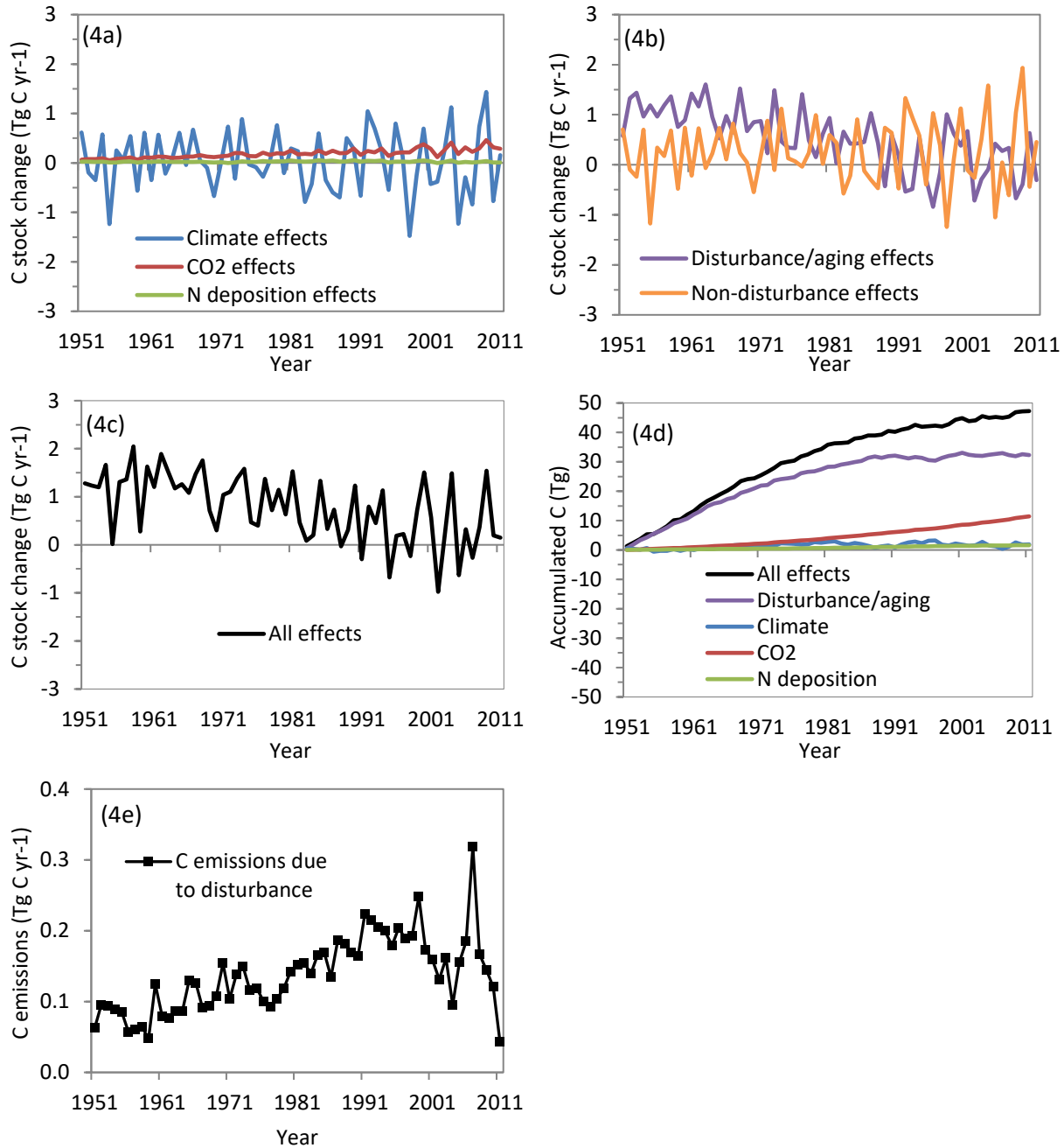
Figure 4.4. Changes in carbon stocks in the Chequamegon-Nicolet National Forest due to: (a) individual non-disturbance factors alone including climate variability, atmospheric CO 2 concentration, and nitrogen deposition; (b) all disturbance factors such as fire, harvest, and insects, as well as regrowth and aging and the sum of all non-disturbance factors combined; and (c) all factors combined which is the sum of disturbance\aging and non-disturbance effects; (d) Accumulated C due to individual disturbance\aging and non-disturbance factors and all factors combined from 1950-2011 excluding C accumulated pre-1950; and (e) C emissions due to disturbance events only. Positive values in Figures 4.4 a-c represent C sinks from the atmosphere or enhancement effects, whereas negative values represent C sources to the atmosphere, or detracting effects.
