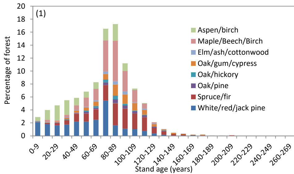
Figure 4.1. Age class distribution in 2011 in the Hiawatha National Forest displaying the percentage of forested area of each forest type in 10-year age classes. Forest types are symbolized by stacked, colored bars that also correspond to the forest types in Figure 2 below.
