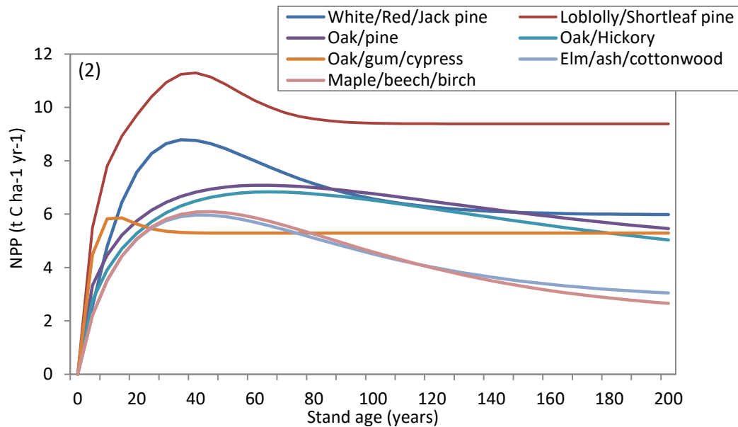
Figure 4.2. Relationship between net primary productivity (NPP) and stand age for each forest type in the Shawnee National Forest. The Loblolly/shortleaf curve was applied to the Other Eastern Softwoods forest type.
