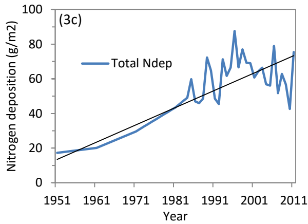
Figure 4.3. (a) Total annual precipitation (cm), (b) average annual temperature (°C), and (c) total annual nitrogen deposition from 1951-2011 in the Hoosier National Forest. Linear trend lines shown in black.
