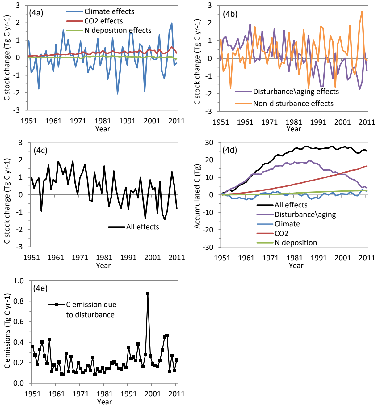
Figure 4.4. Changes in carbon stocks in the Superior National Forest due to: (a) individual non-disturbance factors alone including climate variability, atmospheric CO 2 concentration, and nitrogen deposition; (b) all disturbance factors such as fire, harvest, and insects, as well as regrowth and aging and the sum of all non-disturbance factors combined; and (c) all factors combined which is the sum of disturbance/aging and non-disturbance effects; (d) Accumulated C due to individual disturbance/aging and non-disturbance factors and all factors combined from 1950-2011 excluding C accumulated pre-1950; and (e) C emissions due to disturbance events only. Positive values in Figures 4.4 a-c represent C sinks from the atmosphere or enhancement effects, whereas negative values represent C sources to the atmosphere, or detracting effects.
