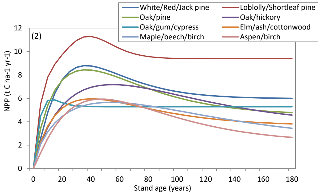
Figure 4.2. Relationship between net primary productivity (NPP) and stand age for each forest type in the Wayne National Forest.
