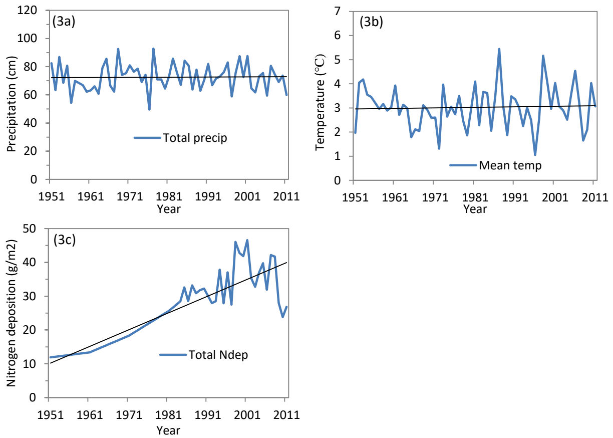
Figure 4.3. (a) Total annual precipitation (cm), (b) average annual temperature (°C), and (c) total annual nitrogen deposition from 1951-2011 in the Superior National Forest. Linear trend lines shown in black.
