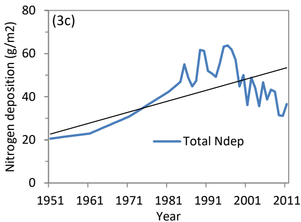
Figure 4.3. (a) Total annual precipitation (cm), (b) average annual temperature (°C), and (c) total annual nitrogen deposition from 1951-2011 in the White Mountain National Forest. Linear trend lines shown in black.
