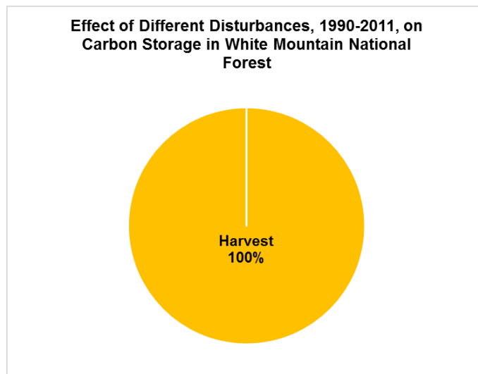
Figure 2.2. Proportional effect of different kinds of disturbance on carbon storage in each national forests in the Eastern Region for the period 1990 through 2011. “Wind” is a combination of ice and wind storms and was labelled “abiotic” in Figure 1.
