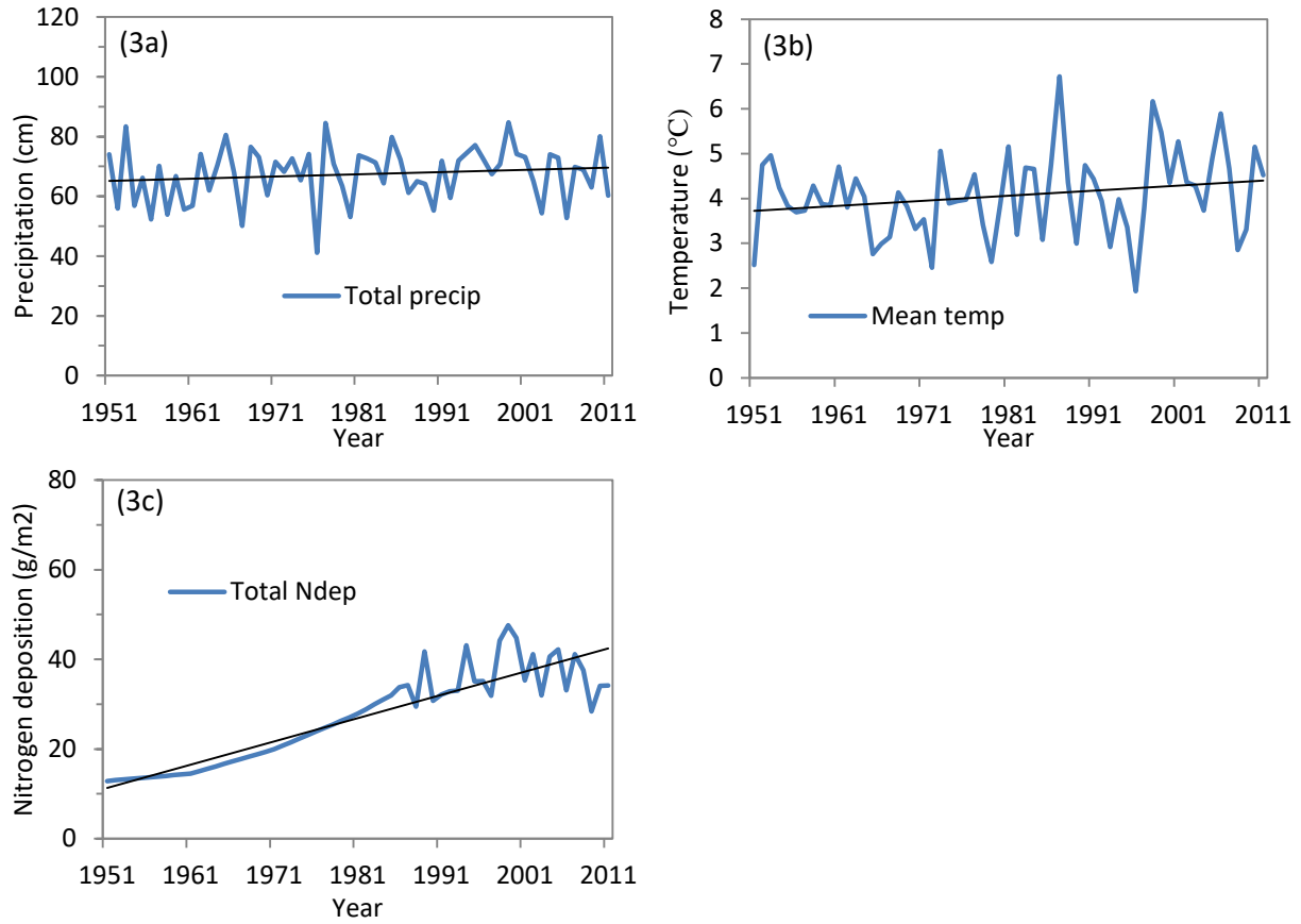
Figure 4.3. (a) Total annual precipitation (cm), (b) average annual temperature (°C), and (c) total annual nitrogen deposition from 1951-2011 in the Chippawa National Forest. Linear trend lines shown in black.
