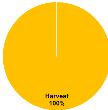
Effect of Different Disturbances, 1990-2011, on Carbon Storage in Shawnee National Forest
