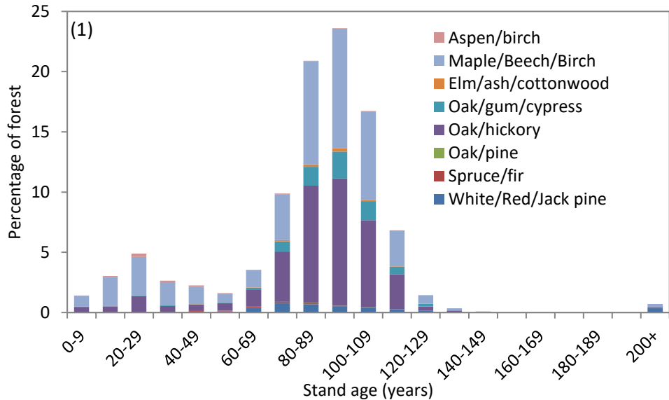
Figure 4.1. Age class distribution in 2011 in the Allegheny National Forest displaying the percentage of forested area of each forest type in 10-year age classes. Forest types are symbolized by stacked, colored bars that also correspond to the forest types in Figure 2 below.
