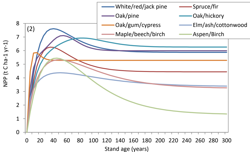
Figure 4.2. Relationship between net primary productivity (NPP) and stand age for each forest type in the Superior National Forest.
