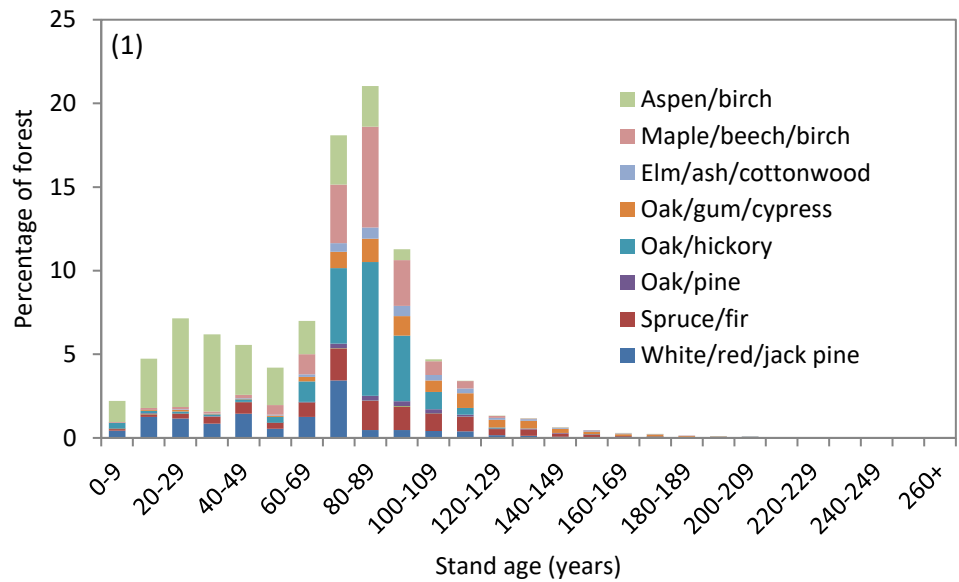
Figure 4.1. Age class distribution in 2011 in the Chequamegon-Nicolet National Forest displaying the percentage of forested area of each forest type in 10-year age classes. Forest types are symbolized by stacked, colored bars that also correspond to the forest types in Figure 2 below.
