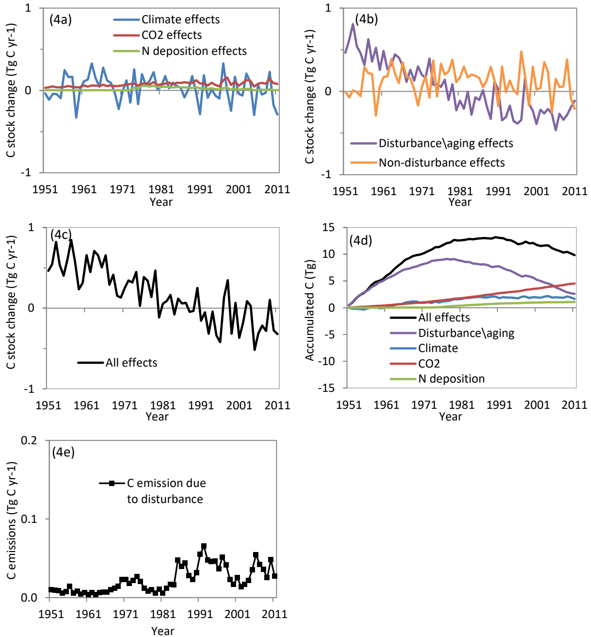
Figure 4.4. Changes in carbon stocks in the Allegheny National Forest due to: (a) individual non-disturbance factors alone including climate variability, atmospheric CO 2 concentration, and nitrogen deposition; (b) all disturbance factors such as fire, harvest, and insects, as well as regrowth and aging and the sum of all non-disturbance factors combined; and (c) all factors combined which is the sum of disturbance\aging and non-disturbance effects; (d) Accumulated C due to individual disturbance\aging and non-disturbance factors and all factors combined from 1950-2011 excluding C accumulated pre-1950; and (e) C emissions due to disturbance events only. Positive values in Figures 4.4 a-c represent C sinks from the atmosphere or enhancement effects, whereas negative values represent C sources to the atmosphere, or detracting effects.
