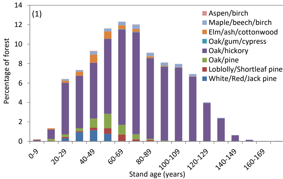
Figure 4.1. Age class distribution in 2011 in the Wayne National Forest displaying the percentage of forested area of each forest type in 10-year age classes. Forest types are symbolized by stacked, colored bars that also correspond to the forest types in Figure 2 below.
