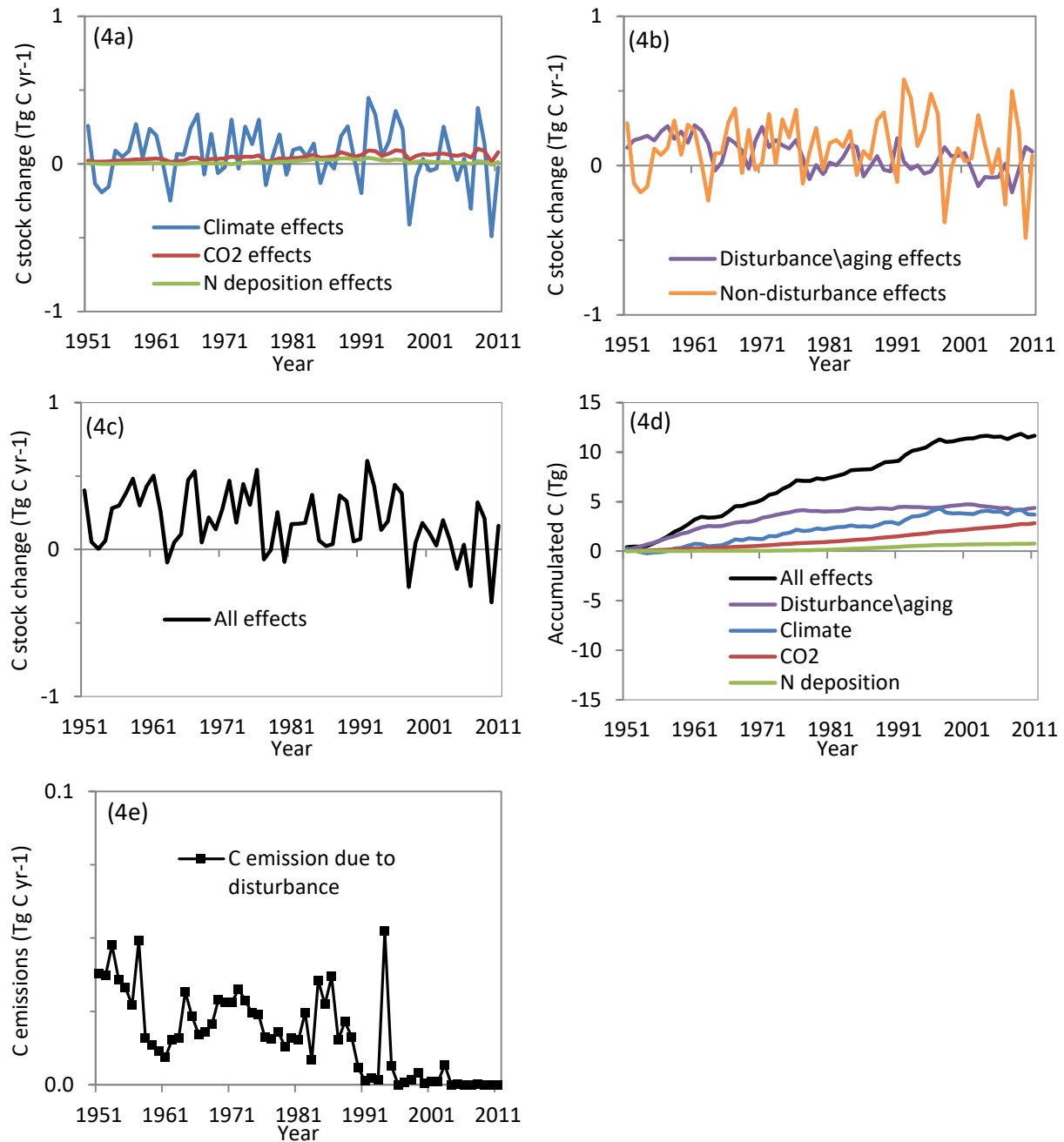
Figure 4.4. Changes in carbon stocks in the Shawnee National Forest due to: (a) individual non-disturbance factors alone including climate variability, atmospheric CO 2 concentration, and nitrogen deposition; (b) all disturbance factors such as fire, harvest, and insects, as well as regrowth and aging and the sum of all non-disturbance factors combined; and (c) all factors combined which is the sum of disturbance\aging and non-disturbance effects; (d) Accumulated C due to individual disturbance\aging and non-disturbance factors and all factors combined from 1950-2011 excluding C accumulated pre-1950; and (e) C emissions due to disturbance events only. Positive values in Figures 4.4 a-c represent C sinks from the atmosphere or enhancement effects, whereas negative values represent C sources to the atmosphere, or detracting effects.
