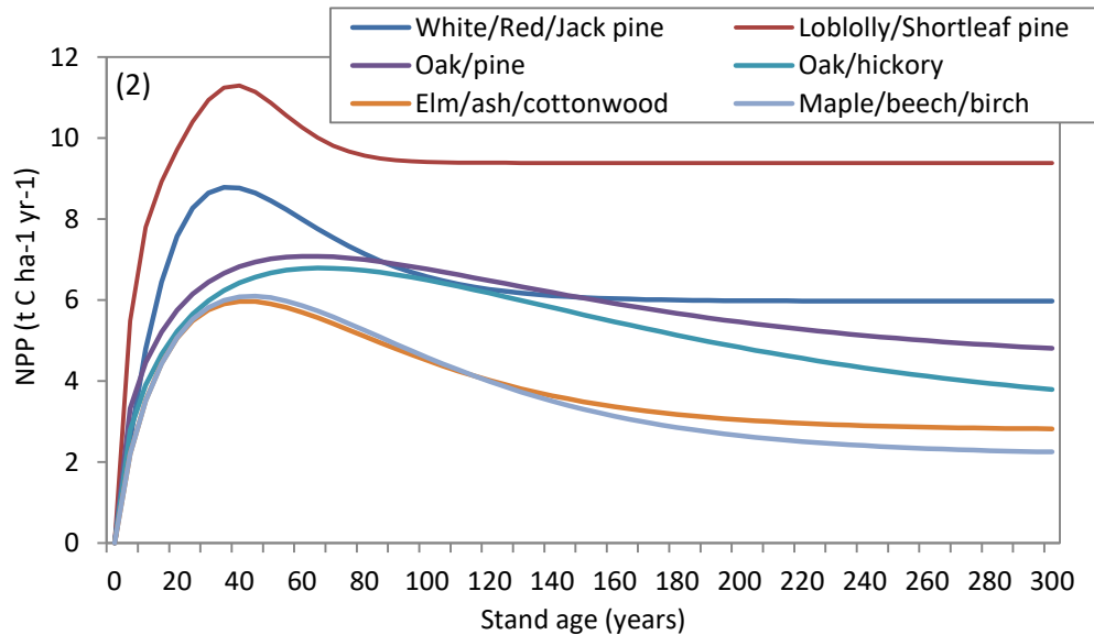
Figure 4.2. Relationship between net primary productivity (NPP) and stand age for each forest type in the Mark Twain National Forest. The Loblolly/shortleaf curve was applied to the Other Eastern Softwoods forest type.
