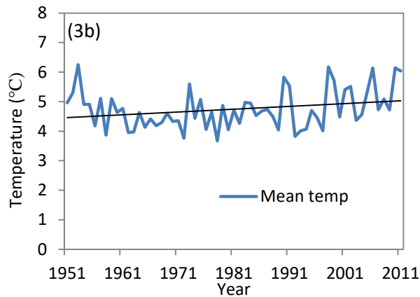
Figure 4.3. (a) Total annual precipitation (cm), (b) average annual temperature (°C), and (c) total annual nitrogen deposition from 1951-2011 in the Green Mountain and Finger Lakes National Forests. Linear trend lines shown in black.
