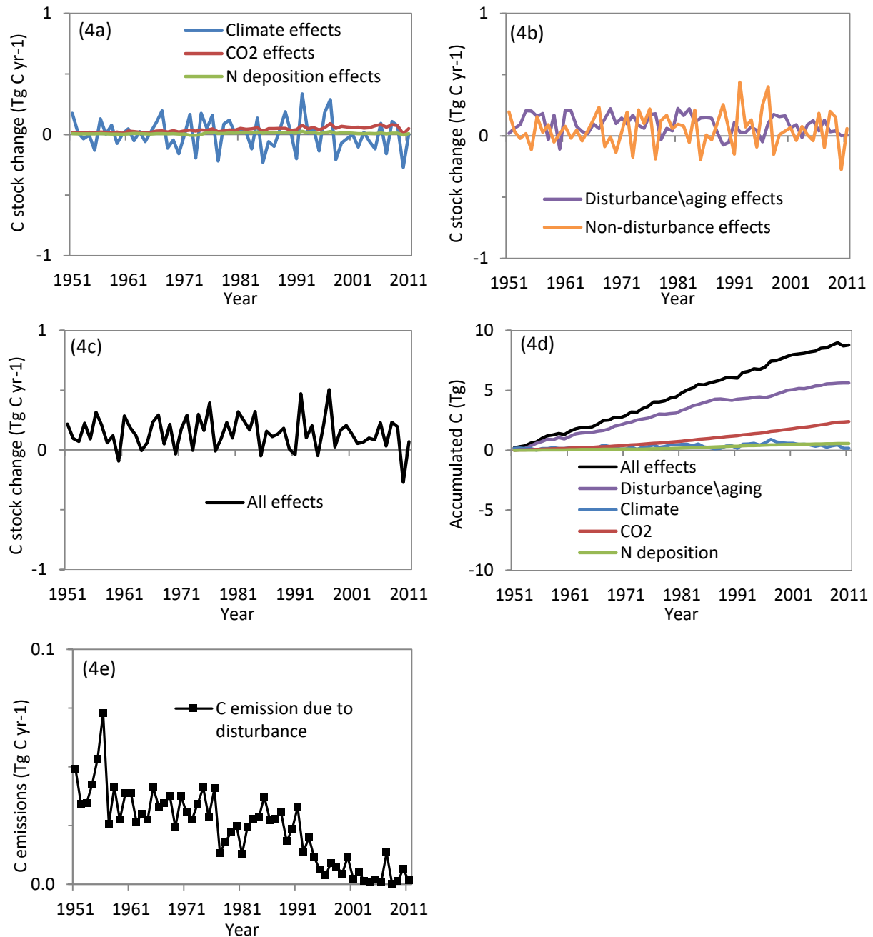
Figure 4.4. Changes in carbon stocks in the Wayne National Forest due to: (a) individual non-disturbance factors alone including climate variability, atmospheric CO 2 concentration, and nitrogen deposition; (b) all disturbance factors such as fire, harvest, and insects, as well as regrowth and aging and the sum of all non-disturbance factors combined; and (c) all factors combined which is the sum of disturbance\aging and non-disturbance effects; (d) Accumulated C due to individual disturbance\aging and non-disturbance factors and all factors combined from 1950-2011 excluding C accumulated pre-1950; and (e) C emissions due to disturbance events only. Positive values in Figures 4.4 a-c represent C sinks from the atmosphere or enhancement effects, whereas negative values represent C sources to the atmosphere, or detracting effects.
