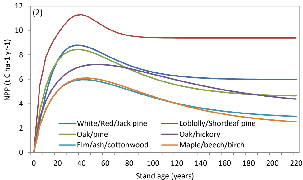
Figure 4.2. Relationship between net primary productivity (NPP) and stand age for each forest type in the Hoosier National Forest.
