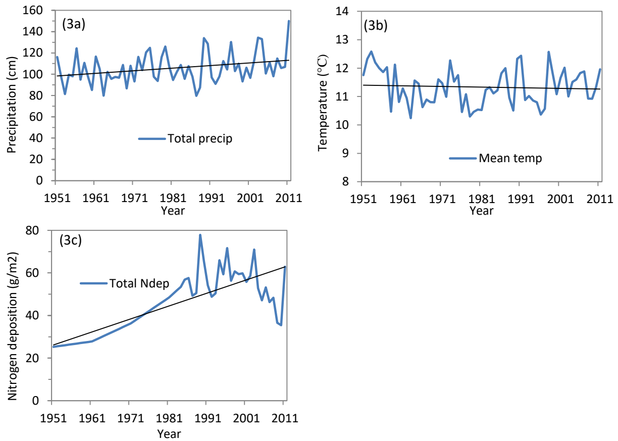
Figure 4.3. (a) Total annual precipitation (cm), (b) average annual temperature (°C), and (c) total annual nitrogen deposition from 1951-2011 in the Wayne National Forest. Linear trend lines shown in black.
