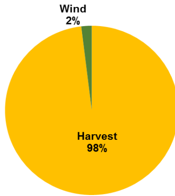
Effect of Different Disturbances, 1990-2011, on Carbon Storage in Green Mountain and Finger Lakes National Forests
