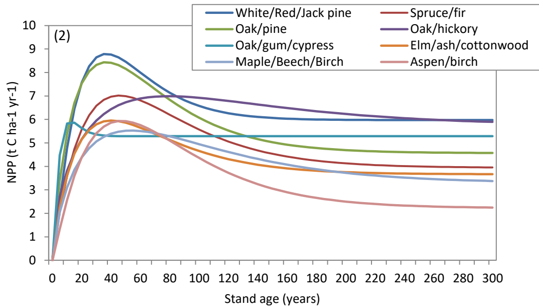
Figure 4.2. Relationship between net primary productivity (NPP) and stand age for each forest type in the White Mountain National Forest.
