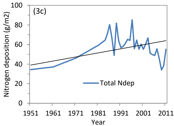
Figure 4.3. (a) Total annual precipitation (cm), (b) average annual temperature (°C), and (c) total annual nitrogen deposition from 1951-2011 in the Monongahela National Forest. Linear trend lines shown in black.
