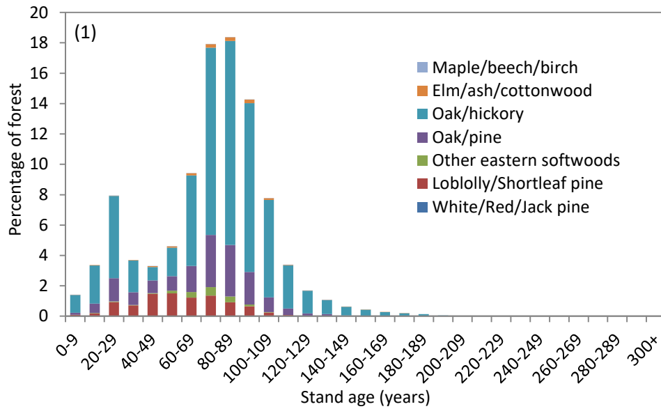
Figure 4.1. Age class distribution in 2011 in the Mark Twain National Forest displaying the percentage of forested area of each forest type in 10-year age classes. Forest types are symbolized by stacked, colored bars that also correspond to the forest types in Figure 2 below.
