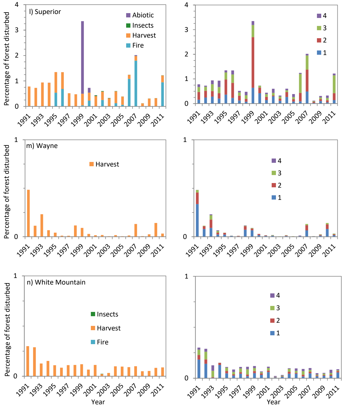
Figure 1.1. Annual rates of disturbance in the Eastern Region, mapped using visual interpretation of several independent datasets and summarized as the percentage of the forested area disturbed from 1991 through 2011 by (a) disturbance types including fire, harvests, insects, and abiotic; and b) magnitude classes, characterized by percentage change in canopy cover (CC) and categorized as follows: (1) 0 to 25 percent CC, (2) 25 to 50 percent CC, (3) 50 to 75 percent CC, and (4) 75 to 100 percent CC.
