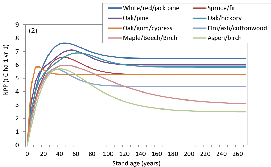
Figure 4.2. Relationship between net primary productivity (NPP) and stand age for each forest type in the Hiawatha National Forest.
