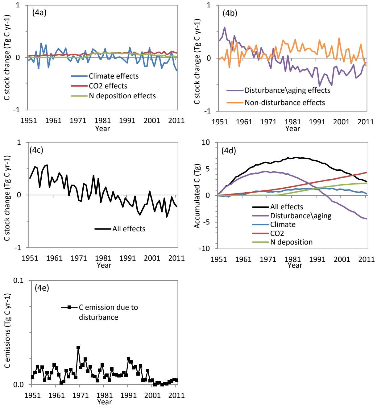
Figure 4.4. Changes in carbon stocks in the Green Mountain and Finger Lakes National Forests due to: (a) individual non-disturbance factors alone including climate variability, atmospheric CO 2 concentration, and nitrogen deposition; (b) all disturbance factors such as fire, harvest, and insects, as well as regrowth and aging and the sum of all non-disturbance factors combined; and (c) all factors combined which is the sum of disturbance\aging and non-disturbance effects; (d) Accumulated C due to individual disturbance\aging and non-disturbance factors and all factors combined from 1950-2011 excluding C accumulated pre-1950; and (e) C emissions due to disturbance events only. Positive values in Figures 4.4 a-c represent C sinks from the atmosphere or enhancement effects, whereas negative values represent C sources to the atmosphere, or detracting effects.
