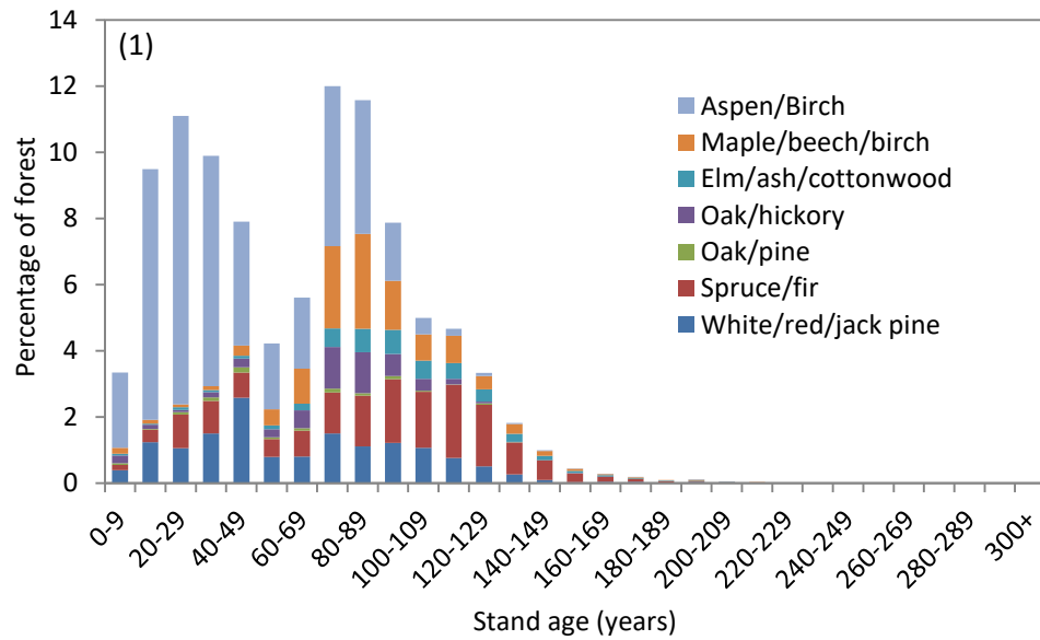
Figure 4.1. Age class distribution in 2011 in the Chippewa National Forest displaying the percentage of forested area of each forest type in 10-year age classes. Forest types are symbolized by stacked, colored bars that also correspond to the forest types in Figure 2 below.
