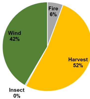
Effect of Different Disturbances, 1990-2011, on Carbon Storage in Monongahela National Forest
