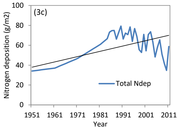
Figure 4.3. (a) Total annual precipitation (cm), (b) average annual temperature (°C), and (c) total annual nitrogen deposition from 1951-2011 in the Allegheny National Forest. Linear trend lines shown in black.
