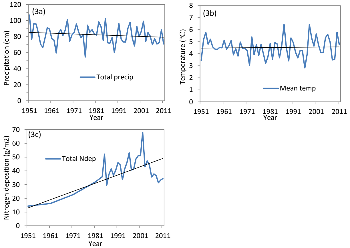
Figure 4.3. (a) Total annual precipitation (cm), (b) average annual temperature (°C), and (c) total annual nitrogen deposition from 1951-2011 in the Ottawa National Forest. Linear trend lines shown in black.
