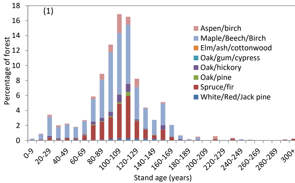
Figure 4.1. Age class distribution in 2011 in the White Mountain National Forest displaying the percentage of forested area of each forest type in 10-year age classes. Forest types are symbolized by stacked, colored bars that also correspond to the forest types in Figure 2 below.
