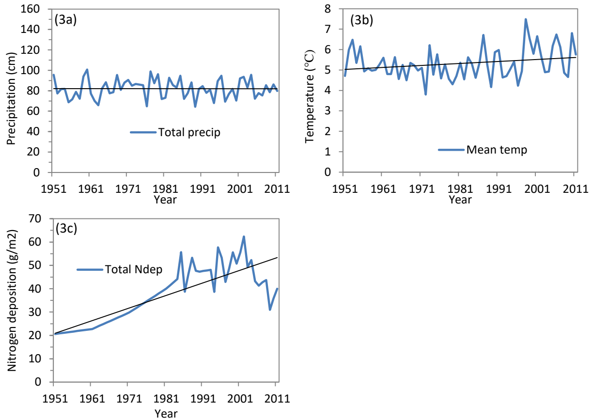
Figure 4.3. (a) Total annual precipitation (cm), (b) average annual temperature (°C), and (c) total annual nitrogen deposition from 1951-2011 in the Hiawatha National Forest. Linear trend lines shown in black.
