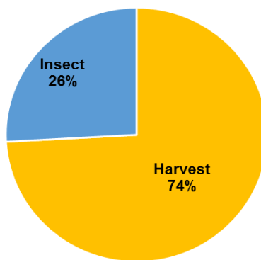
Effect of Different Disturbances, 1990-2011, on Carbon Storage in Hoosier National Forest
