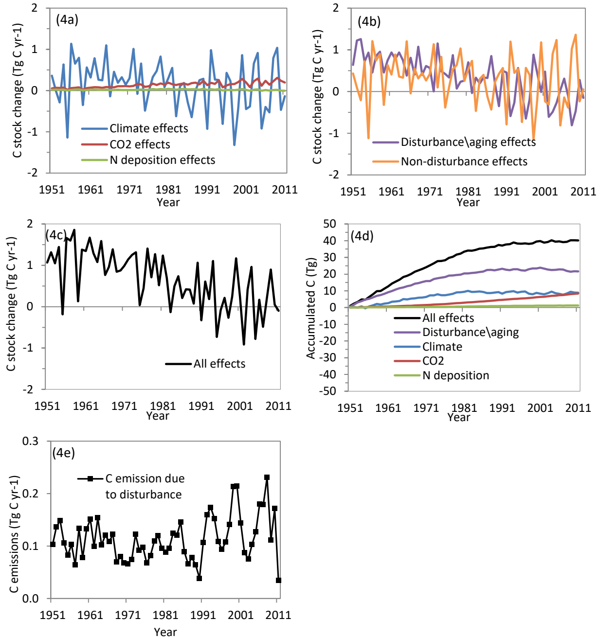
Figure 4.4. Changes in carbon stocks in the Hiawatha National Forest due to: (a) individual non-disturbance factors alone including climate variability, atmospheric CO 2 concentration, and nitrogen deposition; (b) all disturbance factors such as fire, harvest, and insects, as well as regrowth and aging and the sum of all non-disturbance factors combined; and (c) all factors combined which is the sum of disturbance\aging and non-disturbance effects; (d) Accumulated C due to individual disturbance\aging and non-disturbance factors and all factors combined from 1950-2011 excluding C accumulated pre-1950; and (e) C emissions due to disturbance events only. Positive values in Figures 4.4 a-c represent C sinks from the atmosphere or enhancement effects, whereas negative values represent C sources to the atmosphere, or detracting effects.
