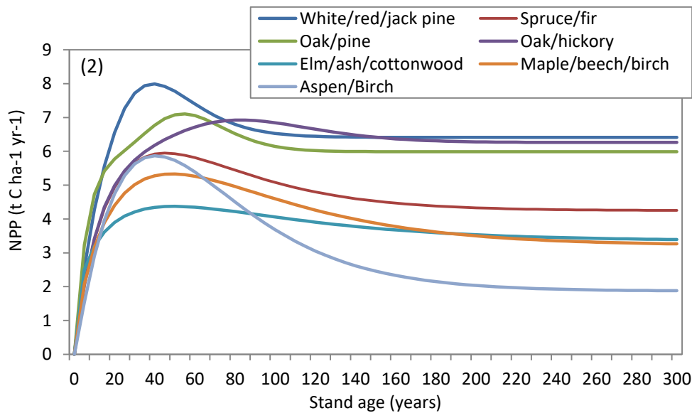
Figure 4.2. Relationship between net primary productivity (NPP) and stand age for each forest type in the Chippewa National Forest.
