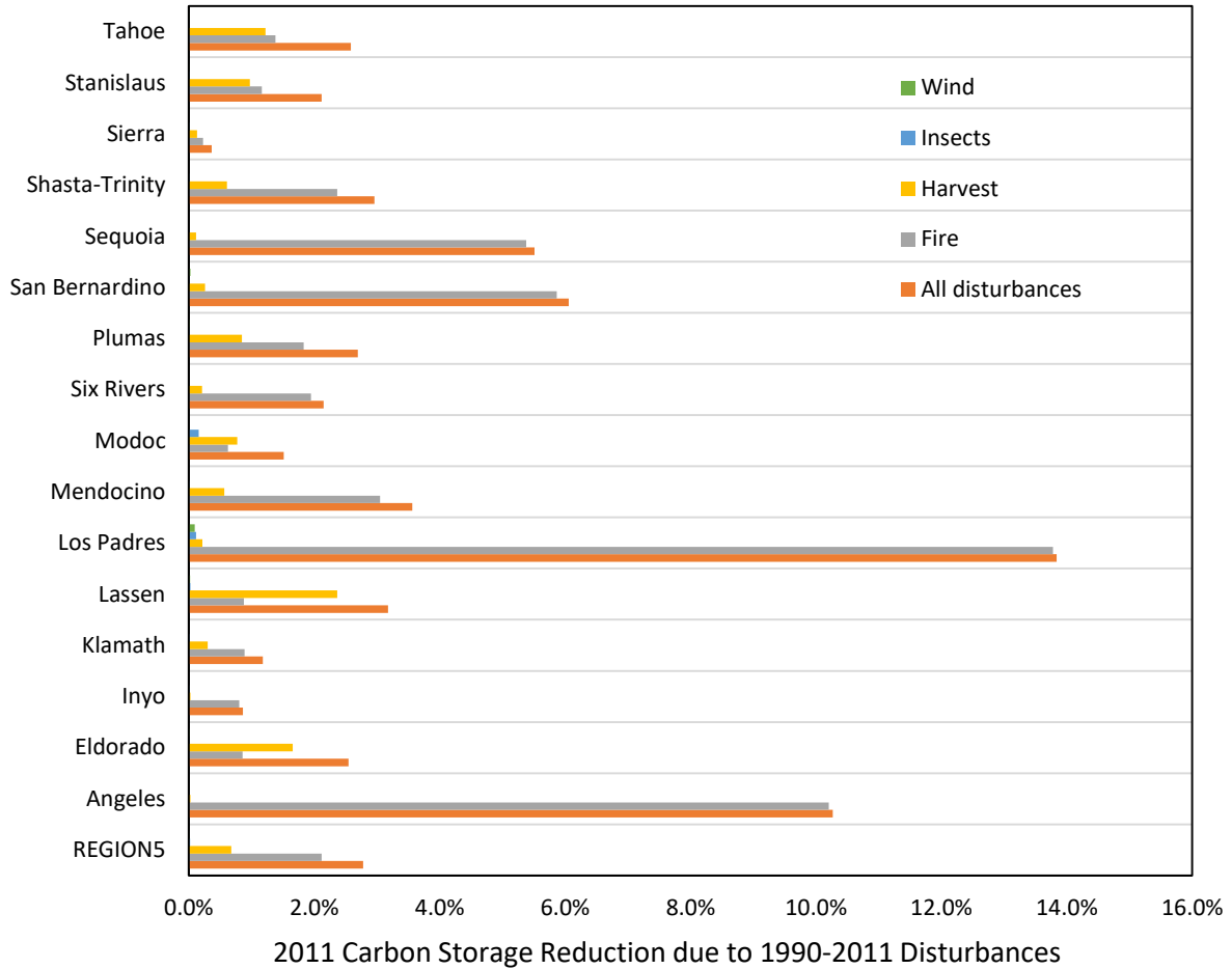
Figure 3.1. The degree to which 2011 carbon storage on each national forest was reduced by disturbances occurring from 1990 to 2011 in the Pacific Southwest Region. Results were derived through the ForCaMF system (Healey et al., 2014), and the baseline assessment of carbon stocks (USDA Forest Service 2015b). Percent reduction represents how much non-soil carbon was lost from the baseline forest inventory carbon stock estimates. “Wind” is a combination of ice and wind storms and was labelled “abiotic” in Figure 1.
