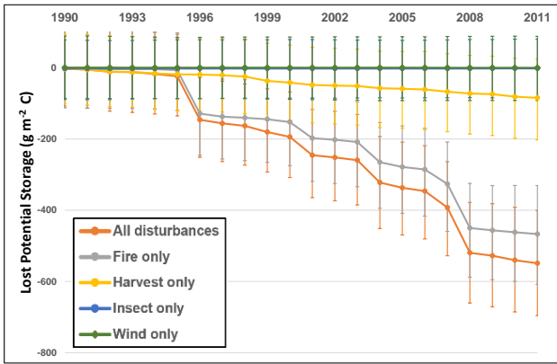
2.1g) Mendocino National Forest
