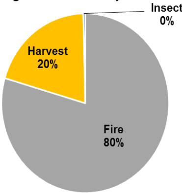
Effect of Different Disturbances, 1990-2011, on Carbon Storage in Shasta-Trinity National Forest
