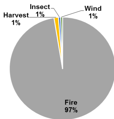
Effect of Different Disturbances, 1990-2011, on Carbon Storage in Los Padres National Forest
