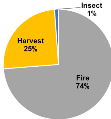
Effect of Different Disturbances, 1990-2011, on Carbon Storage in Klamath National Forest
