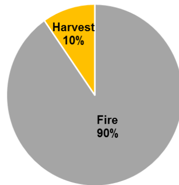
Effect of Different Disturbances, 1990-2011, on Carbon Storage in Six Rivers National Forest
