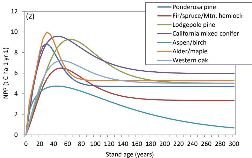
Figure 4.2. Relationship between net primary productivity (NPP) and stand age for each forest type group.
