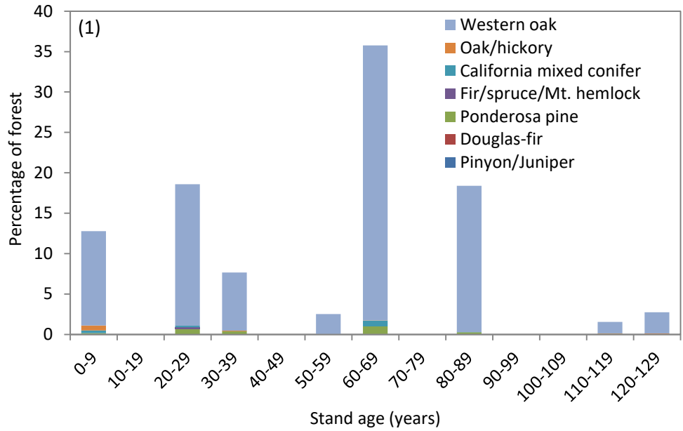
Figure 4.1. Age class distribution in 2010 displaying the percentage of forested area of each forest type in 10-year age classes. Forest types are symbolized by stacked, colored bars that also correspond to the forest types in Figure 2 below.
