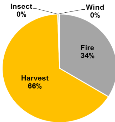
Effect of Different Disturbances, 1990-2011, on Carbon Storage in Eldorado National Forest
