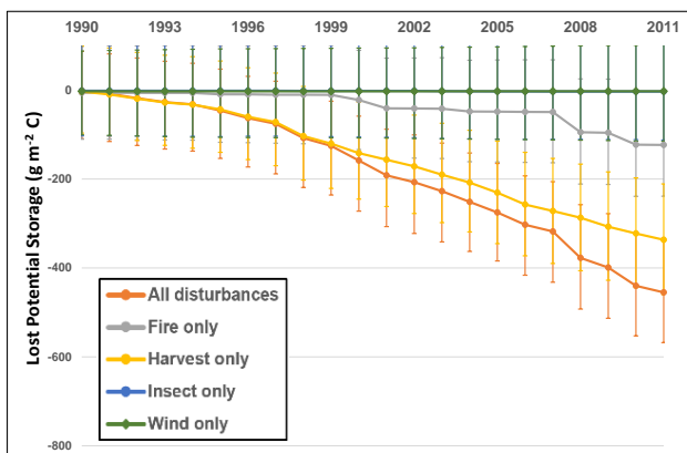
2.1e) Lassen National Forest
