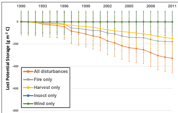
Figure 2.1. The impact of different kinds of disturbance, occurring from 1990 through 2011, on carbon (C) stores in the Pacific Southwest Region. The difference in storage for each year is shown between an “undisturbed” scenario and a scenario that includes only observed amounts of the specified type of disturbance. Error bars represent a 95-percent confidence interval; 100 g/m 2 equals 1 metric tonne (or Mg)/ha.
