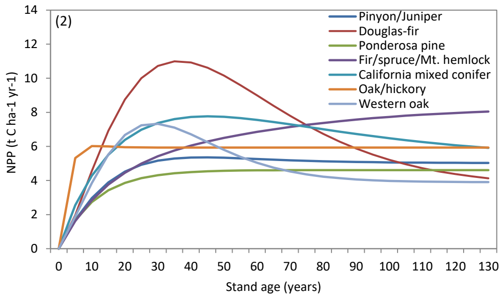
Figure 4.2. Relationship between net primary productivity (NPP) and stand age for each forest type group.
