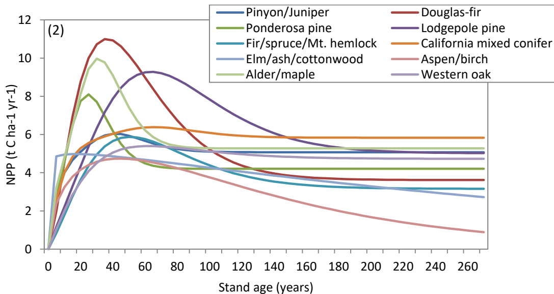
Figure 4.2. Relationship between net primary productivity (NPP) and stand age for each forest type group.
