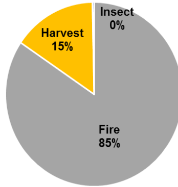
Effect of Different Disturbances, 1990-2011, on Carbon Storage in Mendocino National Forest
