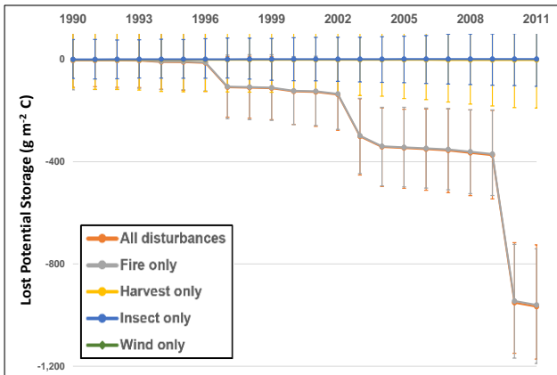
2.1a) Angeles National Forest
