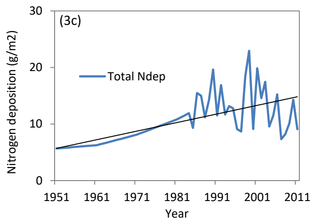
Figure 4.3. (a) Total annual precipitation (cm), (b) average annual temperature ( ^{\circ}\text{C} ), and (c) total annual nitrogen deposition from 1951-2011. Linear trend lines shown in black.
