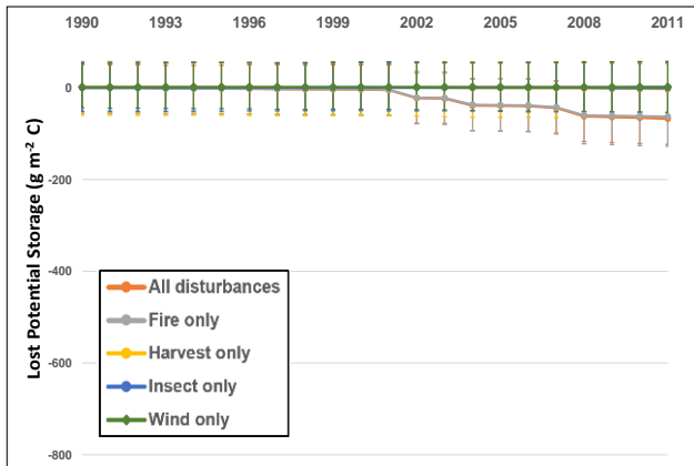
2.1c) Inyo National Forest
