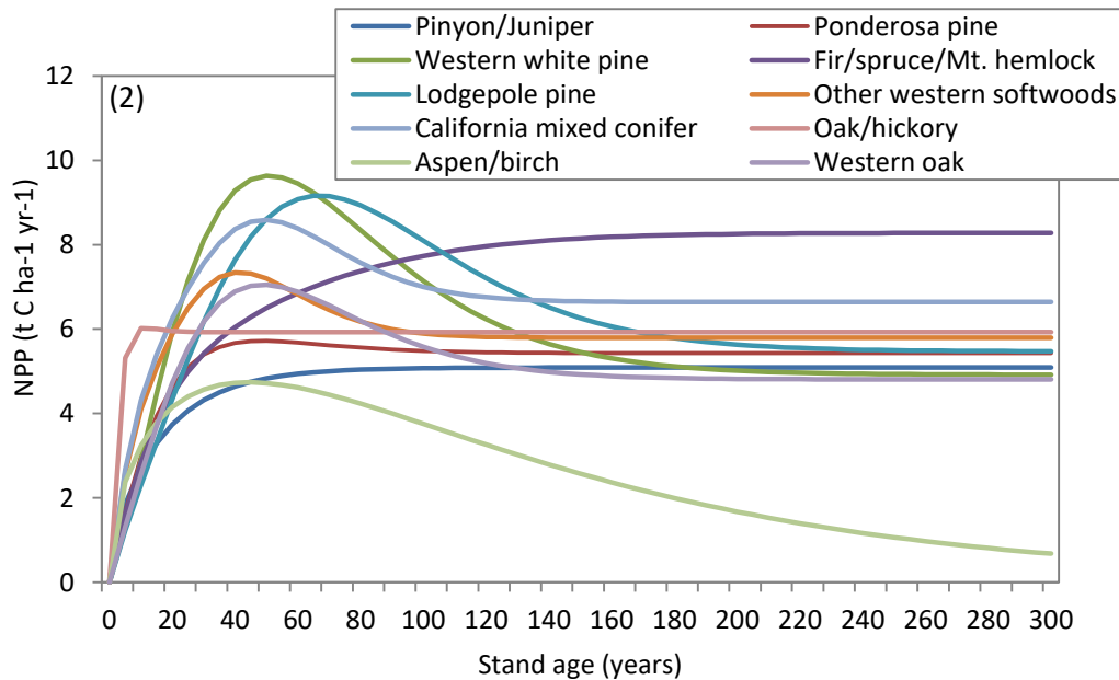
Figure 4.2. Relationship between net primary productivity (NPP) and stand age for each forest type group.
