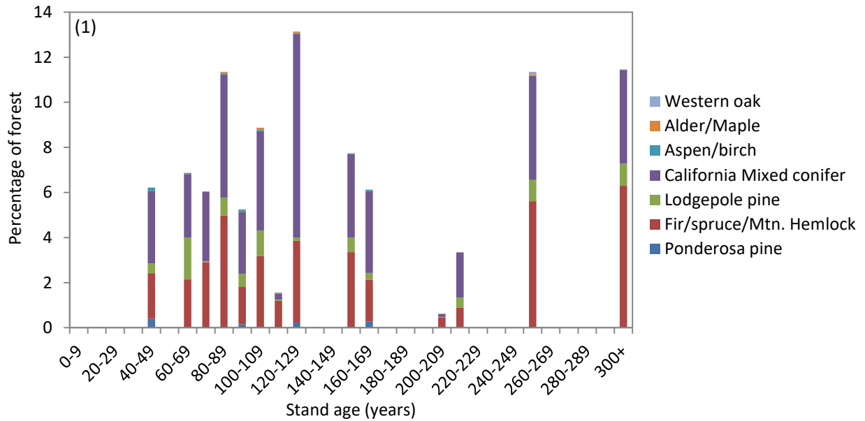
Figure 4.1. Age class distribution in 2010 displaying the percentage of forested area of each forest type group in 10-year age classes. Forest type groups are symbolized by stacked, colored bars that also correspond to the forest types in Figure 2 below.
