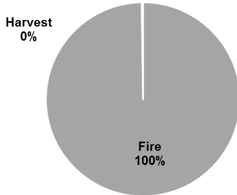
Effect of Different Disturbances, 1990-2011, on Carbon Storage in Angeles National Forest
