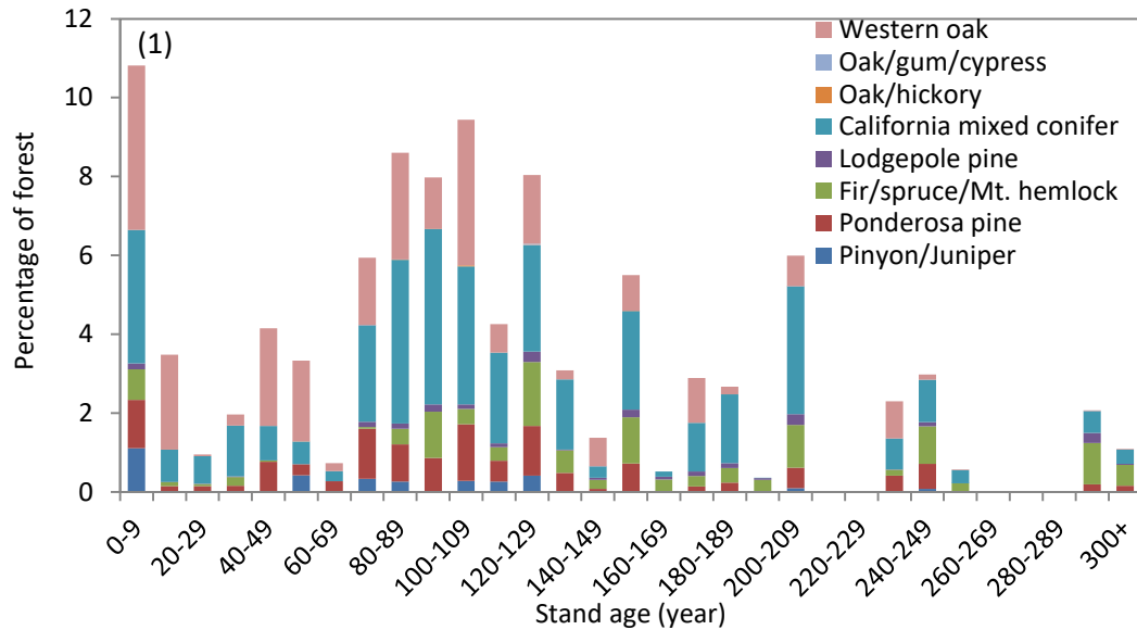
Figure 4.1. Age class distribution in 2010 displaying the percentage of forested area of each forest type group in 10-year age classes. Forest type groups are symbolized by stacked, colored bars that also correspond to the forest types in Figure 2 below.
