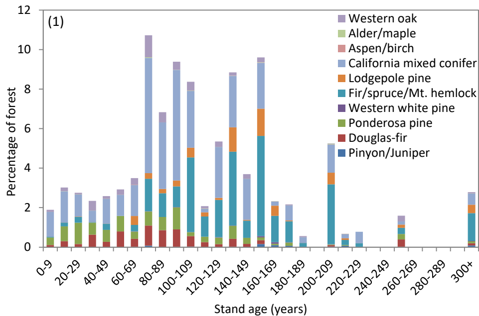
Figure 4.1. Age class distribution in 2010 displaying the percentage of forested area of each forest type group in 10-year age classes. Forest type groups are symbolized by stacked, colored bars that also correspond to the forest types in Figure 2 below.
