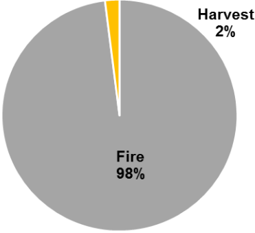
Effect of Different Disturbances, 1990-2011, on Carbon Storage in Sequoia National Forest
