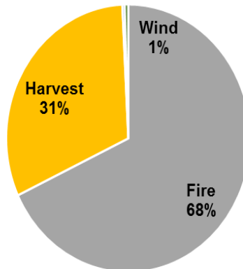
Effect of Different Disturbances, 1990-2011, on Carbon Storage in Plumas National Forest
