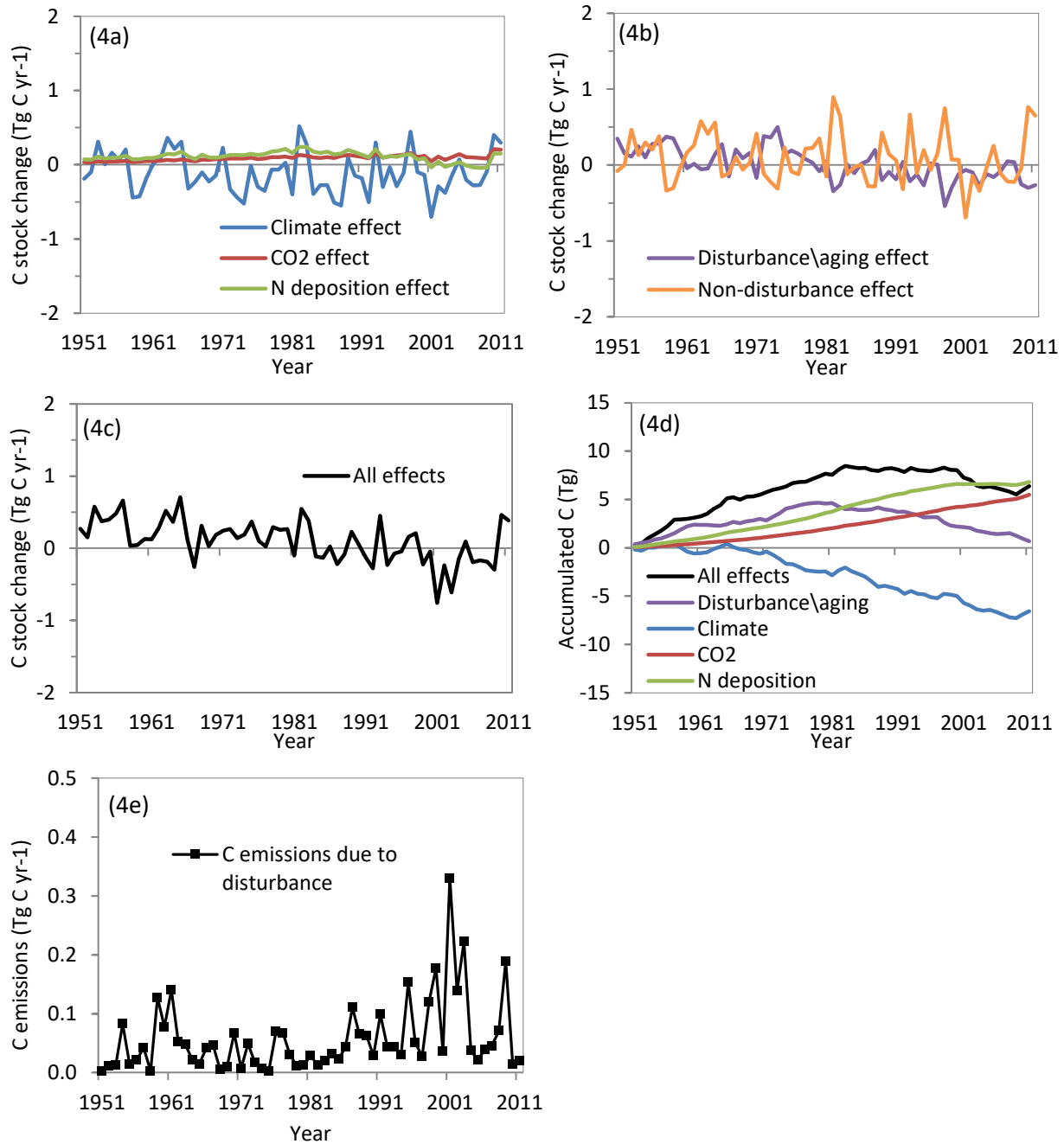
Figure 4.4. Changes in carbon stocks due to: (a) individual non-disturbance factors alone including climate variability, atmospheric CO 2 concentration, and nitrogen deposition; (b) all disturbance factors such as fire, harvest, and insects, as well as regrowth and aging and the sum of all non-disturbance factors combined; and (c) all factors combined which is the sum of disturbance/aging and non-disturbance effects; (d) Accumulated C due to individual disturbance/aging and non-disturbance factors and all factors combined from 1950-2010 excluding C accumulated pre-1950; and (e) C emissions due to disturbance events only. Positive values in Figures 4a-c represent C sinks from the atmosphere or enhancement effects, whereas negative values represent C sources to the atmosphere, or detracting effects.
