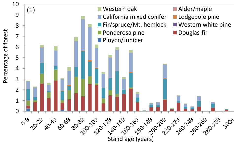
Figure 4.1. Age class distribution in 2010 displaying the percentage of forested area of each forest type group in 10-year age classes. Forest type groups are symbolized by stacked, colored bars that also correspond to the forest types in Figure 2 below.
