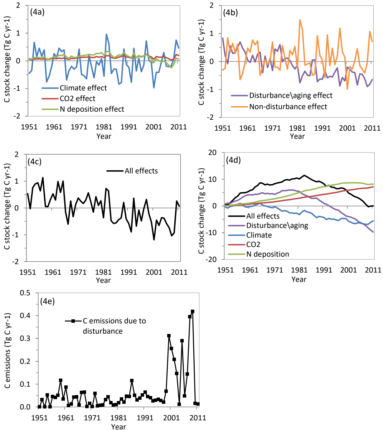
Figure 4.4. Changes in carbon stocks due to: (a) individual non-disturbance factors alone including climate variability, atmospheric CO 2 concentration, and nitrogen deposition; (b) all disturbance factors such as fire, harvest, and insects, as well as regrowth and aging and the sum of all non-disturbance factors combined; and (c) all factors combined which is the sum of disturbance/aging and non-disturbance effects; (d) Accumulated C due to individual disturbance/aging and non-disturbance factors and all factors combined from 1950-2010 excluding C accumulated pre-1950; and (e) C emissions due to disturbance events only. Positive values in Figures 4a-c represent C sinks from the atmosphere or enhancement effects, whereas negative values represent C sources to the atmosphere, or detracting effects.
