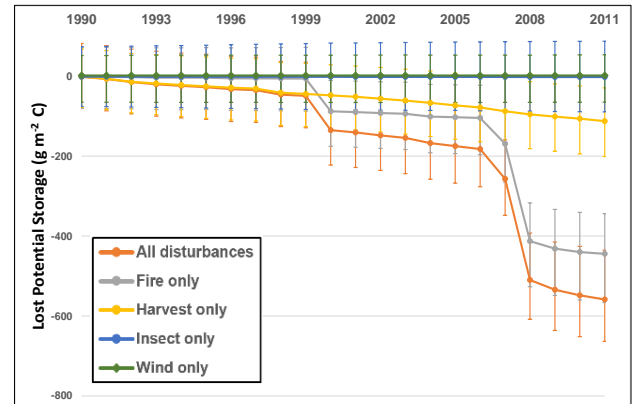
2.1l) Shasta-Trinity National Forest
