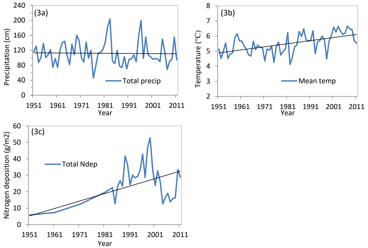
Figure 4.3. (a) Total annual precipitation (cm), (b) average annual temperature (°C), and (c) total annual nitrogen deposition from 1951-2011. Linear trend lines shown in black.
