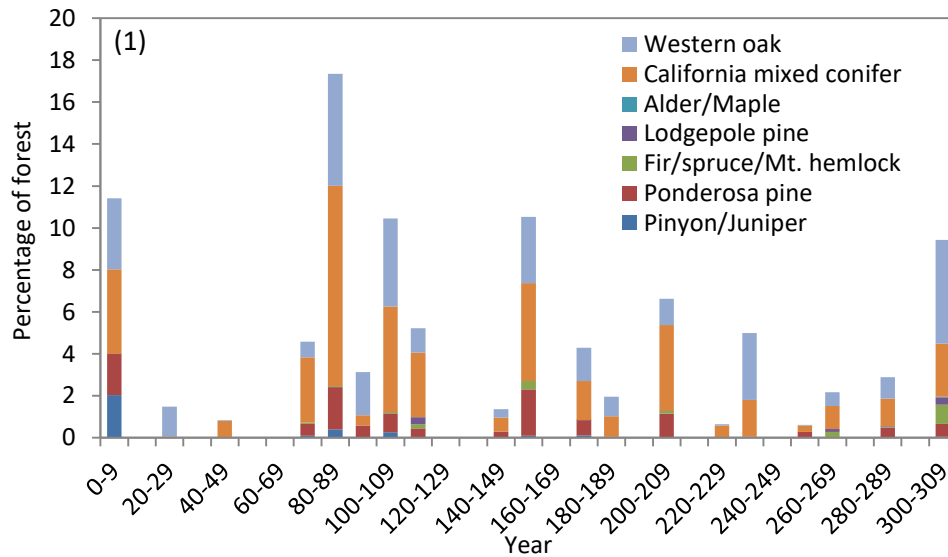
Figure 4.1. Age class distribution in 2010 displaying the percentage of forested area of each forest type group in 10-year age classes. Forest type groups are symbolized by stacked, colored bars that also correspond to the forest types in Figure 2 below.
