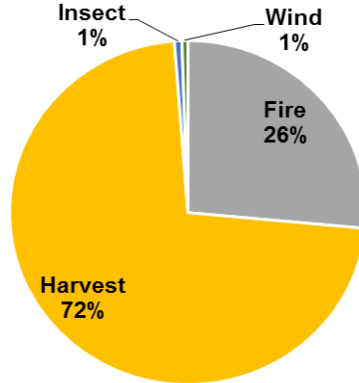
Effect of Different Disturbances, 1990-2011, on Carbon Storage in Lassen National Forest
