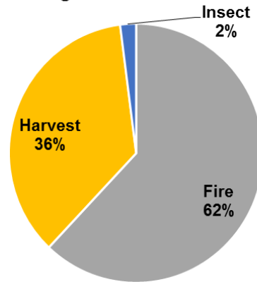
Effect of Different Disturbances, 1990-2011, on Carbon Storage in Sierra National Forest
