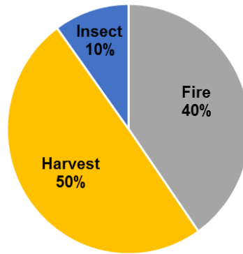
Effect of Different Disturbances, 1990-2011, on Carbon Storage in Modoc National Forest
