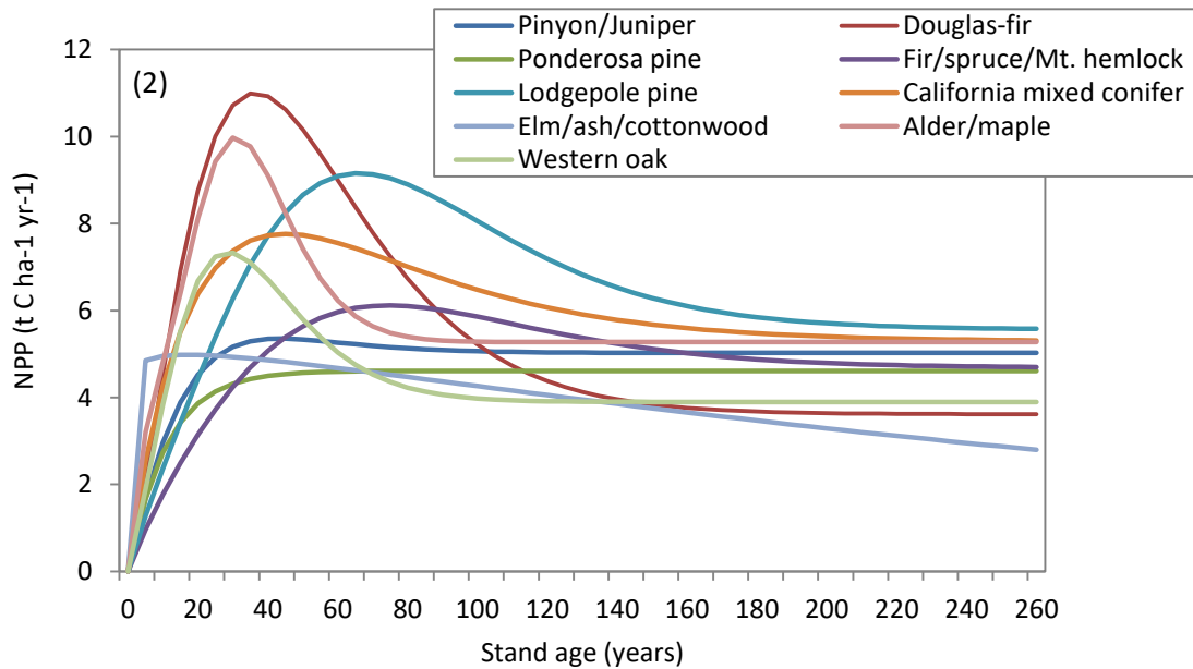
Figure 4.2. Relationship between net primary productivity (NPP) and stand age for each forest type group.
