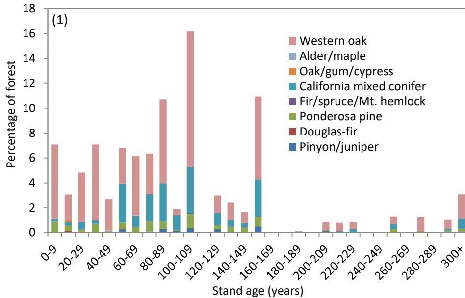
Figure 4.1. Age class distribution in 2010 displaying the percentage of forested area of each forest type group in 10-year age classes. Forest type groups are symbolized by stacked, colored bars that also correspond to the forest types in Figure 2 below.
