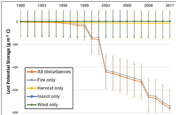
2.1k) Sequoia National Forest
