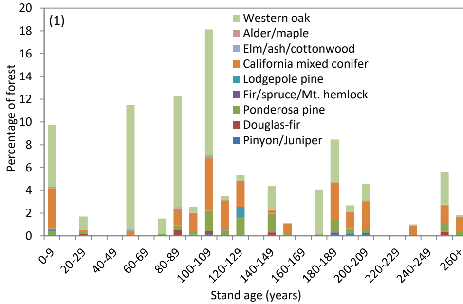
Figure 4.1. Age class distribution in 2010 displaying the percentage of forested area of each forest type in 10-year age classes. Forest types are symbolized by stacked, colored bars that also correspond to the forest types in Figure 2 below.
