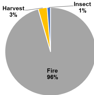
Effect of Different Disturbances, 1990-2011, on Carbon Storage in Inyo National Forest
