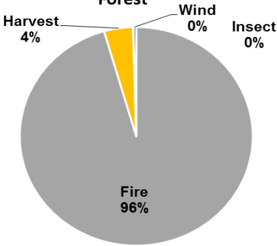
Effect of Different Disturbances, 1990-2011, on Carbon Storage in San Bernardino National Forest
