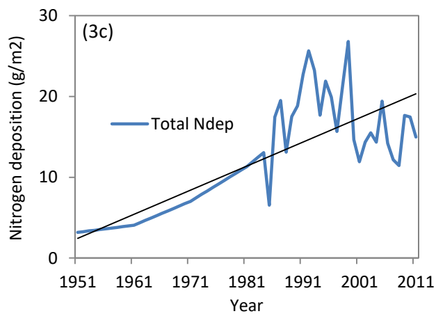
Figure 4.3. (a) Total annual precipitation (cm), (b) average annual temperature (°C), and (c) total annual nitrogen deposition from 1951-2011. Linear trend lines shown in black.
