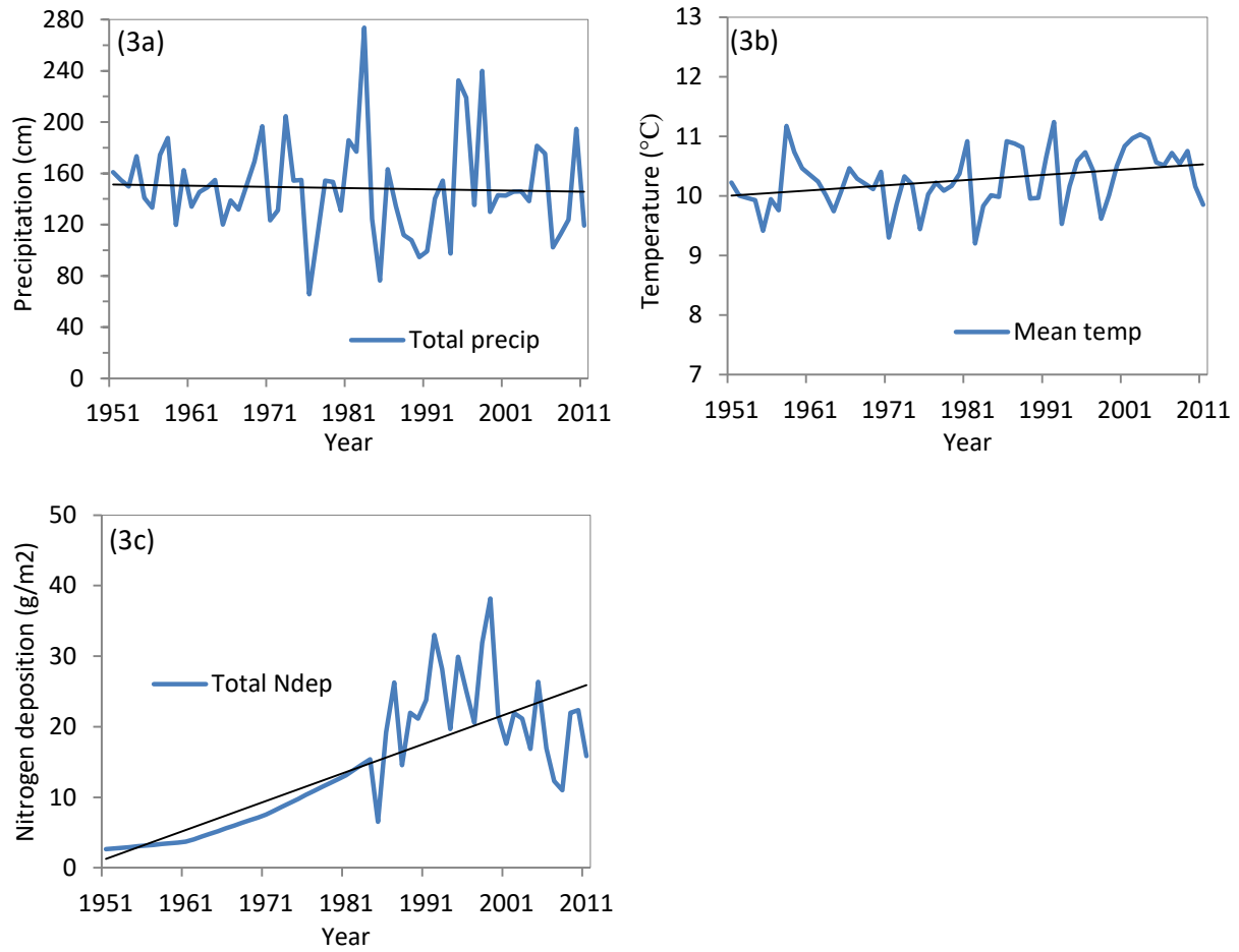
Figure 4.3. (a) Total annual precipitation (cm), (b) average annual temperature (°C), and (c) total annual nitrogen deposition from 1951-2011. Linear trend lines shown in black.
