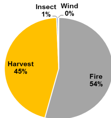
Effect of Different Disturbances, 1990-2011, on Carbon Storage in Stanislaus National Forest
