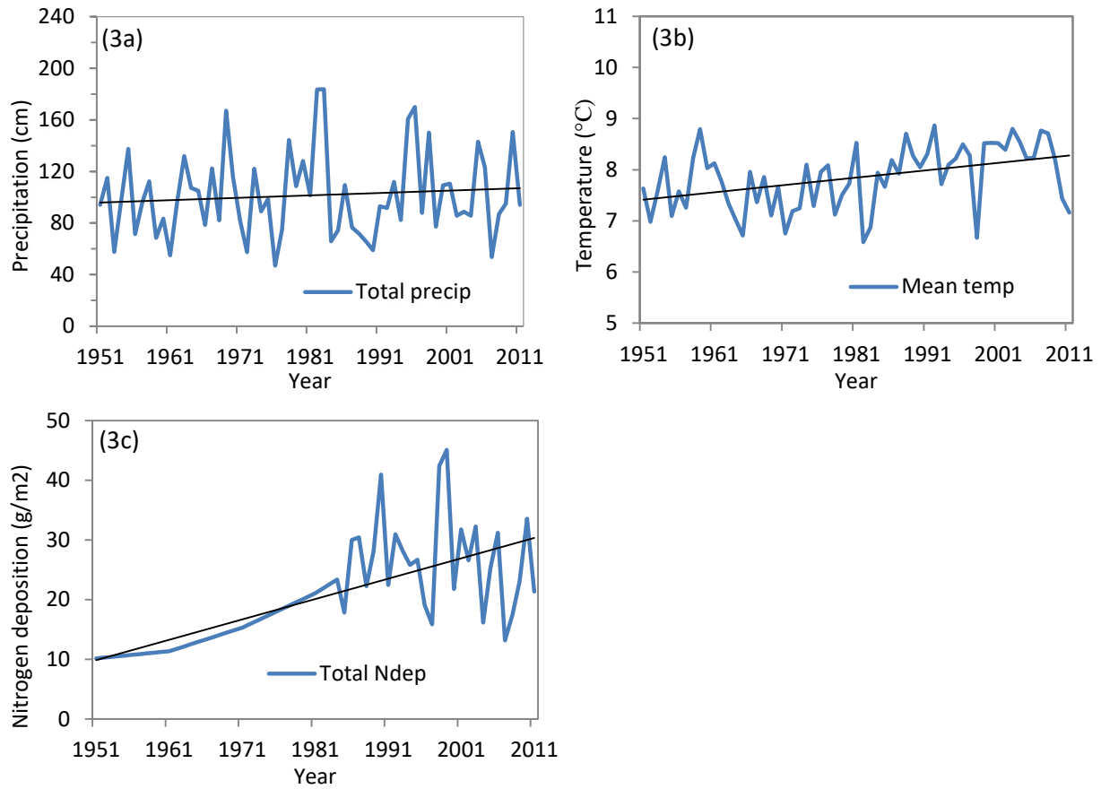
Figure 4.3. (a) Total annual precipitation (cm), (b) average annual temperature (°C), and (c) total annual nitrogen deposition from 1951-2011. Linear trend lines shown in black.
