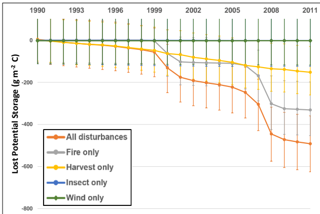
2.1k) Sequoia National Forest
