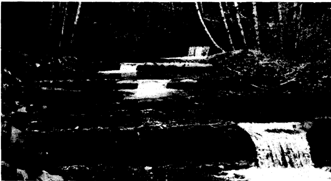
Figure 3.--Log weirs used to correct a culvert entry barrier.
