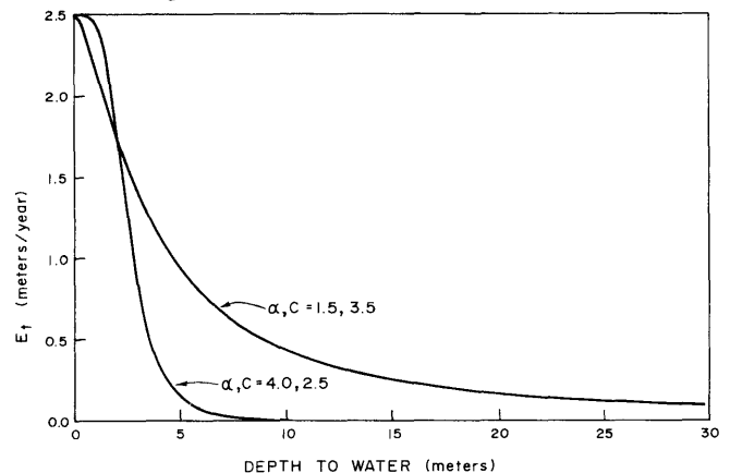
Figure 3.-- E_t/D Models.
