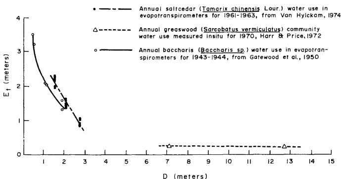
Figure 2.-- E_t/D data.
