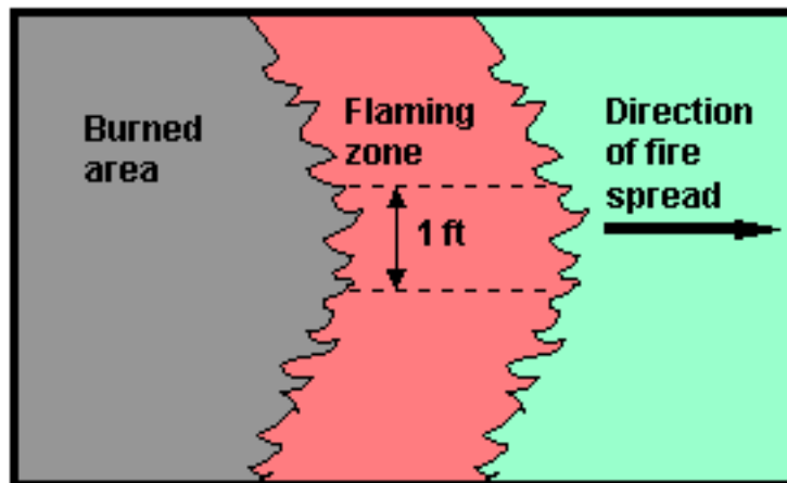
Figure 3—Fireline intensity.
