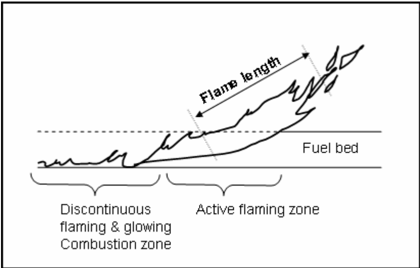
Figure 2—Flame length.
