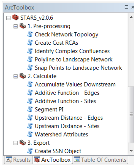
Figure 1. Spatial Tools for the Analysis of River Systems (STARS) geoprocessing toolbox for ArcGIS version 10.5.
