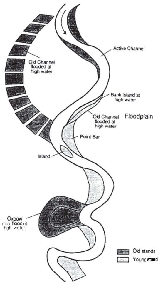
Figure 9. Zones of cottonwood and other riparian species establishment along an unmodified river (Crawford et al, 1993).
