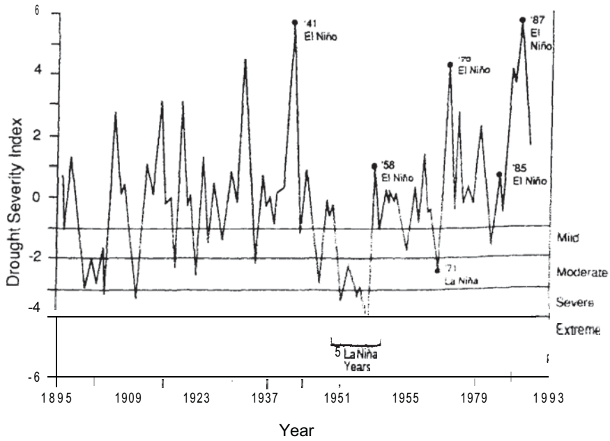
Figure 6a. Drought severity index 1895 through 1988 and El Nina and La Nina events over the past 50 years for the Middle Rio Grande Valley (after U.S. Army Corps of Engineers, 1991).
