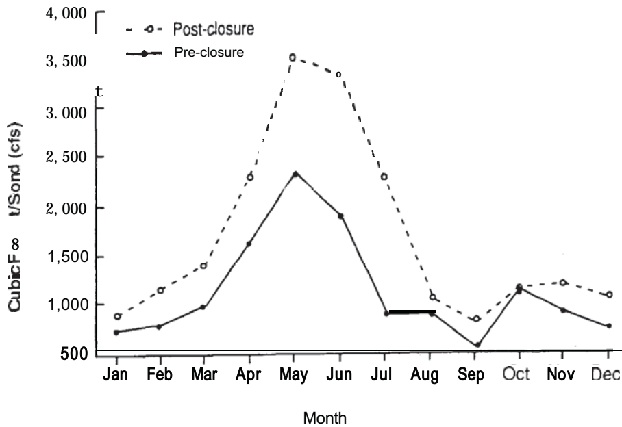
Figure 6b. Fifteen-year average of Rio Grande monthly mean discharge for pre- and post-Cochiti Dam closure periods at San Felipe gauge (from Crawford et al, 1993).
