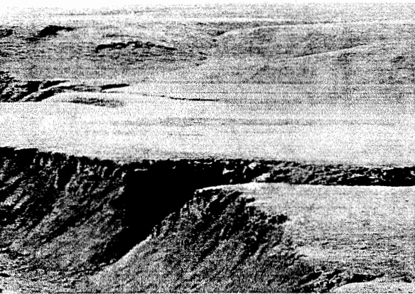
Typical degraded riparian area in the Bad River drainage. The channel is downcut and banks are near vertical walls 8-12 feet high. There is little riparian vegetation to protect streambanks against further erosion or to slow runoff and reduce transport of sediment and bed-load downstream.
