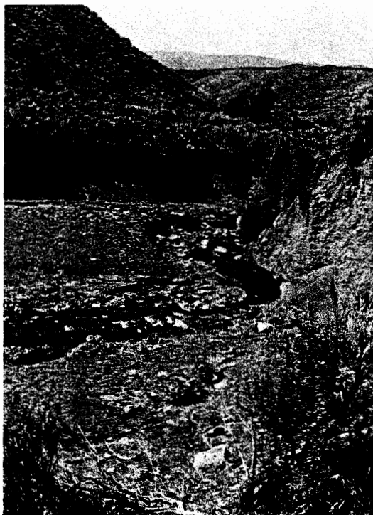
Vertically unstable stream channel.
