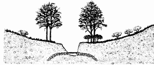
Stage 2: Rapid downcutting
