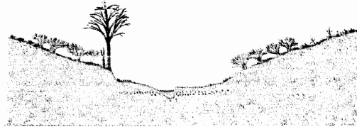
Stage 3: Channel widening and forming new floodplain
