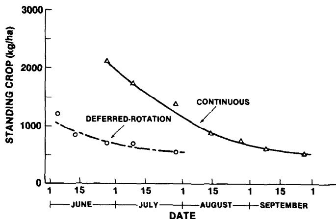
Fig. 1. Standing crop of total herbage on dry riparian meadows, 1980. Each point represents the mean of 4 sampling sites. Curves were calculated from regression equations in Table 2.
