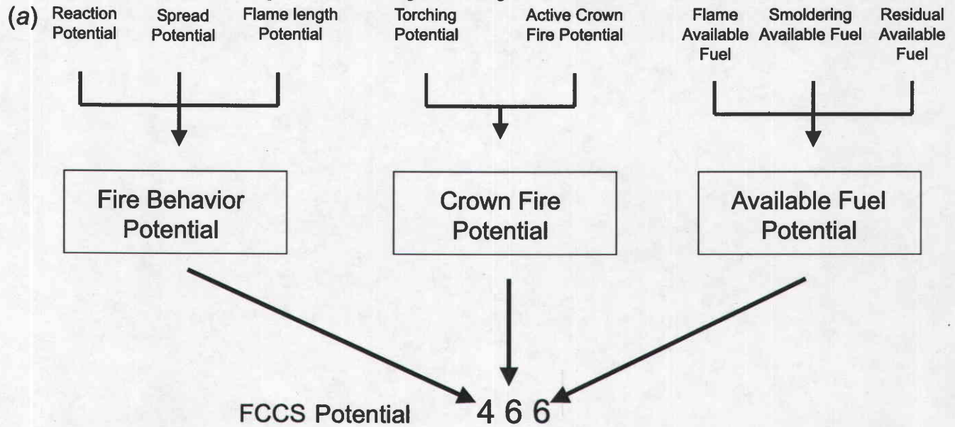
Fig. 4. (a) Fuel Characteristic Classification System (FCCS) fire potentials are a set of relative index values (0–9) that rate the intrinsic physical capacity of a fuelbed to support surface and crown fire and to consume and smolder fuels. (b) The forested area on the Eagle Creek Ranger District of the Lassen National Forest has been thinned and the fuels treated, resulting in reduced FCCS surface, crown, and available fuel potentials. (Reproduced with permission of the Eagle Lake Ranger District, Lassen National Forest, Susanville, California).
