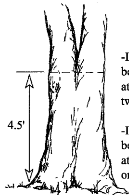
Bottleneck tree
