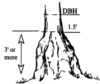
Bottleneck tree
