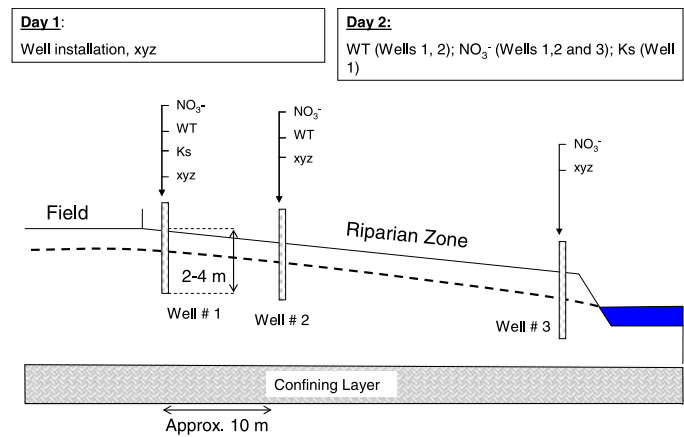
FIGURE 1. Schematic Diagram of the Field Layout and Summary of Measurements for the Simplified Method ( \text{NO}_3^- , nitrate concentration measurement; WT, water table elevation measurement; Ks, saturated soil hydraulic conductivity measurement; xyz, measurement of relative distances and elevations between wells). The dashed line indicates the water table.
