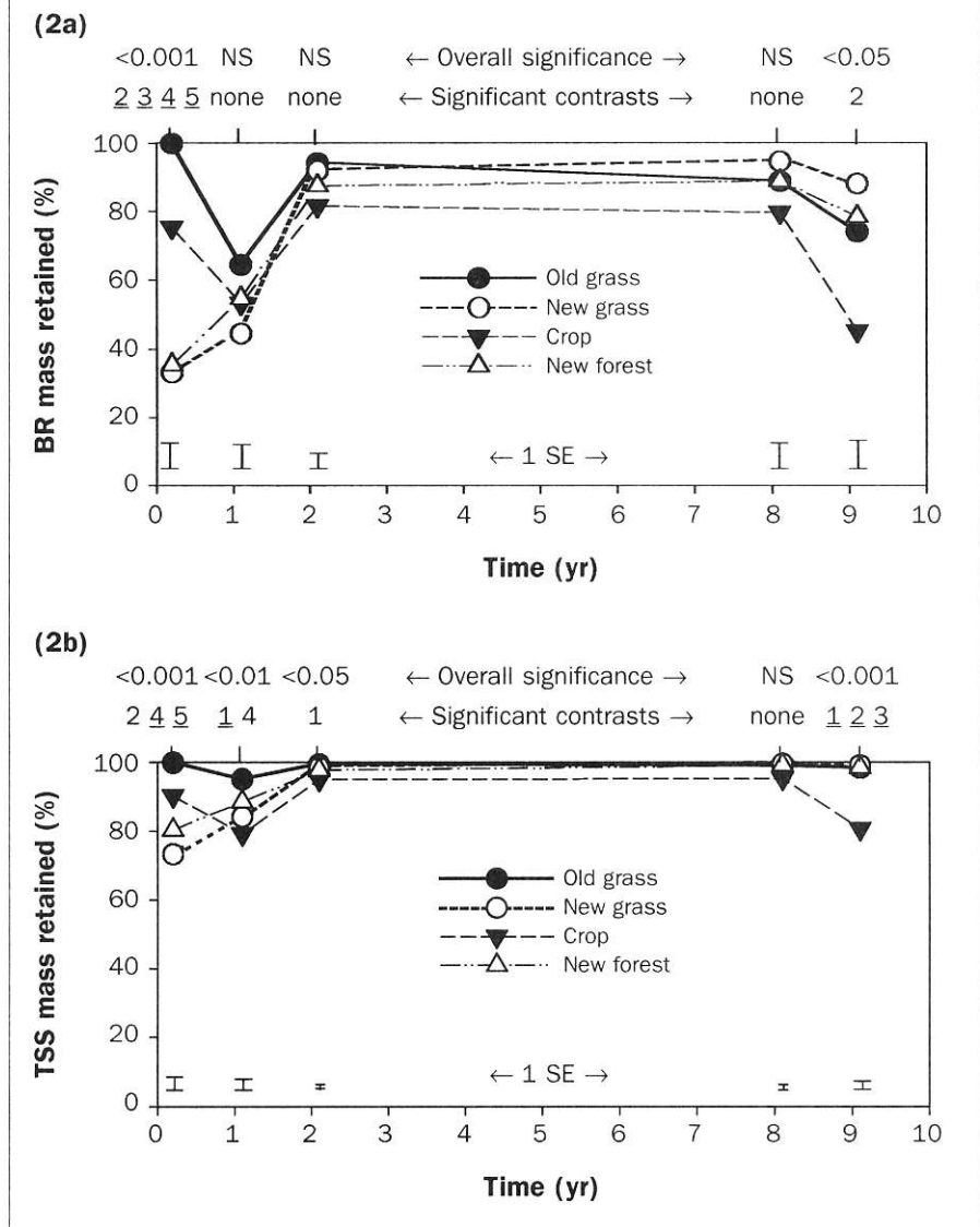
Figure 2 - a, b Average percentage of component mass from the tank source that was retained by the 7.5 m-length plots as a function of time since plot establishment: (a) Bromide or BR, (b) Total suspended solids or TSS. Also shown for each time point are: P -value of the overall F-test, significance level indicators for the individual treatment contrasts, and the pooled standard error (SE) for multiple comparisons. The numeric codes for indicating significance of individual contrasts are displayed in Table 2.
