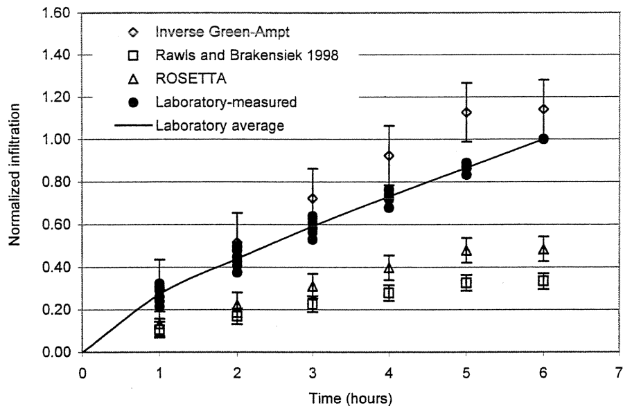
Figure 3. Normalized infiltration (cumulative) for four of the parameter estimation methods based on data from all six field sites. Bars indicate \pm standard error from the mean.
