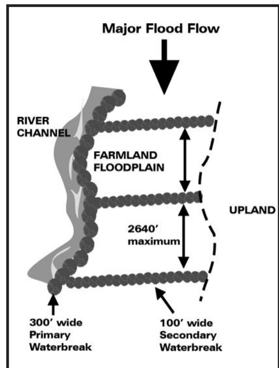
Typical waterbreak layout designed to reduce flooding damage to farmland adjacent to a large river.
