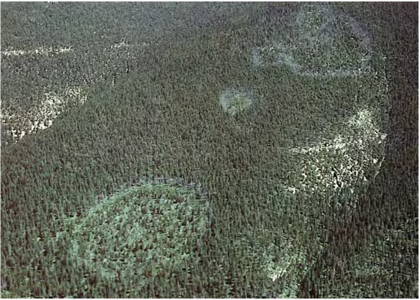
Figure 10 —Three disease centers in a virgin, mixed conifer forest in western Montana. The lowermost center covers nearly 20 acres (8 ha).
