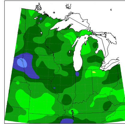
Accumulated Precipitation: Percent of Mean June 1, 2014 to August 31, 2014
