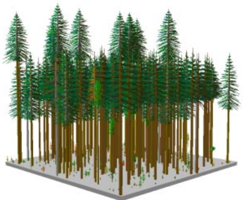
Year 2140: old forest, single stratum Canopy cover 74 percent
