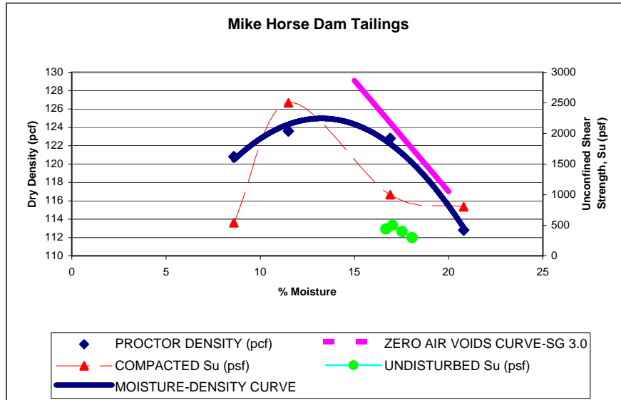
FIGURE 6-3. MOISTURE-DENSITY CURVE AND UNCONFINED SHEAR STRENGTH OF TAILINGS
