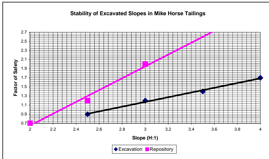
FIGURE 6-4. FACTORS OF SAFETY FOR SLOPE STABILITY
