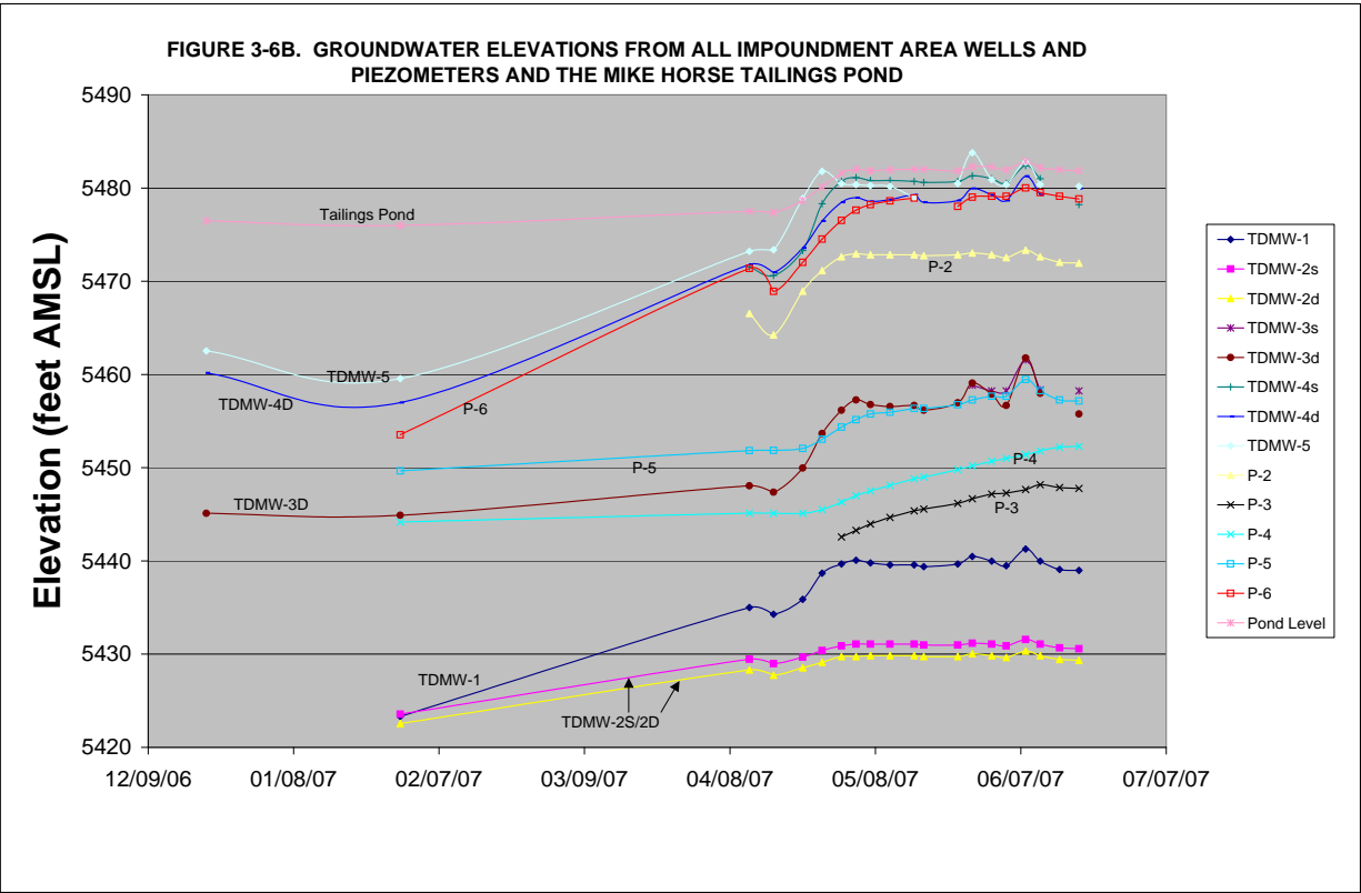
FIGURE 3-6. GROUNDWATER LEVELS IN THE MIKE HORSE TAILINGS IMPOUNDMENT AREA
