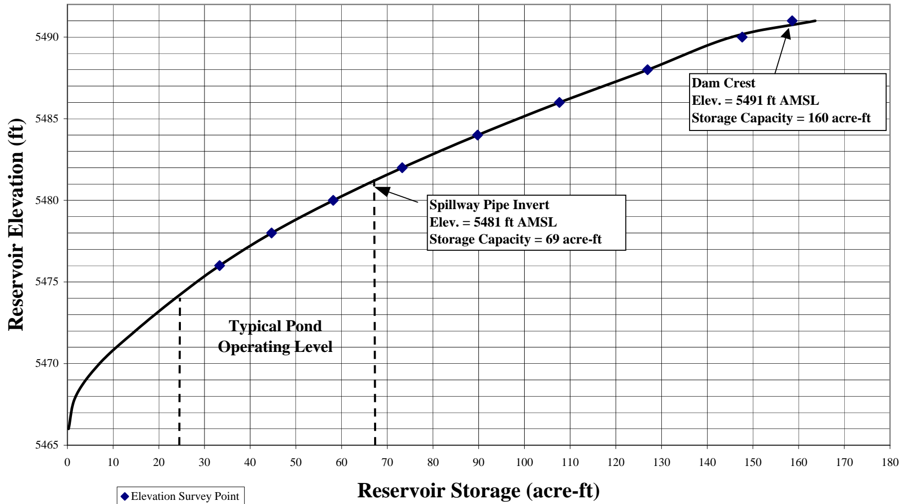
FIGURE 2-2. MIKE HORSE TAILINGS IMPOUNDMENT STAGE-STORAGE CURVE
