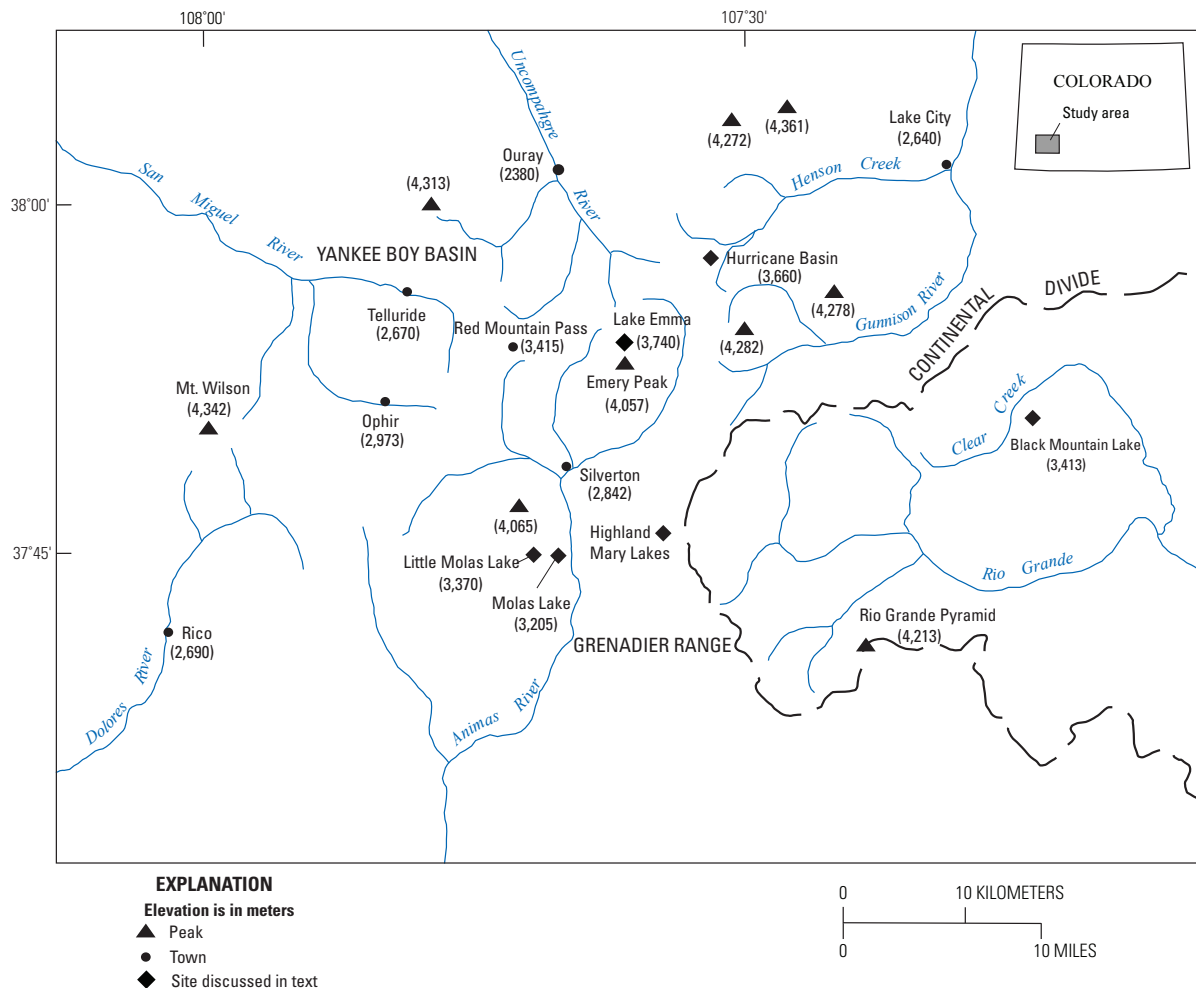
Figure 1. Northern San Juan Mountains and selected sites discussed in this study. Elevations in meters.
