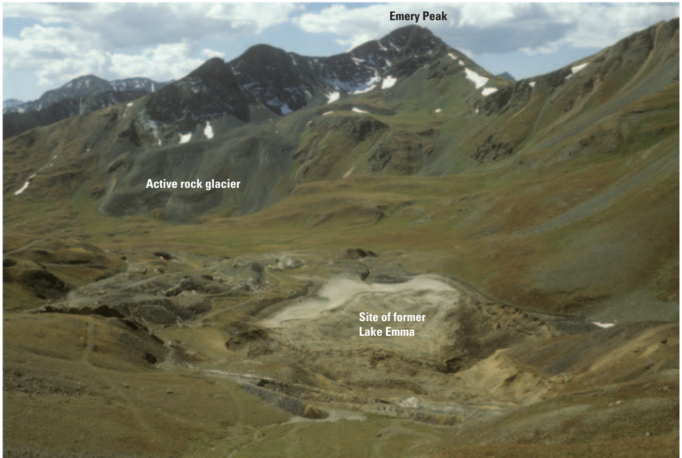
Figure 4. Site of former Lake Emma in 1979 after accidental drainage of the lake. Note an active rock glacier flowing from the cirque on Emery Peak about 1 km south of the former Lake Emma and the lack of coniferous trees, even krummholz forms.
