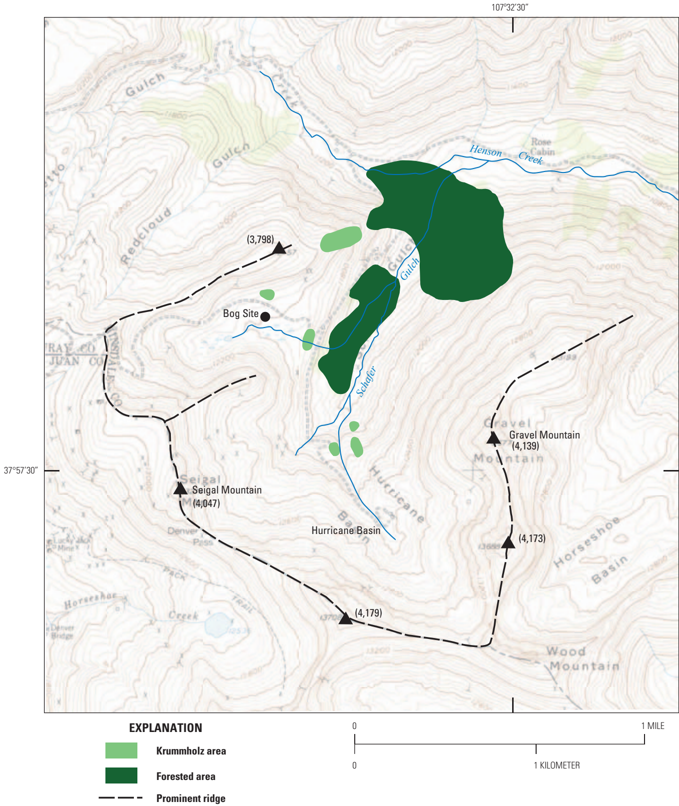
Figure 16. Hurricane Basin area. Elevations are in meters.
