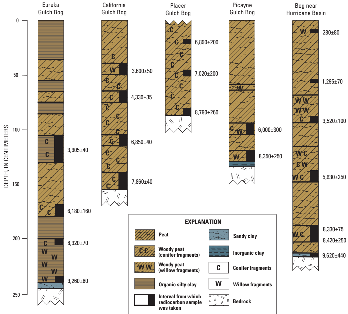
Figure 8. Stratigraphic sections and radiocarbon ages (yr B.P.) from bogs in the northern San Juan Mountains. The section for the bog near Hurricane Basin represents a composite stratigraphy from Andrews and others (1975) and Carrara and others (1991).
