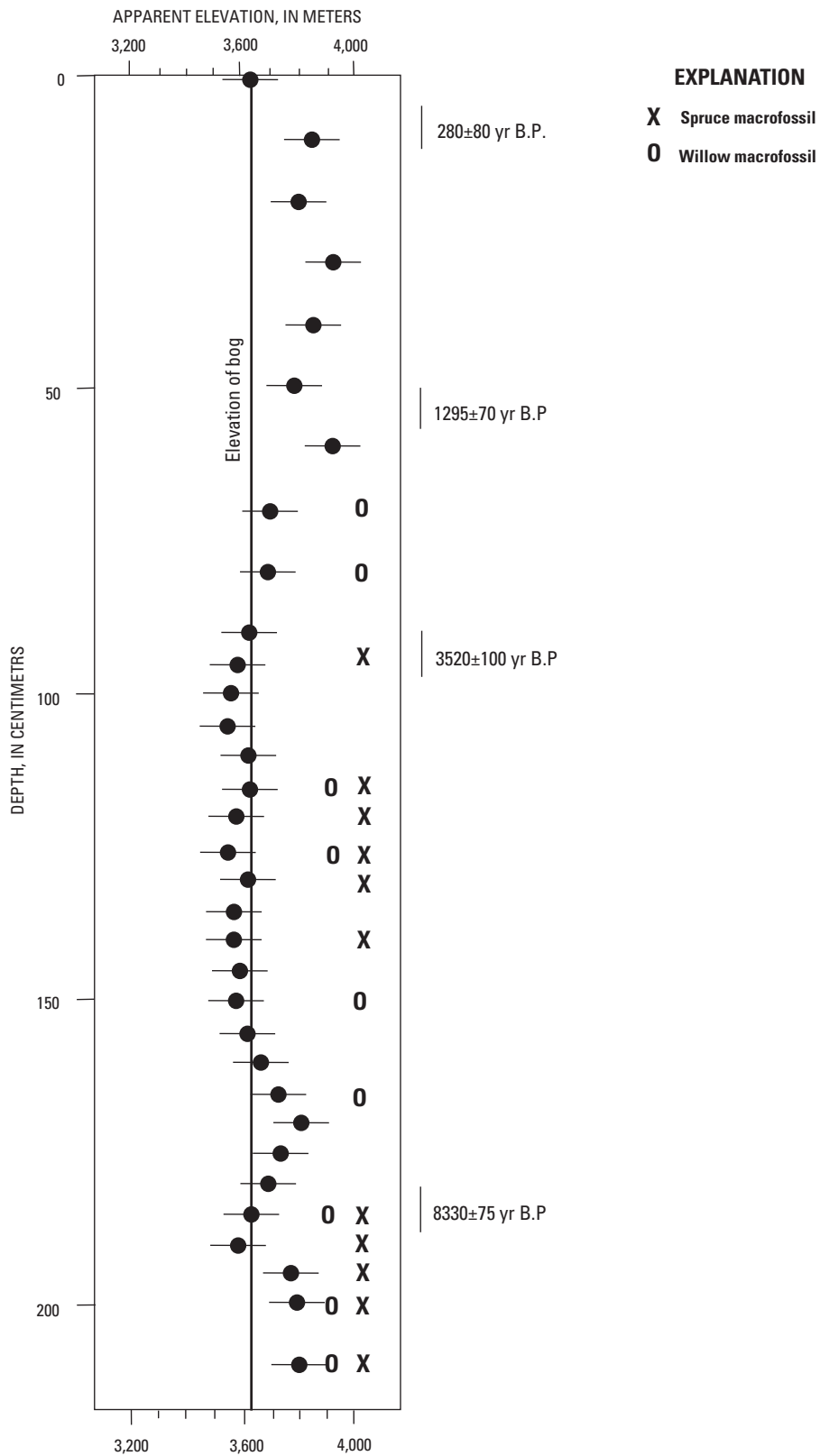
Figure 18. Changing apparent elevation of the Hurricane Basin core based on spruce/pine ratios; radiocarbon ages (yr. B.P.) and location of macrofossils also shown (after Andrews and others, 1975).
