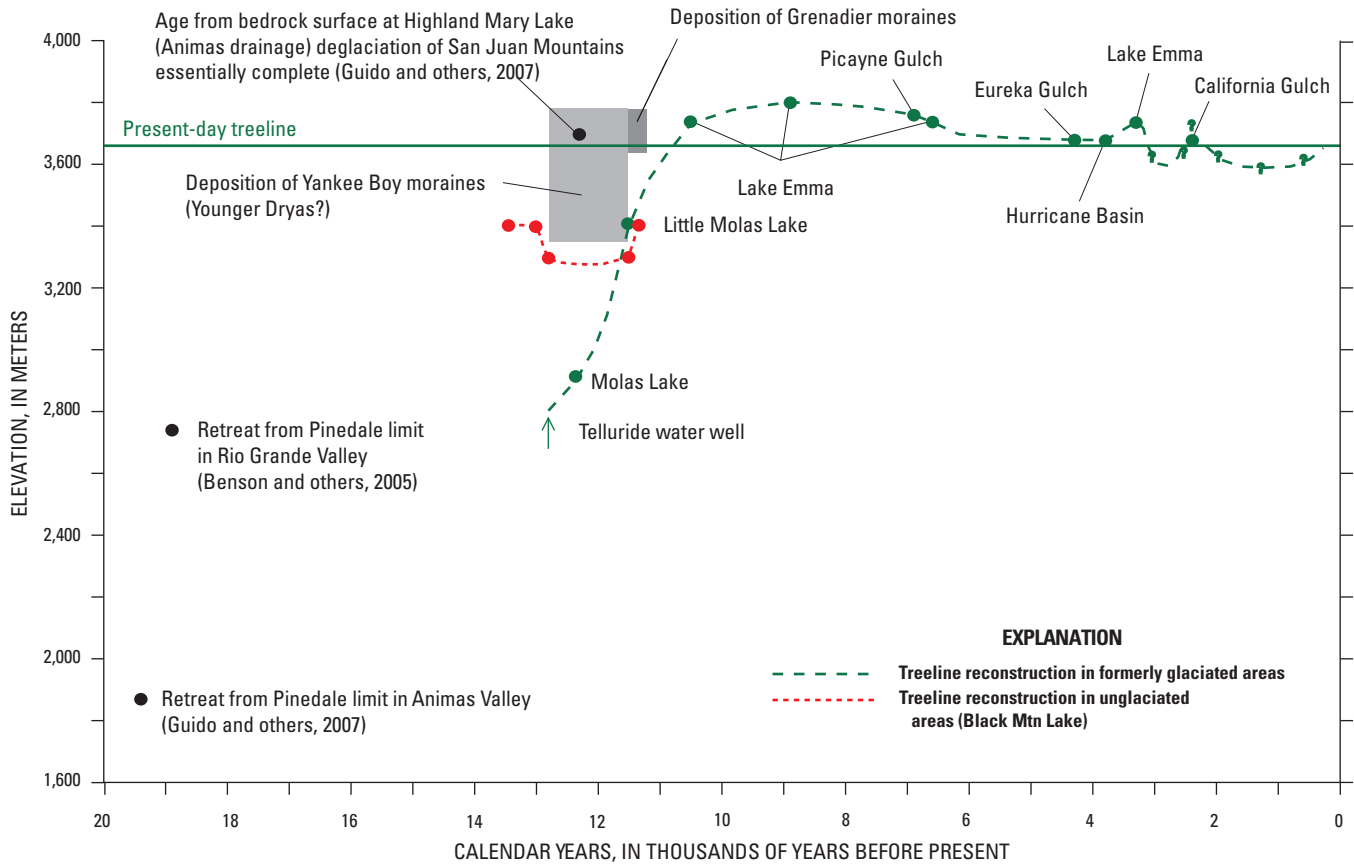
Figure 25. Timeline of events in the San Juan Mountains showing initial timing of Pinedale glacial retreat, deglaciation of the range, deposition of the Yankee Boy and Grenadier moraines, and treeline fluctuations from the late Pleistocene through the Holocene.
