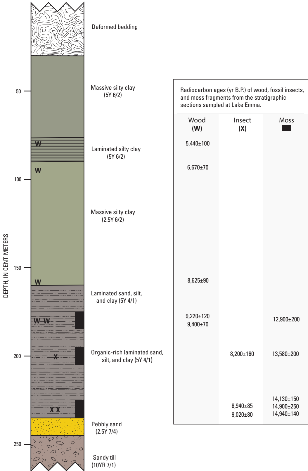
Figure 7. Composite stratigraphic section at the Lake Emma site (after Carrara and others, 1984; and Elias and others, 1991) showing radiocarbon ages (yr. B.P.) of wood, insect fossils, and detrital moss.
