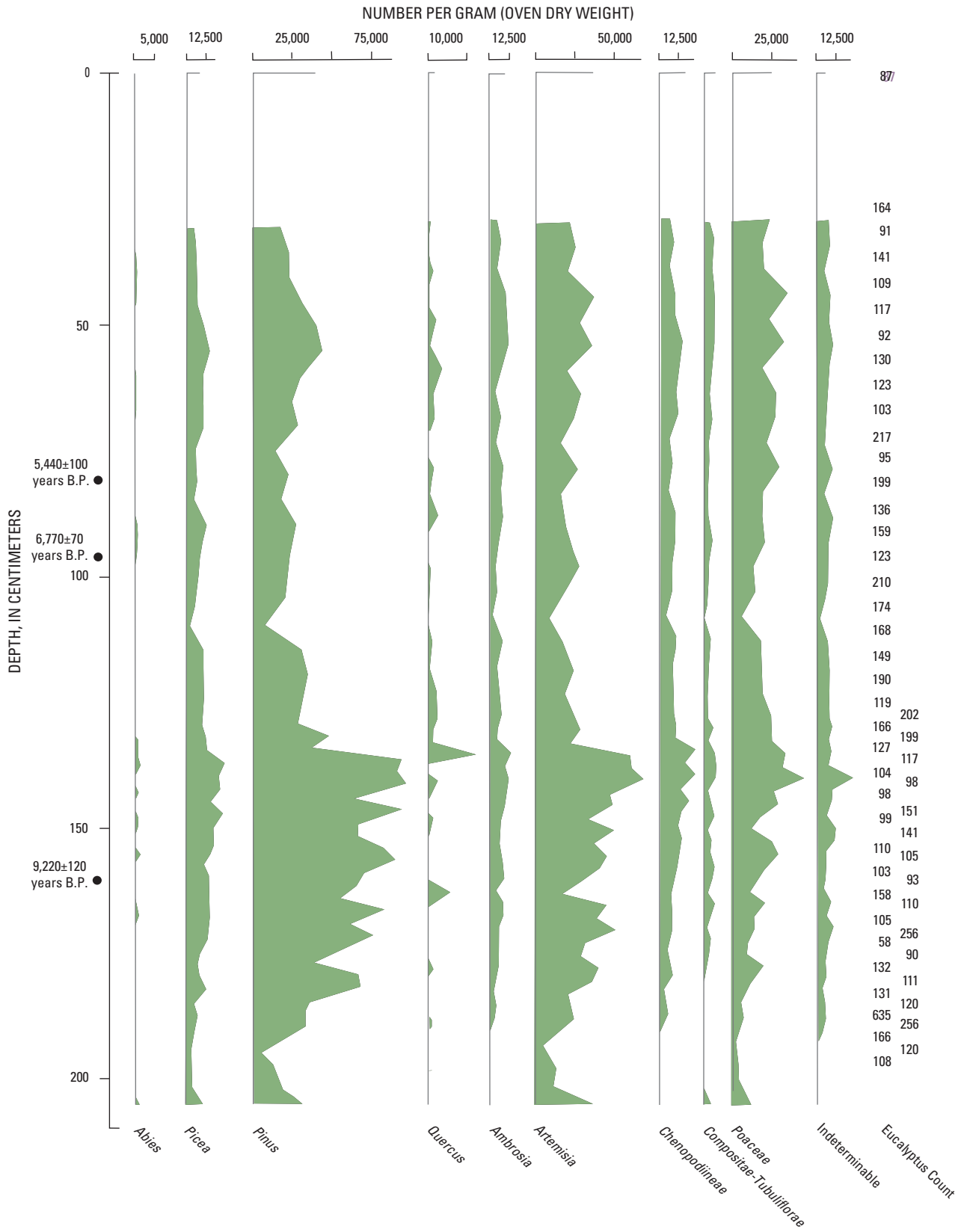
Figure 23. Pollen concentration summary diagram from Lake Emma (after Carrara and others, 1984). B.P., before present.
