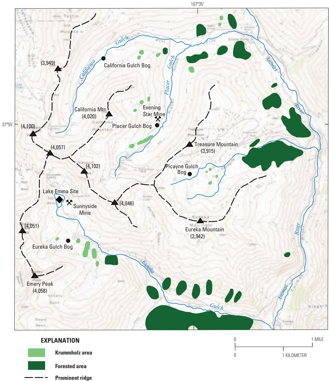
Figure 2. Study sites near headwater region of Animas River. Elevations in meters.
