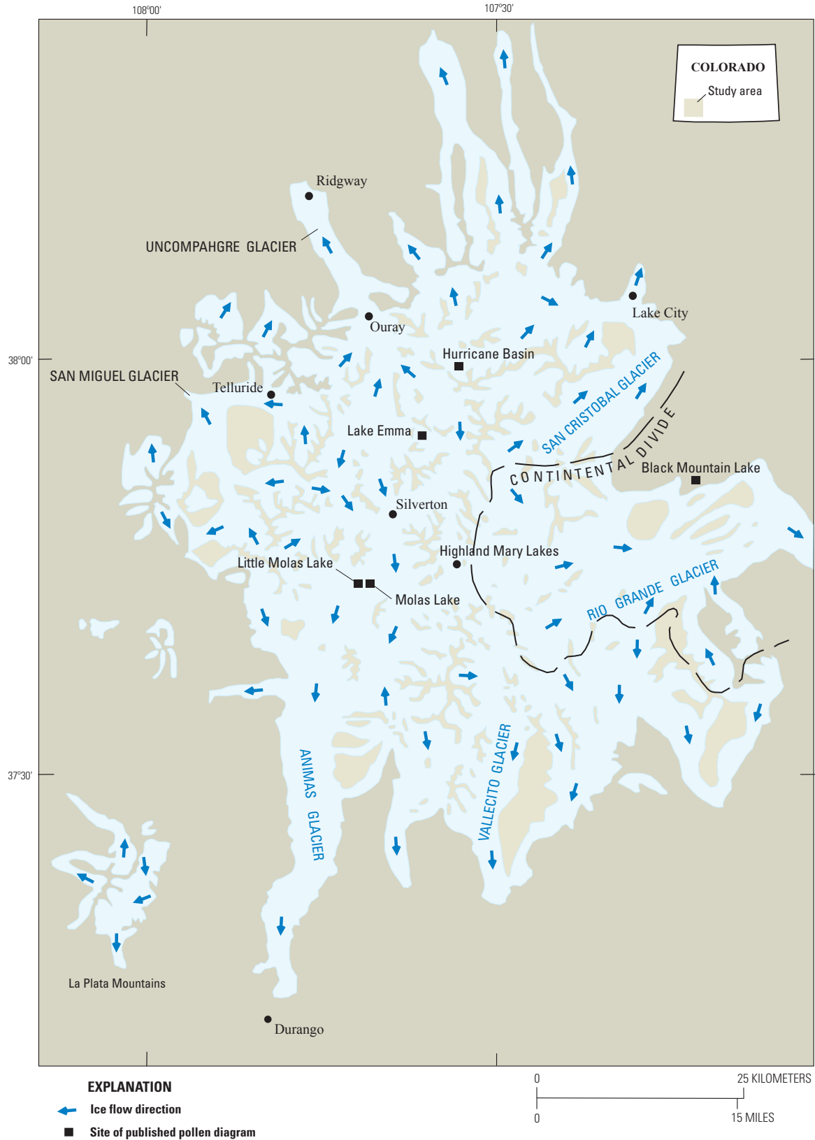
Figure 5. Limits of Wisconsin (Pinedale) glacialiation in western San Juan Mountains (after Atwood and Mather, 1932), including the Animas-Uncompahgre transection glacier. This glacier stretched from near the present-day town of Ridgway south for about 100 km to near the present-day town of Durango.
