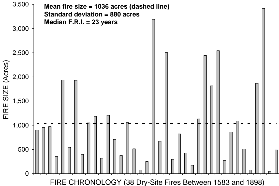
Figure 1 – Spatial variability in fire extent for dry-forest sites in Tucannon River watershed, northern Blue Mountains of southeastern Washington (figure based on data from Heyerdahl 1997). Forty individual fire years were determined for Tucannon River watershed, and 38 of them included fires on what are predominantly dry-forest sites. The smallest fire extent on dry-forest sites was 47 acres and the largest was 3,417 acres. Average fire extent for dry-site fires was 1,036 acres (dashed line shows an average). Note that the last recorded fire for this watershed occurred in 1898 (Heyerdahl 1997).
