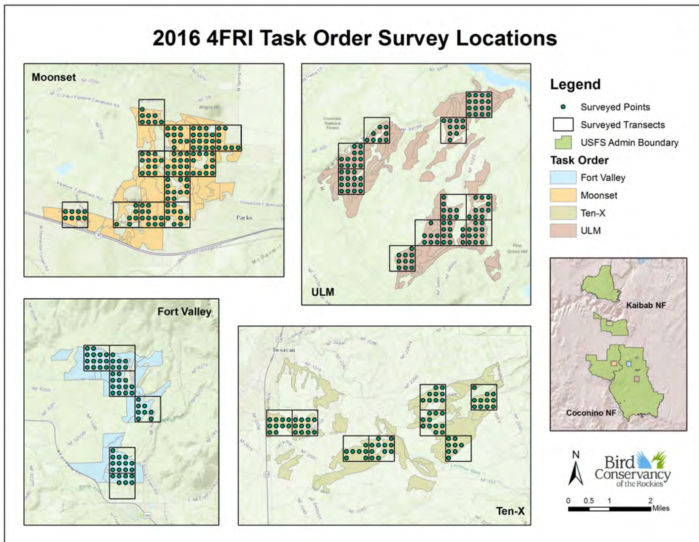
Figure 1. Spatial extent of sampling for the Four Forest Restoration Initiative, 2016.
