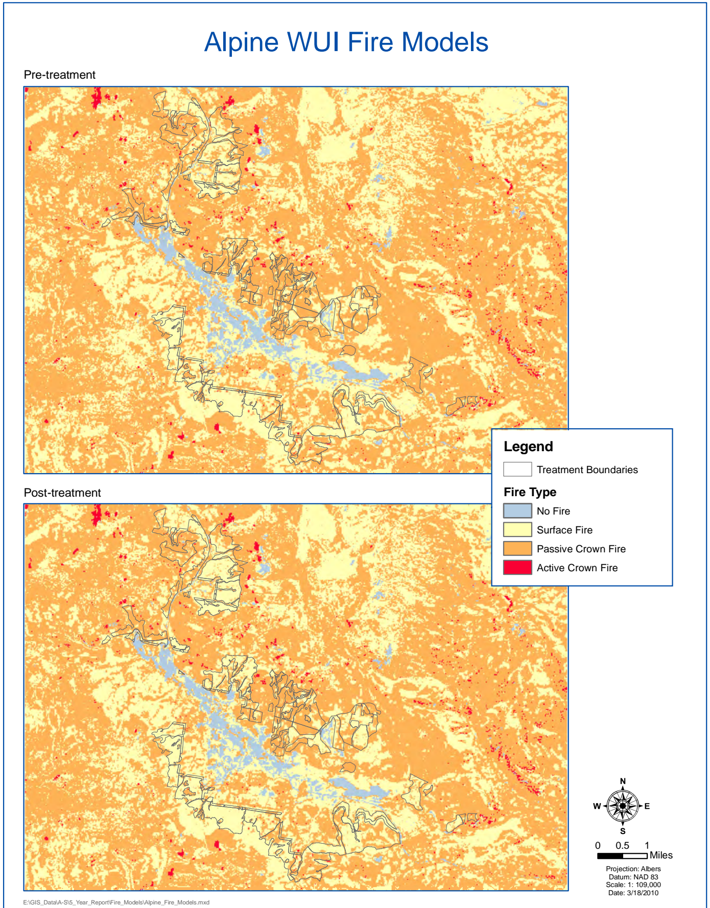
Figure 5. Projected fire behavior characteristics for pre- and post-treatment conditions in the Alpine WUI project area, treated as part of the White Mountain Stewardship Project
