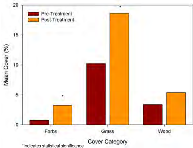
Figure 4. Mean forb, grass, and wood cover (%) changes in pre- and post-treatment conditions for permanent point-intercept transects sampled at the Greer project area in the White Mountain Stewardship Project
