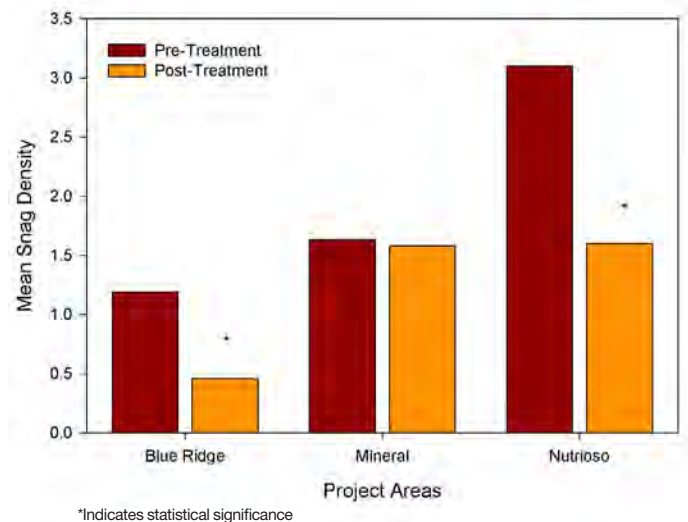
Figure 2. Mean snag density (snags per acre) changes in pre- and post-treatment conditions for permanent plots sampled at three project areas in the White Mountain Stewardship Project
